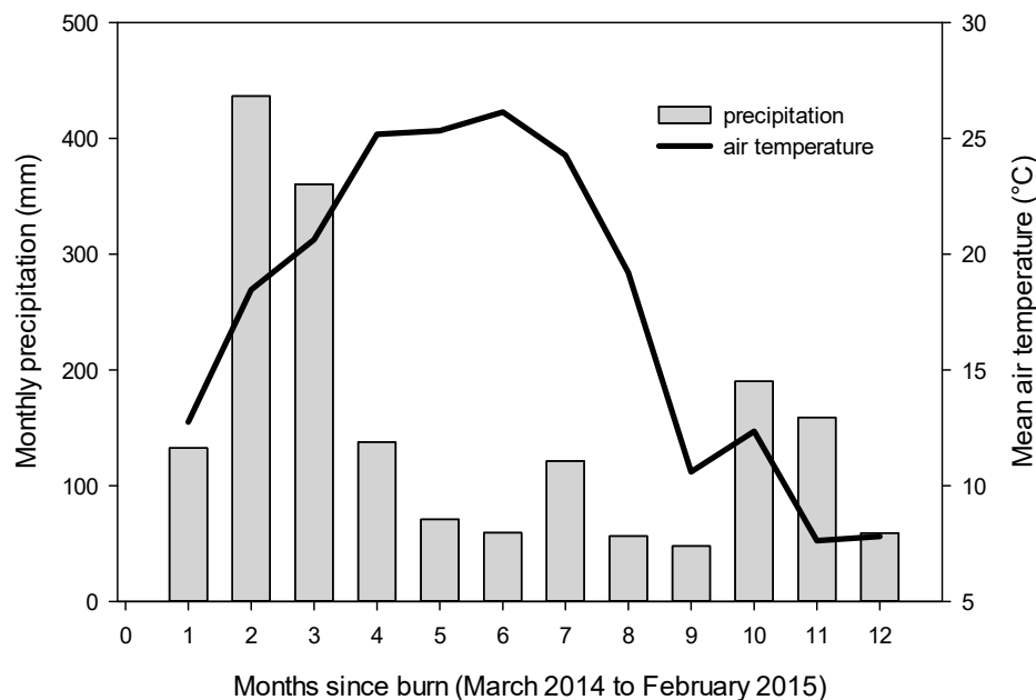
Figure 2. Monthly precipitation and monthly mean air temperature at the Harrison Experimental Forest near Saucier, Mississippi, for the 12 months following prescribed burning on 28 February 2014.
