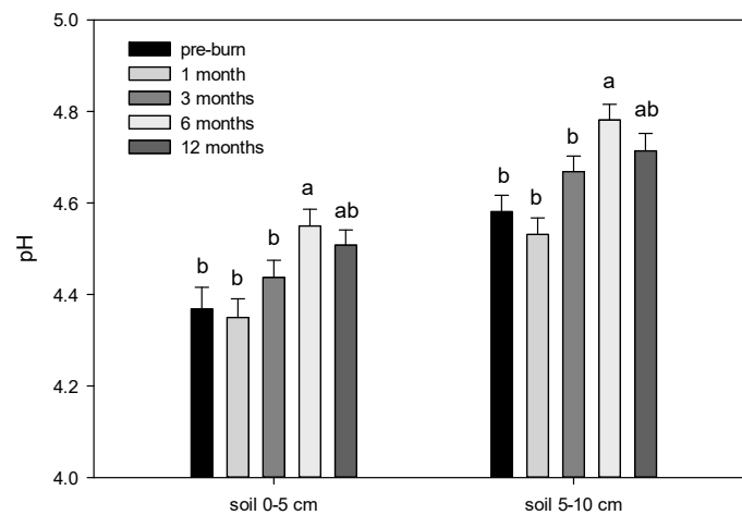
Figure 6. Soil pH from samples collected pre-burn, followed by collections at 1, 3, 6, and 12 months after the fire. Within each group, means with the same letter do not differ at p < 0.05 and error bars represent the standard error of the mean.
