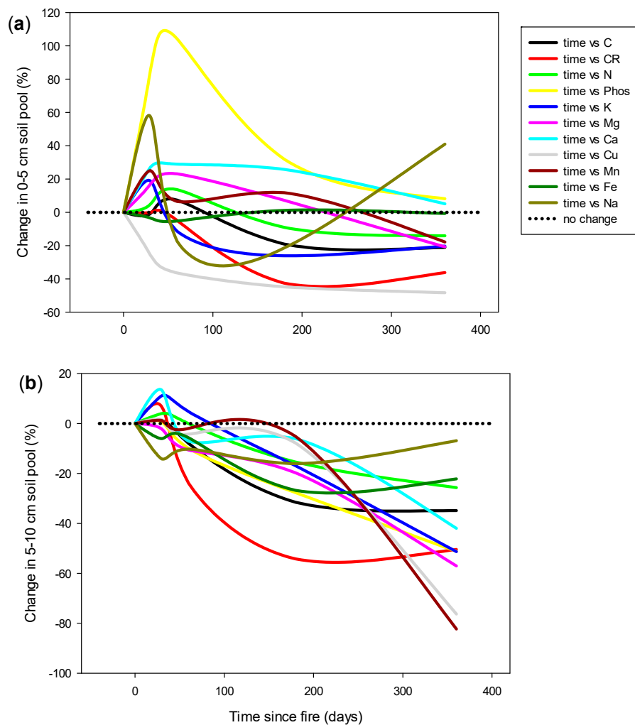
Figure 7. Percent change in soil C, CR, N, macro and micronutrients from samples collected pre-burn and 1, 3, 6, and 12 months after the fire at depths of 0–5 (a) and 5–10 cm (b).
