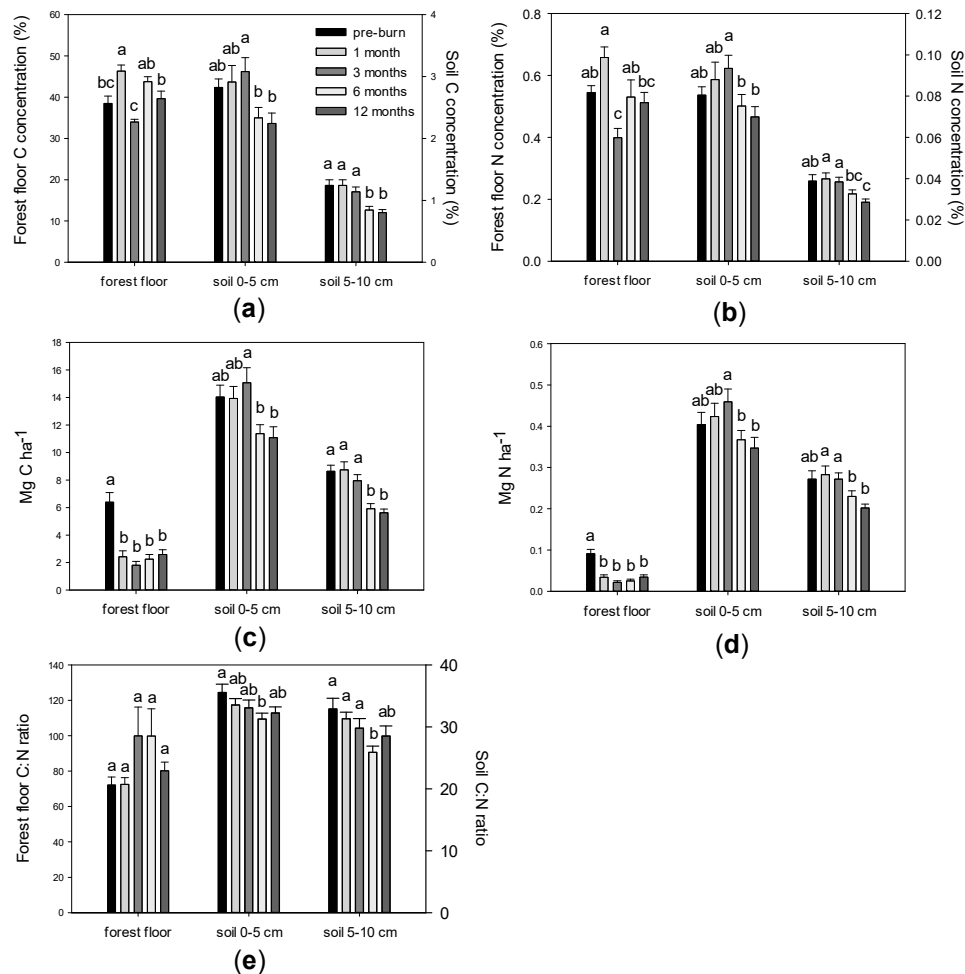
Figure 3. C and N concentrations (a,b), C and N pools (c,d) and C:N ratios (e) of forest floor and soil collected pre-burn and 1, 3, 6, and 12 months after the fire. Within each group, means with the same letter do not differ at p < 0.05 and error bars represent the standard error of the mean. Note that a , b and e have separate x axes scaled for forest floor and soil, respectively.
