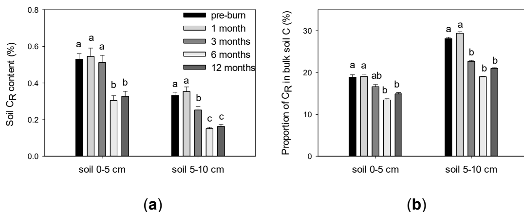
Figure 4. Oxidation resistant soil C ( C_R ) content of soils from depths of 0–5 and 5–10 cm (a) and the proportion of C_R in bulk soil C (b). Within each group, means with the same letter do not differ at p < 0.05 and error bars represent the standard error of the mean.
