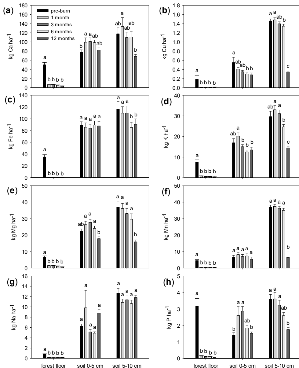
Figure 5. Soil nutrient content of Ca, Cu, Fe, K, Mg, Mn, Na, and P (a–h) from samples collected pre-burn, followed by collections 1, 3, 6, and 12 months after the fire. Within each group, means with the same letter do not differ at p < 0.05 and error bars represent the standard error of the mean.
