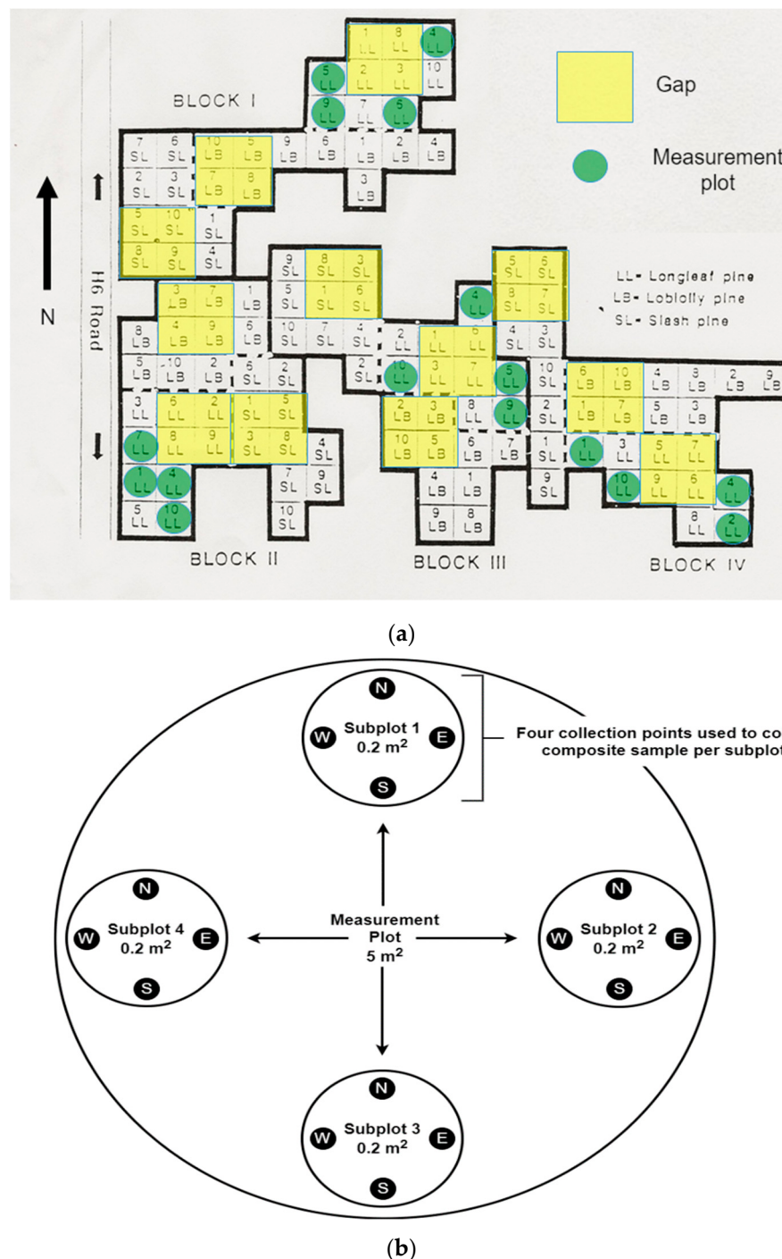
Figure 1. Map of study site at the Harrison Experimental Forest near Saucier, Mississippi, where green circles denote the location of 16 measurement plots and yellow squares identify 12 gaps that were harvested (a). Within each 5 m 2 measurement plot, four 0.2 m 2 subplots were located 1 m from center (b).
