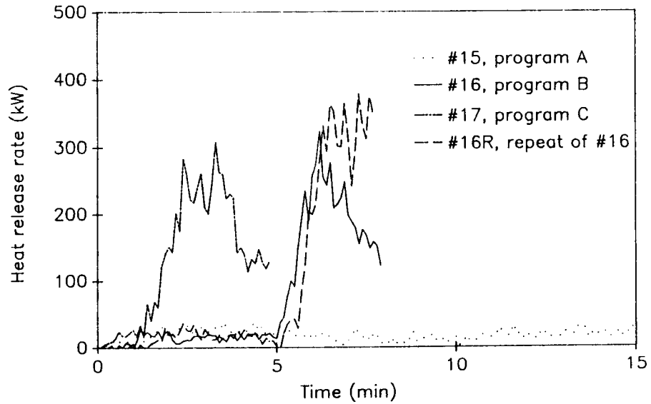
Figure 5. Rate of heat release in wall tests.
