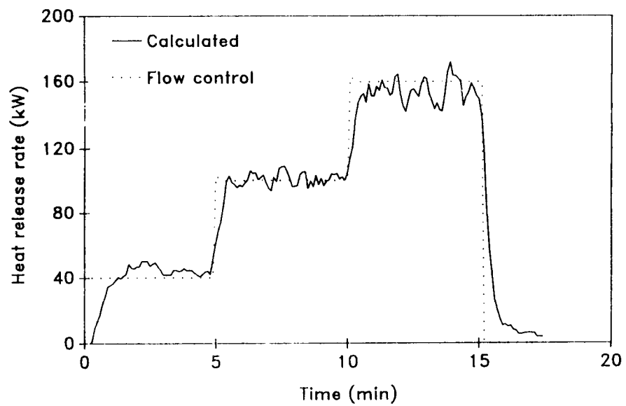
Figure 4. Calibration test no. 23, program D.
