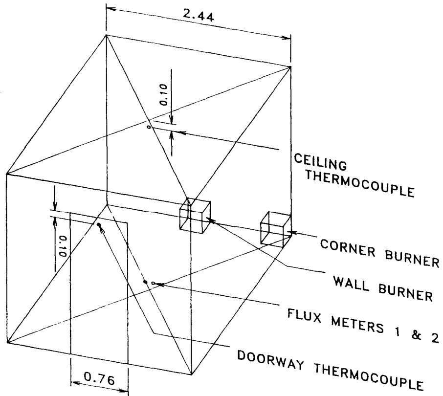
Figure 1. Three-dimensional view of burn room.
