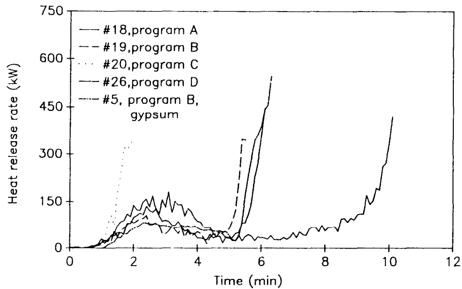
Figure 6. Rate of heat release in corner tests.
