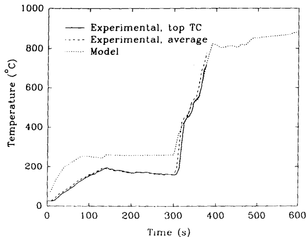
FIG. 10—Benchmark model data and experimental data on upper layer temperature
