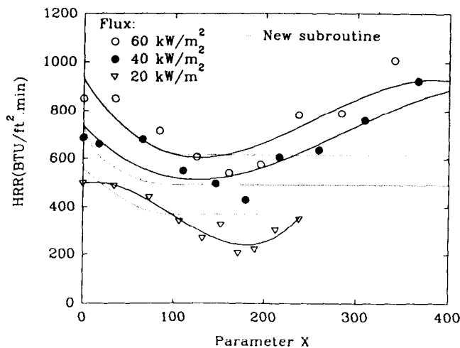
FIG. 6—Weyco heat release rate data for particleboard.
