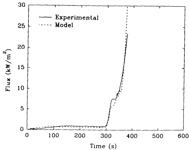
FIG. 11—Benchmark model data and experimental data on heat flux to the floor.
