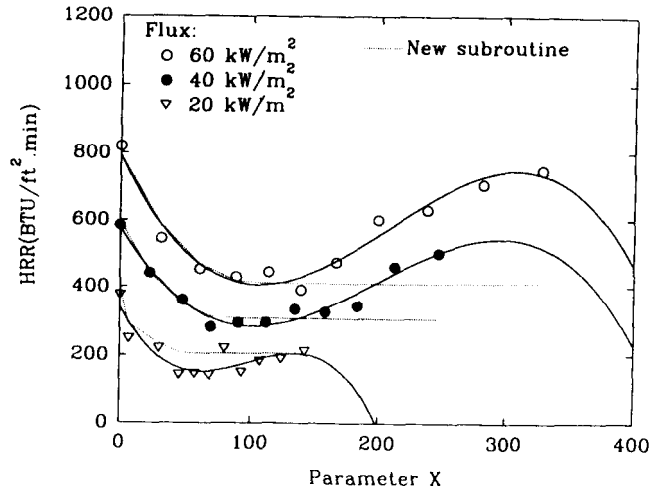
FIG. 4—Weyco heat release rate data for redwood.
