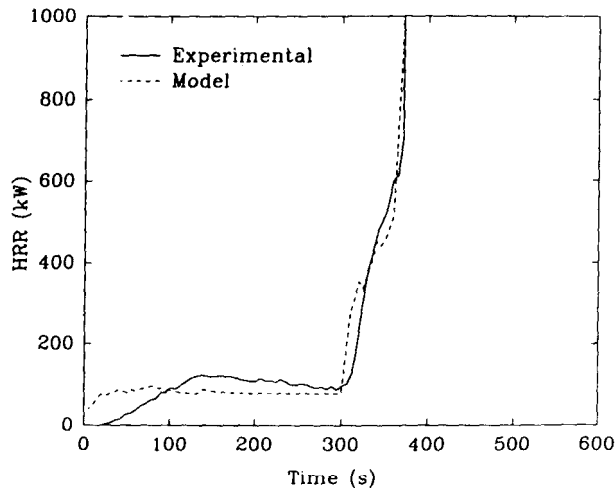
FIG. 9—Benchmark model data and experimental data on heat release rate
