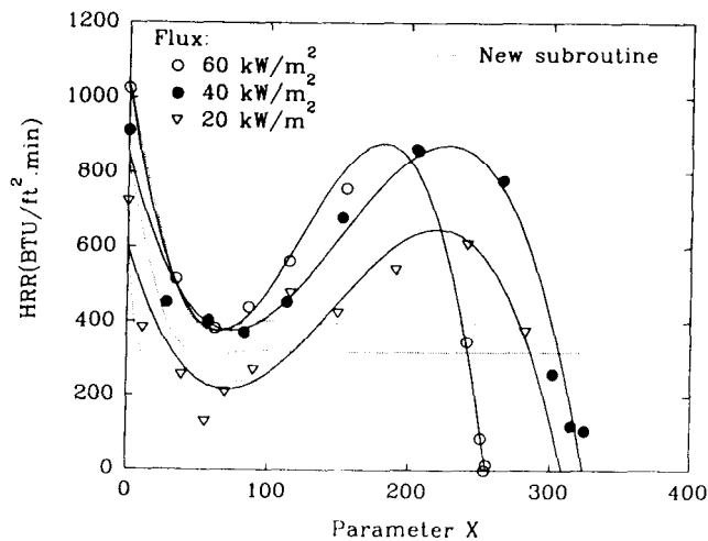
FIG. 3—Weyco heat release rate data for DF plywood.
