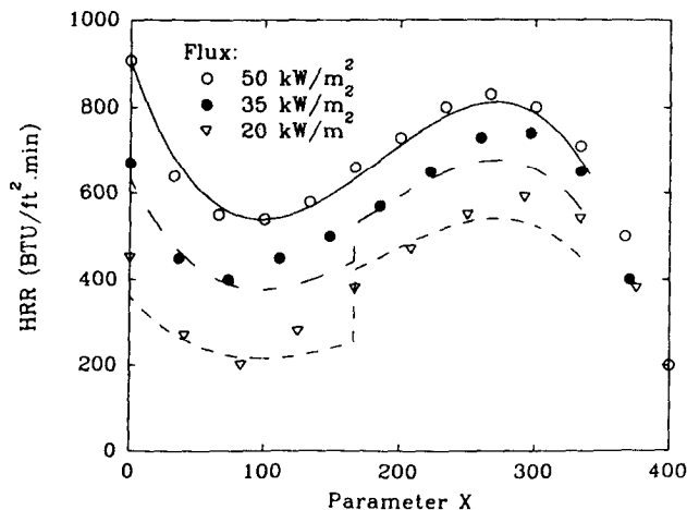
FIG. 2—Heat release rate data for DF plywood from Smith's subroutine.
