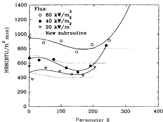
FIG. 7—Weyco heat release rate data for OSB.
