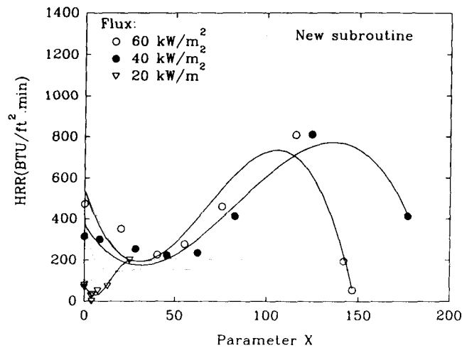
FIG. 8—Weyco heat release rate data for FRT plywood
