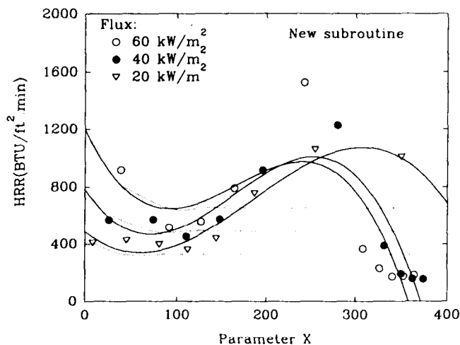
FIG. 5—Weyco heat release rate data for SP plywood.
