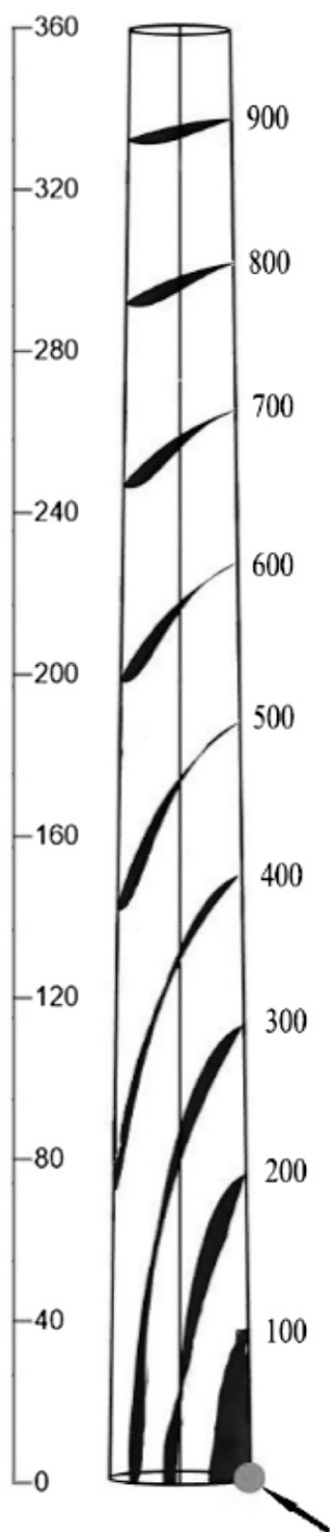
Figure 7. Wave front progression maps of the tree model (unit: \mu s; the dot in the lower right corner indicates the wave initiation point).
