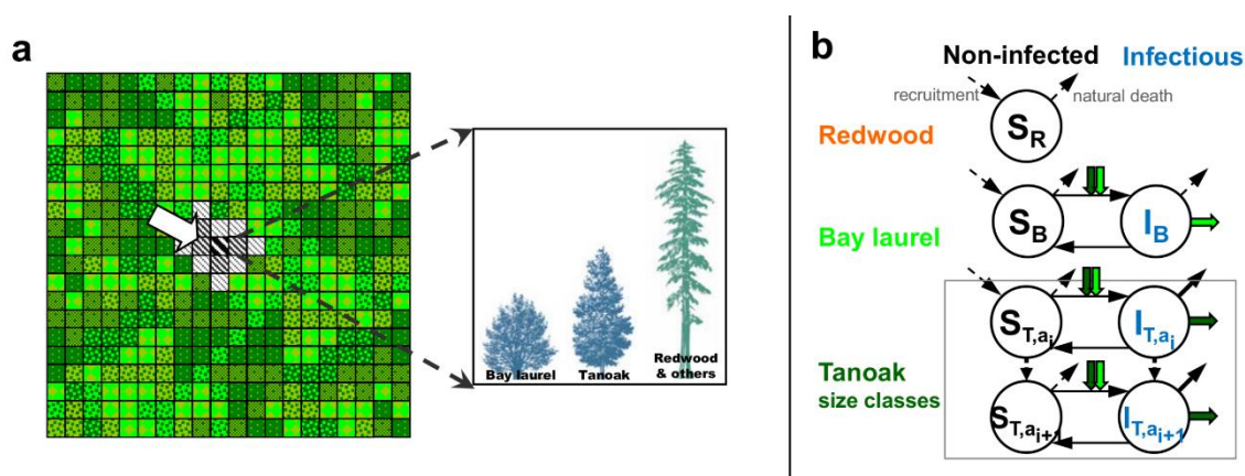
Figure 1. Model of community composition and pathogen invasion. (a) Illustrative spatial dynamics of an epidemic spreading from the centre of a model stand that represents a single-landowner forest plot of 20 ha. The stand is a spatial lattice of 400 cells, each with approximately 2.5 m × 2.5 m and with specific and changing tree composition and canopy structure (different shadings). The figure shows increasing pathogen level in the cells invaded from the introduction point (stripping), but not the associated changes in densities of host species. Here, species have heterogeneous densities across the stand before and after pathogen invasion to illustrate the model’s generic scope; the results shown later refer to stands that are heterogeneous after but homogeneous before disease in order to simplify interpretation of the impacts of disease management actions. (b) Compartmental model of the unmanaged dynamics of the stand (circles and transition arrows) defined by epidemic and species-density states in each cell i [45]. Epidemic state is represented by susceptible (non-infected) (S) and infectious (I) compartments, and the species populations by redwood (R) and bay laurel (B) average-size and tanoak (T) canopy-size-class ( a i ) compartments. Infected cells contribute according to relative distance (thick horizontal arrows, species-specific tone) to the force of infection (thick vertical arrows) on each non-infected host in cell i . Species have mortality and density-dependent birth (thin-arrows). See Appendix A for more detail on the model dynamics.
