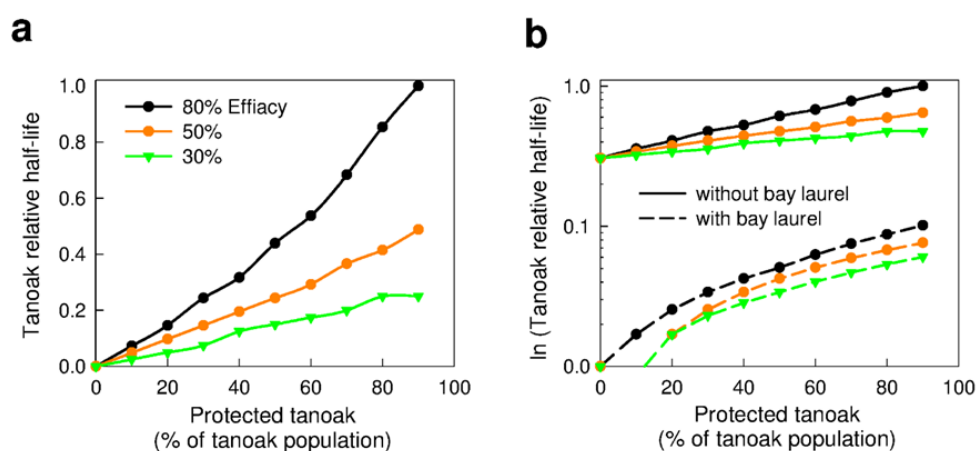
Figure 7. Potential of chemical protection to increase the durability of a tanoak population invaded by P. ramorum , in a forest with 60% tanoak and (a) without bay laurel (40% redwood) (time relative to this forest type only), and (b) without bay laurel or with 20% bay laurel (20% redwood) (time relative to both forest types, natural-log scale), over the range of coverage strategies for three chemical protectants (efficacy 30%, 50%, and 80%; see text for details) applied biennially across the stand one year after invasion of P. ramorum . Here, relative half-life is the period after which 20% (not 50%) of the initial tanoak has been lost since invasion.
