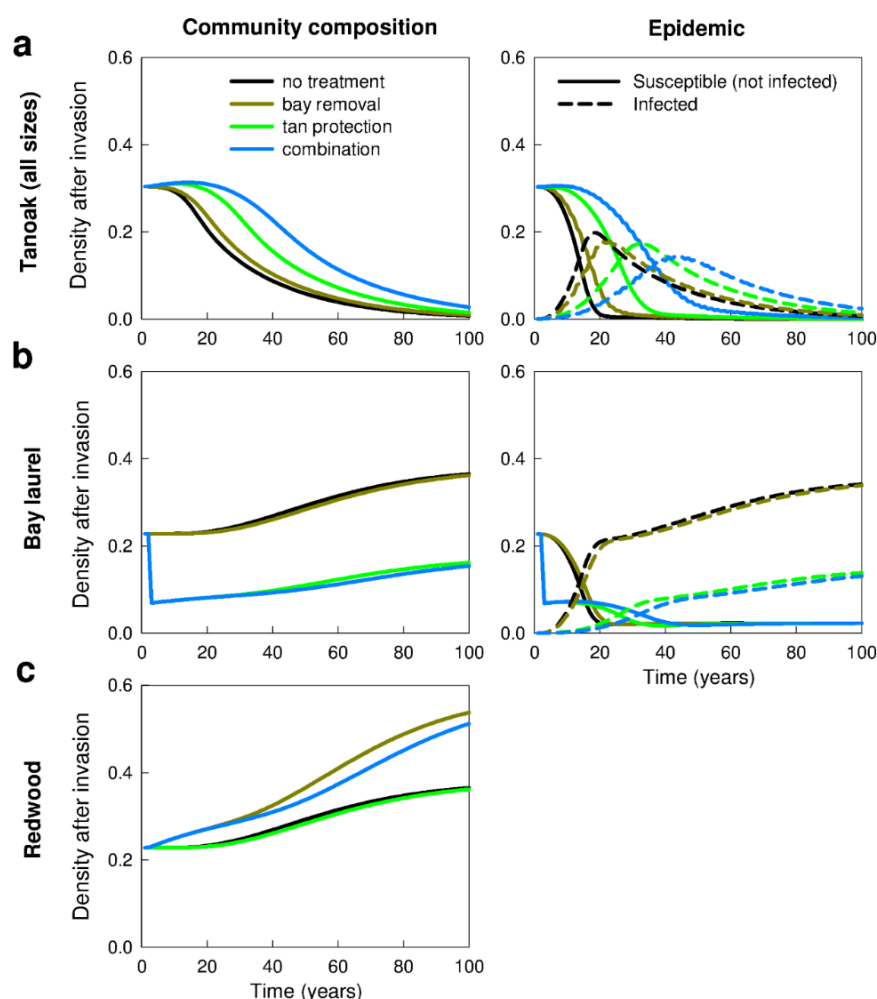
Figure 5. Impact of treatments on the pace of composition change (species density—left) and epidemic progress (densities of susceptible and infectious tanoak and bay laurel—right) in a mixed-forest stand from the time of invasion by P. ramorum . All quantities are spatial totals of the spatially heterogeneous epidemic in the stand (see Methods). Treatments applied one year after invasion: no treatment, removal of bay laurel (single round with herbicide application), chemical protection of tanoak (“tan protection”), and combination strategy. Impacts on: (a) tanoak (all size classes), (b) bay laurel, and (c) redwood (this category represents all epidemiologically non-significant species in our study area, of which redwood ( S. sempervirens ) is the most common). In mixed-forest stands, the impact of tanoak protection alone is weak because of high abundance of bay laurel (prevalence 30%, density 23%).
