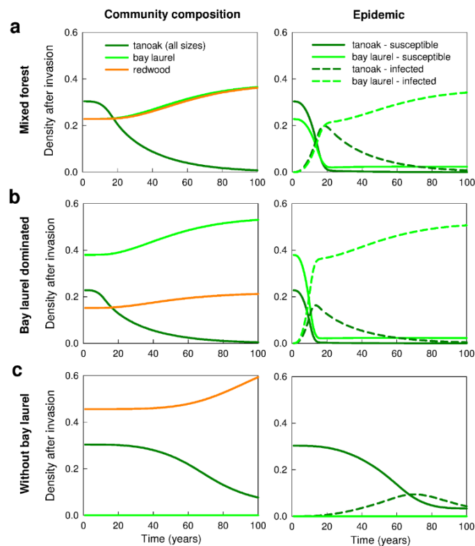
Figure 4. Temporal change in forest composition of an unmanaged stand invaded by P. ramorum : change by species spatial-averaged density (left) and epidemic progress in the host populations (right). Forest type: (a) mixed, (b) dominated by bay laurel, (c) without bay laurel. The outbreak starts at time 0. The initial and final tanoak densities in c correspond to those in Figure 3a. Tanoak density aggregates all size classes.
