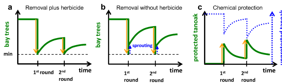
Figure 2. Schematic illustration of the application of treatments to P. ramorum hosts over time: removal of bay laurel and chemical protection of tanoak. Vertical axes represent amounts of bay laurel and protected and unprotected tanoak in the stand before and after treatments: (a,b) After removal, there is natural recovery in the bay laurel population. (c) After chemical protection, tanoak trees lose protection gradually. Herbicide: (a) Illustration of herbicide application to prevent re-sprouting (Scheme 2 corresponds to the period prior to the second round). (b) If herbicide is not applied after cutting, bay laurel trees can re-sprout; this rebound is represented by an instantaneous increase in the number of non-infected bay laurel stems in each cell (Scheme 3 corresponds to the full time line). Constraints on treatment coverage: (a,b) There is a cap on the amount of bay laurel that can be removed in each cell and treatment round, corresponding to a maximum effort. Moreover, for conservation purposes, we do not allow the bay laurel population to drop below a minimum density ('min'); hence, in some cells fewer removal resources are used than their available maximum. (c) There is a maximum density of tanoak that can receive chemical application in each cell and treatment round.
