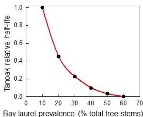
Figure 8. How bay laurel limits the effectiveness of chemical protection of tanoak against P. ramorum infection in mixed forests with differing initial prevalence (% of stems) of bay laurel and redwood and 40% prevalence of tanoak. Chemical treatment is as in Figure 7, but with default coverage (80%) and efficacy (70%). The relative half-life is in the sense of Figure 7.
