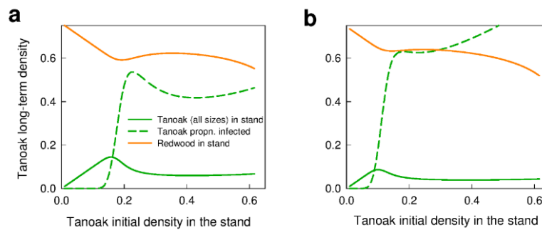
Figure 3. Epidemic thresholds in tanoak density (proportion of stand area occupied by species) in unmanaged forest stands: tanoak proportion infected and density in the stand 100 years after P. ramorum invasion across scenarios where tanoak density prior to invasion ranges from 0 and 0.6 and, (a) without bay laurel, or (b) with 1.5% prevalence (proportion of total stems) of bay laurel. For very low bay laurel density, a threshold tanoak density exists below which the pathogen does not cause epidemics; for higher bay laurel density this threshold ceases to exist. See Figure 4c for examples of epidemic trajectories on tanoak and bay laurel up to the current point after pathogen invasion. An epidemic threshold is a minimum number or density of susceptible hosts necessary for an epidemic to occur; reducing the density of susceptible hosts below this minimum is the underlying principle of vaccination [52]. The tanoak density comprises all tanoak size classes.
