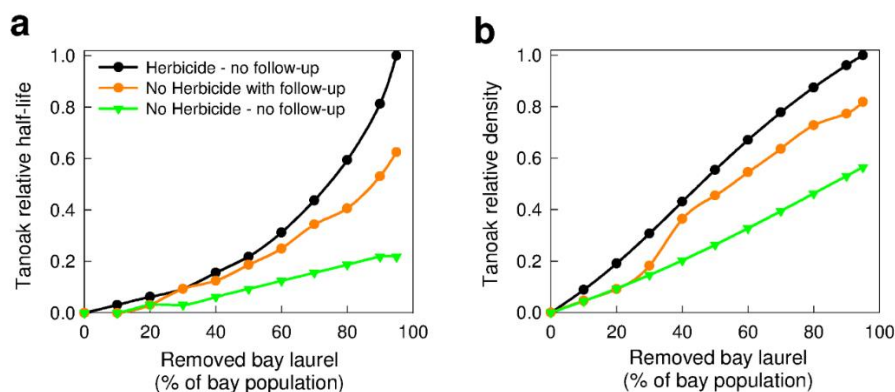
Figure 6. Comparison of how much herbicide application or follow-up of treatment enhance the ability of bay laurel removal to increase the durability of tanoak populations in mixed-forest stands invaded by P. ramorum . (a) Tanoak relative half-life; and (b) tanoak relative density (space-averaged) 20 years after invasion, in three strategies of implementation of removal (one round with herbicide application, and one round or two rounds (in 5 years) without herbicide application) initiated one year after invasion across the range of population coverage levels. We obtained similar results (not shown) in a mixed forest with more redwood than tanoak (40% and 30%, rather than 30% and 40%). Relative measures of durability are defined in Methods. Results rely on model accuracy up to time considered, e.g., half-life, not up to the considerably longer 100 year horizon in Figures 4 and 5.
