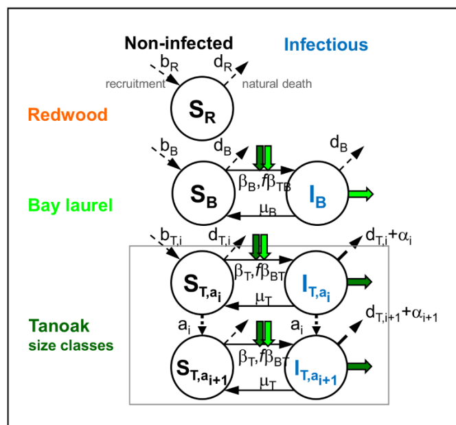
Figure A1. Compartmental model of the unmanaged dynamics of P. ramorum in a forest stand. The epidemic is represented by susceptible (non-infected) (S) and infectious (I), and the species populations by redwood (R) and bay laurel (B) average-size and tanoak (T) canopy-size-class compartments in each cell i within the stand metapopulation. Transition dynamics: infection and recovery (full dark arrows), recruitment (broken, inward arrows), death (broken, outward arrows, thicker for disease-augmented mortality), ageing of tanoak (dotted arrows), contribution to infection rate (thick arrows). See Table A1. Similar to Figure 1a but with parameter notation.
