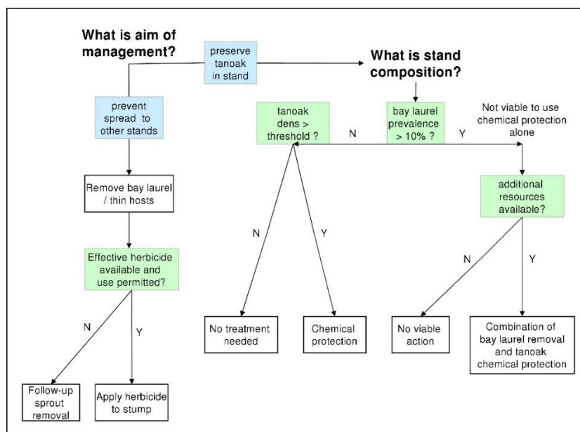
Figure 10. Diagram of options of disease management for tanoak conservation in a forest stand. Species prevalence is the proportion of the total stems; species density is the proportion of the stand area occupied by the species.
