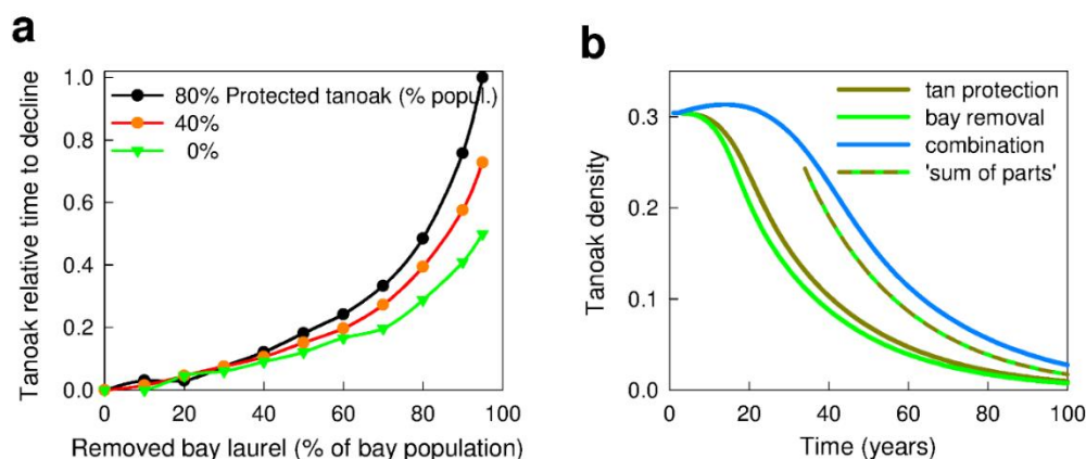
Figure 9. Benefits of combination strategies. (a) Potential of combination strategies to increase the durability of the tanoak population in a mixed-forest stand, for a variety of strategies differing in the levels of coverage of bay laurel removal (0–95%) and coverage of tanoak chemical protection (0%, 40%, 80%). Treatments: removal of bay laurel (single round with herbicide) and chemical protection (75% efficacy, as in Figure 7) initiated one year after pathogen invasion. Note that the efficacy of chemical protection is lower than that documented for phosphonate treatments against P. ramorum [41]. (b) Contrast of the impacts of combined- and single-treatment management strategies on the density of tanoak since the start of the epidemic. There is a synergistic effect in the combination strategy as it yields a tanoak abundance that exceeds the sum of the abundances in the separate strategies ('sum of parts'). Treatments are as in A and Figure 6, but coverage of bay removal is 70%.
