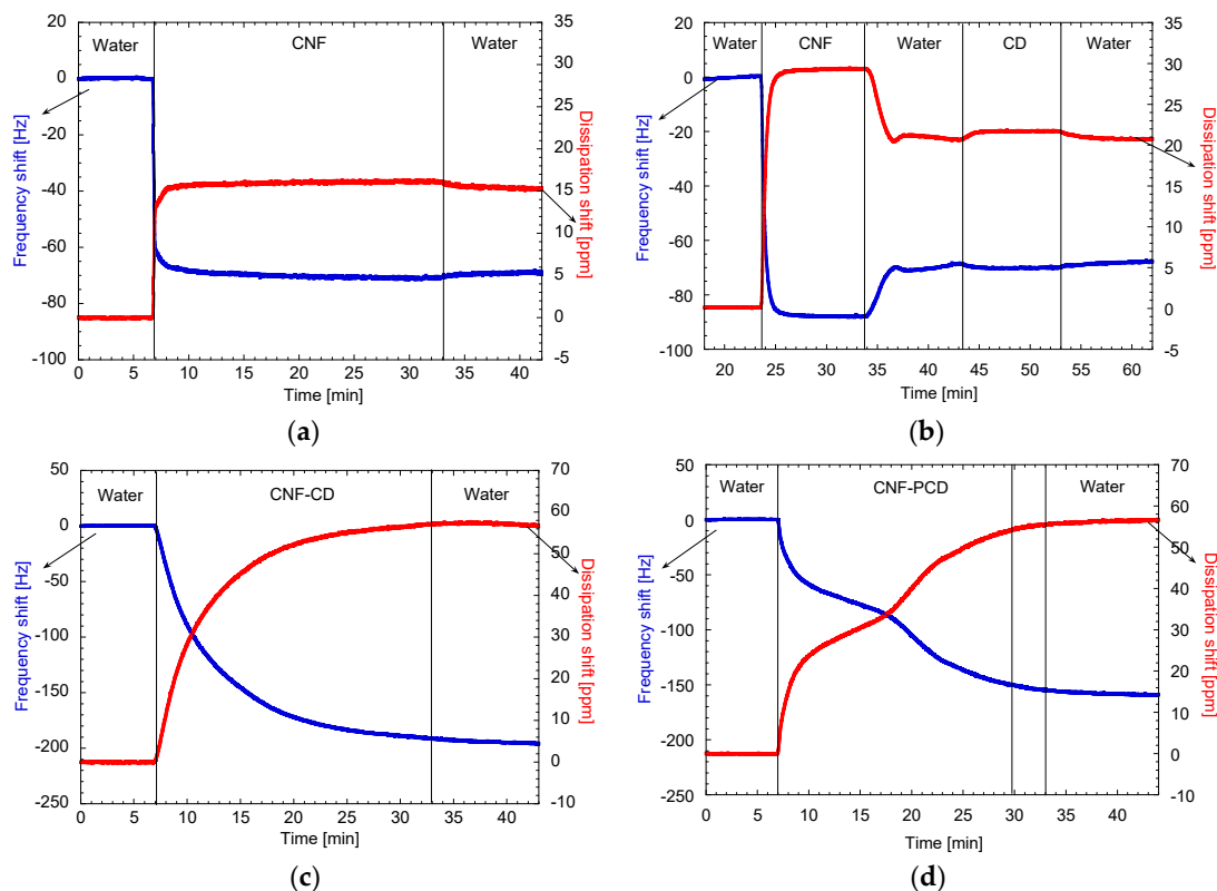
Figure 9. QCM-D sensograms of the in situ surface generation from (a) CNF, (b) CNF and flushed CD (CNF+CD), (c) CNF-CD, and (d) CNF-PCD. CNF, cellulose nanofibrils; CD, cyclodextrin; CNF-CD, cellulose nanofibrils grafted with cyclodextrin; CNF-PCD, cellulose nanofibrils grafted with poly-cyclodextrin.
