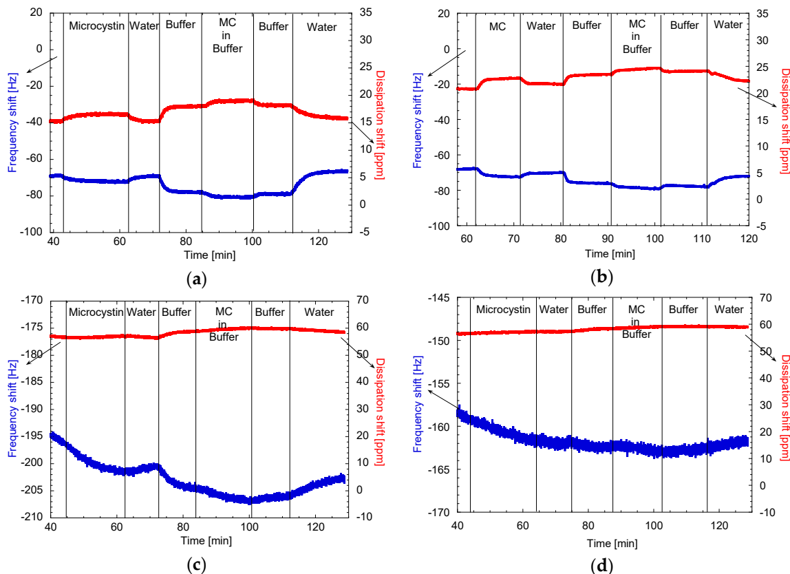
Figure 11. QCM-D sensograms of the adsorption of microcystin in water and Tris-HCl buffer from (a) CNF, (b) CNF and flushed CD (CNF + CD), (c) CNF-CD, and (d) CNF-PCD. CNF, cellulose nanofibrils; CD, cyclodextrin; CNF-CD, cellulose nanofibrils grafted with cyclodextrin; CNF-PCD, cellulose nanofibrils grafted with poly-cyclodextrin.
