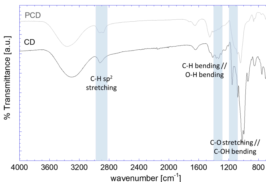
Figure 4. FTIR-ATR spectra of cyclodextrin and poly (cyclodextrin) obtained by crosslinking with epichlorohydrin.
