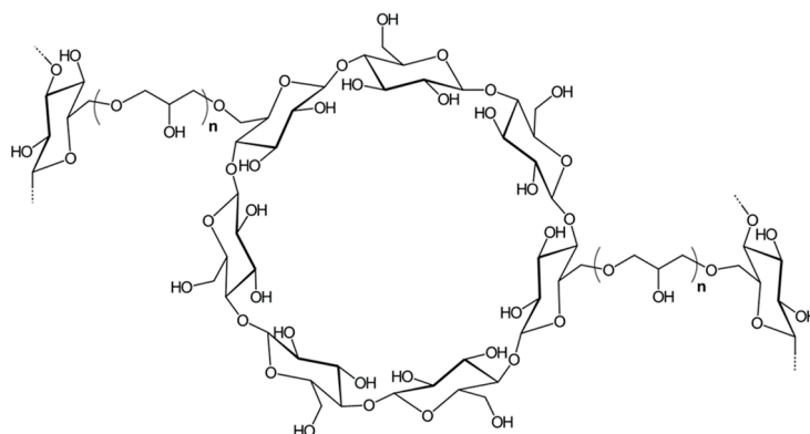
Figure 2. Expected structure of \beta -cyclodextrin crosslinked with other hydroxyl group from polysaccharides (cellulose or other cyclodextrins) through epichlorohydrin.
