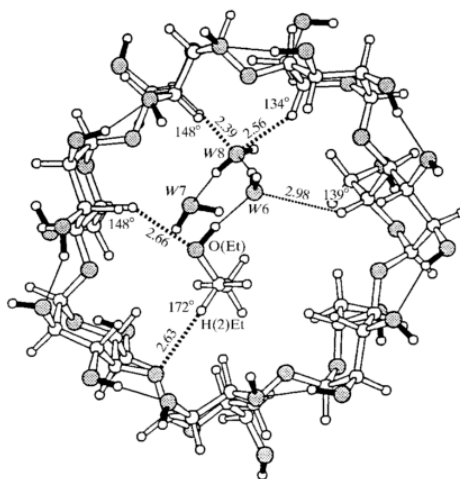
Figure 1. Neutron diffraction structure of \beta -cyclodextrin with ethanol complex. The hydrogen bonding capability can be observed through dash-lines. [17] Reproduced with the permission of International Union of Crystallography ( https://journals.iucr.org/ ).
