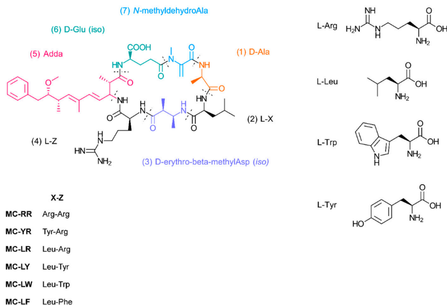
Figure 3. Basic chemical structure of microcystins. Amino acid residues 2 and 4 are interchangeable.
