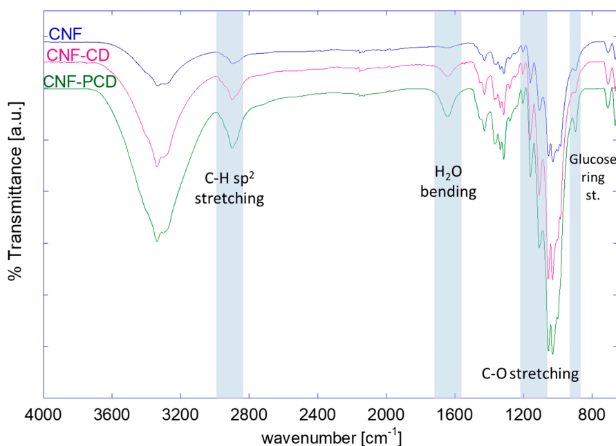
Figure 5. FTIR-ATR spectra comparing cellulose nanofibrils (CNF) and modified cellulose nanofibrils (CNF-CD and CNF-PCD).
