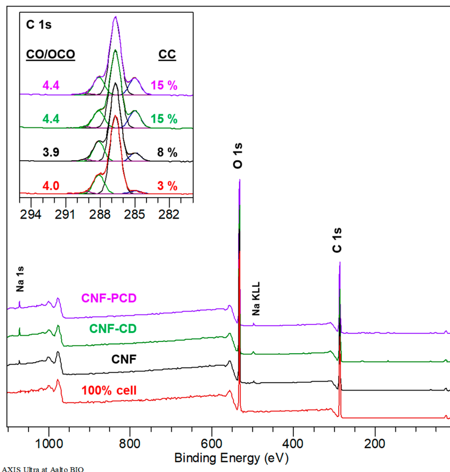
Figure 6. XPS wide energy region spectra comparing a pure cellulose reference, cellulose nanofibrils (CNF) and modified cellulose nanofibrils (CNF-CD and CNF-PCD). The insert shows the high-resolution C 1s spectra.
