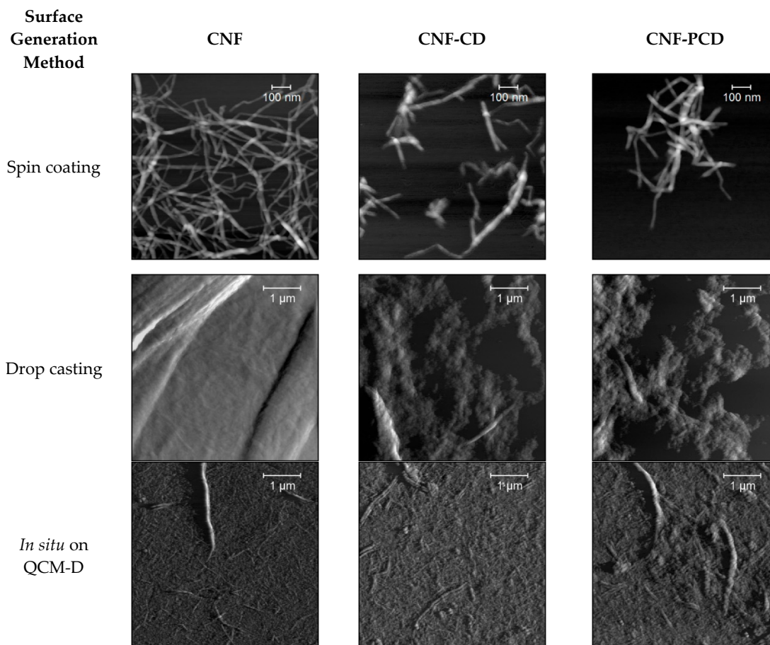
Figure 10. AFM images of the cellulose nanofibrils (CNF) and the modified cellulose nanofibrils (CNF-CD and CNF-PCD) and the average rugosity (Ra), each row was generated by a different technique, while the last one was measured after adsorption of microcystin in the QCM-D.
