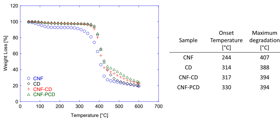
Figure 7. Thermogravimetric analysis of the CNF, CD, and the modified cellulose nanofibrils (CNF-CD and CNF-PCD). The thermogram (left) shows the behavior of the material, and the table (right) presents the main extracted data for each sample.
