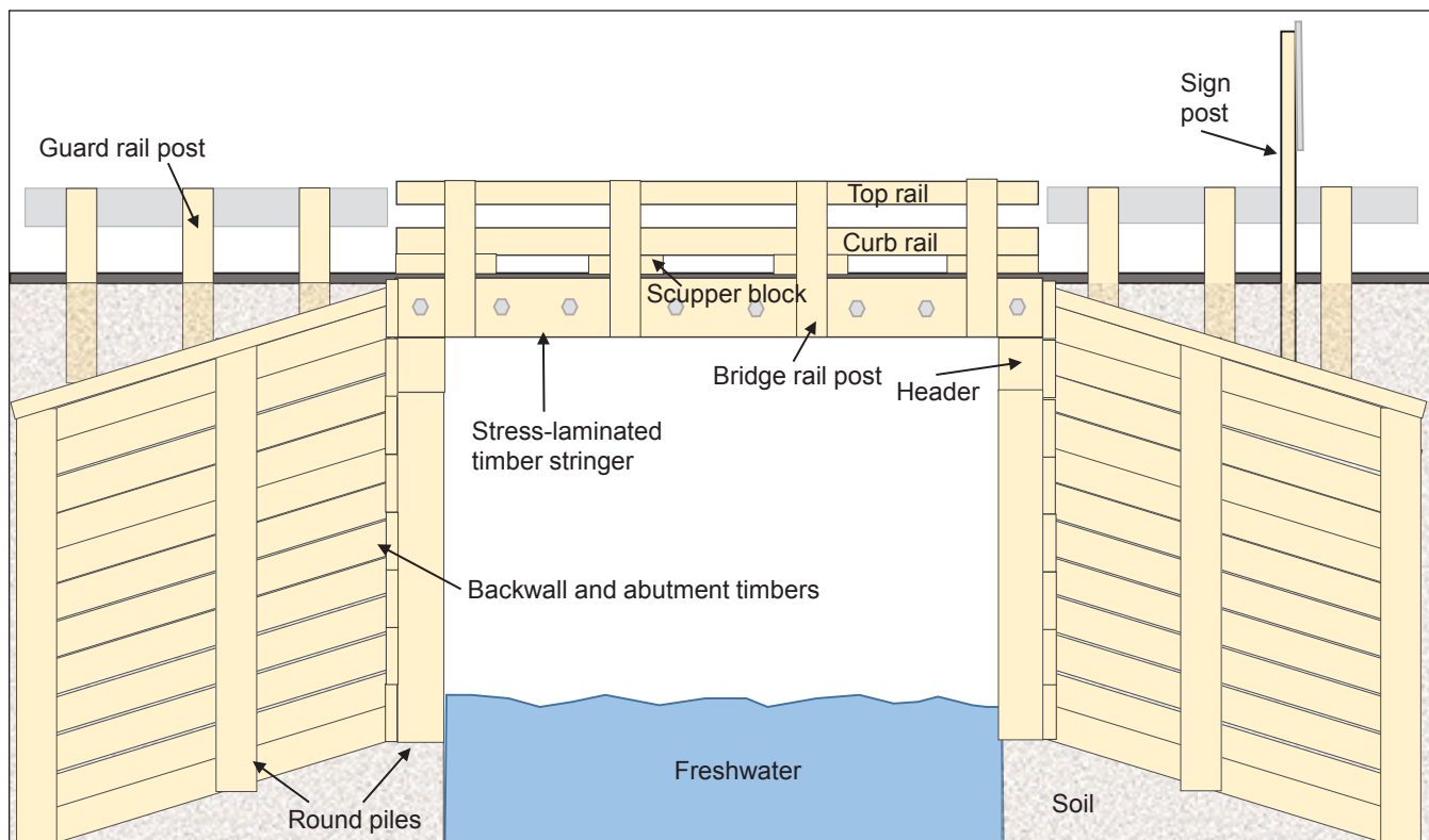
Figure 20. Pressure-treated wood components supporting a highway bridge are considered to be structurally critical and most are pressure-treated to meet AWP A Use Category 4C.
