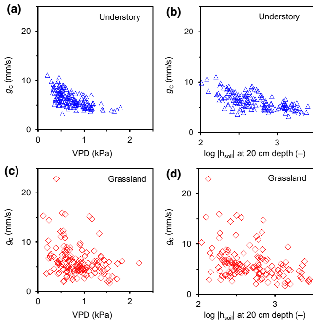
FIGURE 7 Relationship (a, c) between daily means of canopy conductance ( g_c ) and vapor pressure deficit, VPD, and (b, d) between daily means of g_c and the logarithm of soil pressure head ( \log |h_{\text{soil}}| ) at depth of 20 cm for understory (a, b) and grassland (c, d). Shown are daily data for days with rainfall < 1 mm during 2012 and 2013 growing seasons
