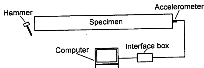
Figure 3. — Schematic of experimental set-up for stress-wave measurement.
