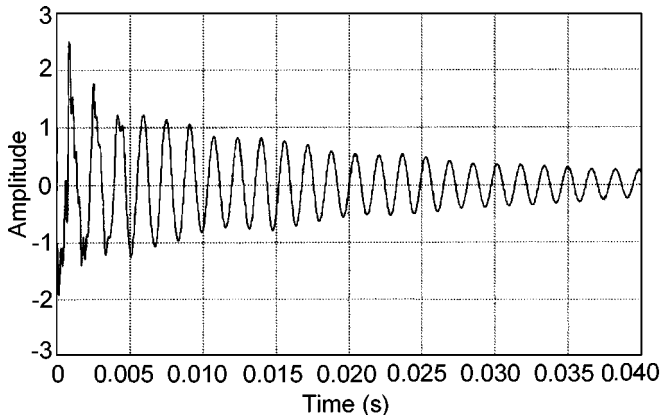
Figure 4—Time history of a typical stress waveform observed in a treated pile section (SP1C).
