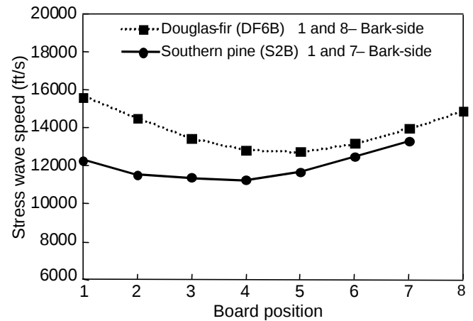
Figure 9—Variation of stress wave speed in an octagon along the radial direction across the board increment (1 ft/s = 0.31 m/s).
