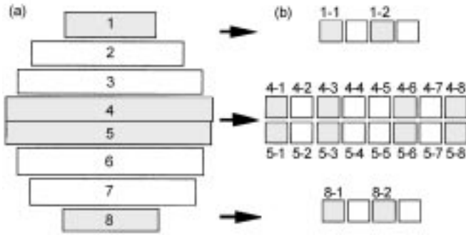
Figure 2—(a) Boards sawn from octagon cant and (b) small, clear wood specimens cut from two side boards and two middle boards.
