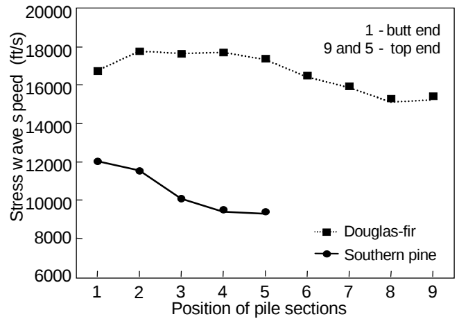
Figure 8—Variation of stress wave speed along the length of a pile (1 ft/s = 0.31 m/s).
