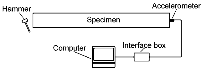
Figure 3—Experimental setup for stress wave measurement.
