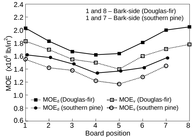
Figure 10—Variation of MOE in an octagon along the radial direction across the board increment (1 lb/in 2 = 6.895 kPa).
