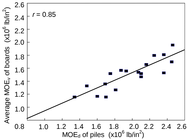
Figure 6—Average MOE v of boards plotted with MOE d of piles (1 lb/in 2 = 6.895 kPa).
