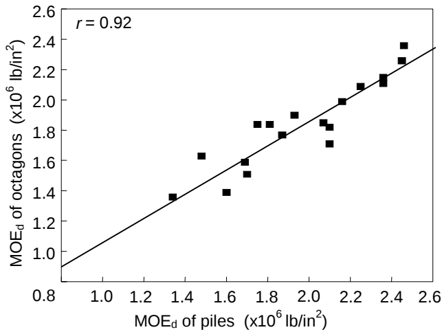
Figure 5—MOE d of piles plotted with MOE d of octagons (1 lb/in 2 = 6.895 kPa).
