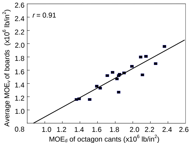
Figure 7—Average MOE v of boards plotted with MOE d of octagon cants (1 lb/in 2 = 6.895 kPa).
