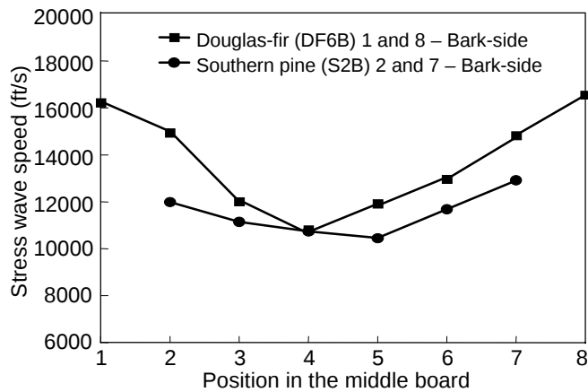
Figure 11—Variation of stress wave speed (SWS) in the middle board along the radial direction (1 ft/s = 0.31 m/s).
