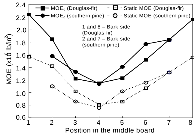
Figure 12—Variation of MOE in the middle board along the radial direction (1 lb/in 2 = 6.895 kPa).
