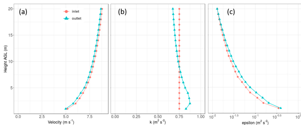
Figure 2. Profiles for (a) velocity, (b) turbulent kinetic energy (TKE), and (c) dissipation of TKE over flat terrain.
