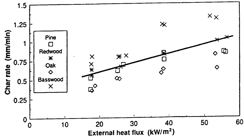
Fig. 2—Char rate \beta (l/m, of Eq. (1)) versus external heat flux. Line is Equation (3).
