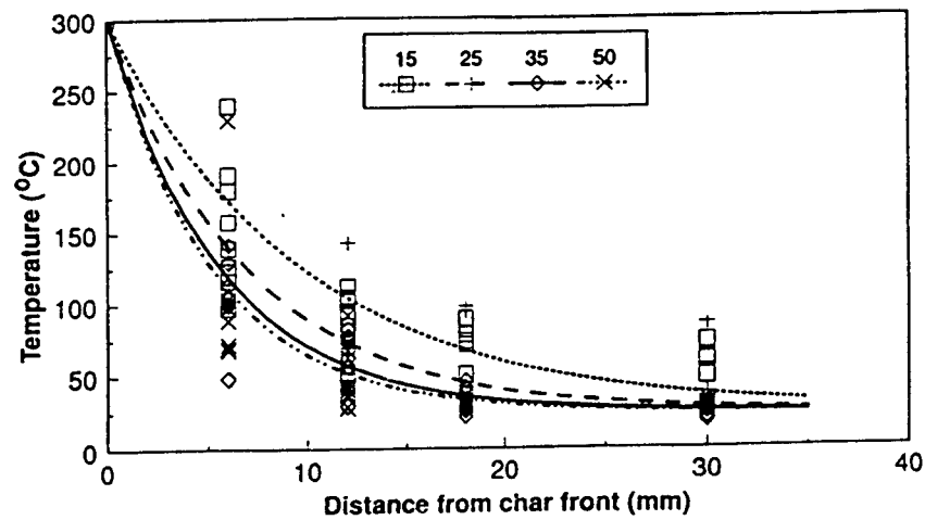
Fig. 3—Temperature profiles in uncharred wood when char front (300°C) is 6 mm from original exposed surface, based on combined data sets of same nominal heat flux level (15, 25, 35, and 50 kW/m 2 ).
