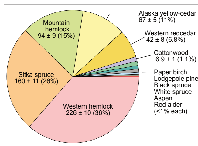
Figure 24—Distribution of aboveground live tree ( \geq 1 inch diameter at breast height) carbon mass among species in coastal Alaska. Values are in million Mg C ( \pm 1 standard error) and percentage of total carbon mass (~620 million Mg C) throughout the inventory unit.
