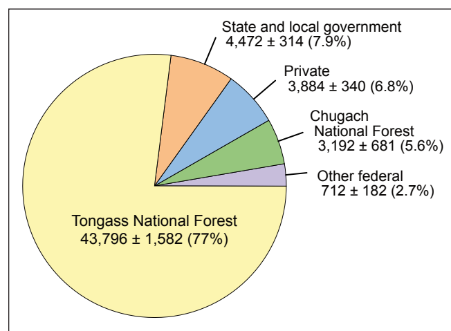
Figure 16—Net volume of live trees across ownership groups. Values are in million cubic feet ( \pm 1 standard error) and percentage of total volume.
