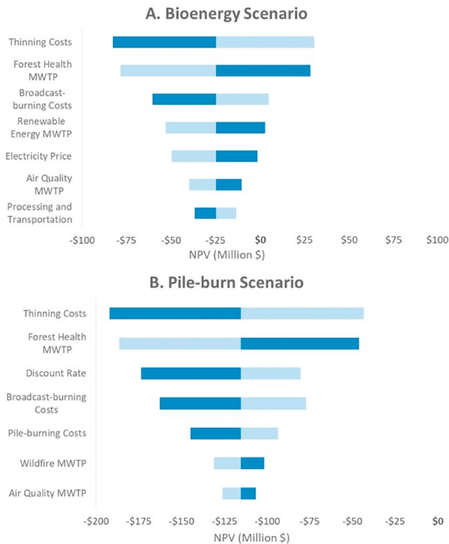
Fig. 3. Sensitivity tornado for Bioenergy and Pile-burn Scenarios. Bars represent each variable's effect on mean NPV across its distribution (Table 5), with all other variables held at mean values. Dark shaded bars represent an increase in the input value of the variable and light shaded bars represent decrease in input value.
