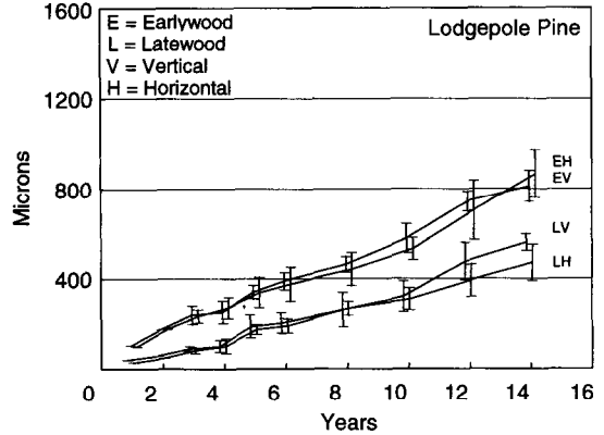
FIG. 3. Erosion of vertical-grained lodgepole pine as a function of years of exposure (average of measurements on three replicate specimens). Bars indicate standard deviation and are offset for clarity.
