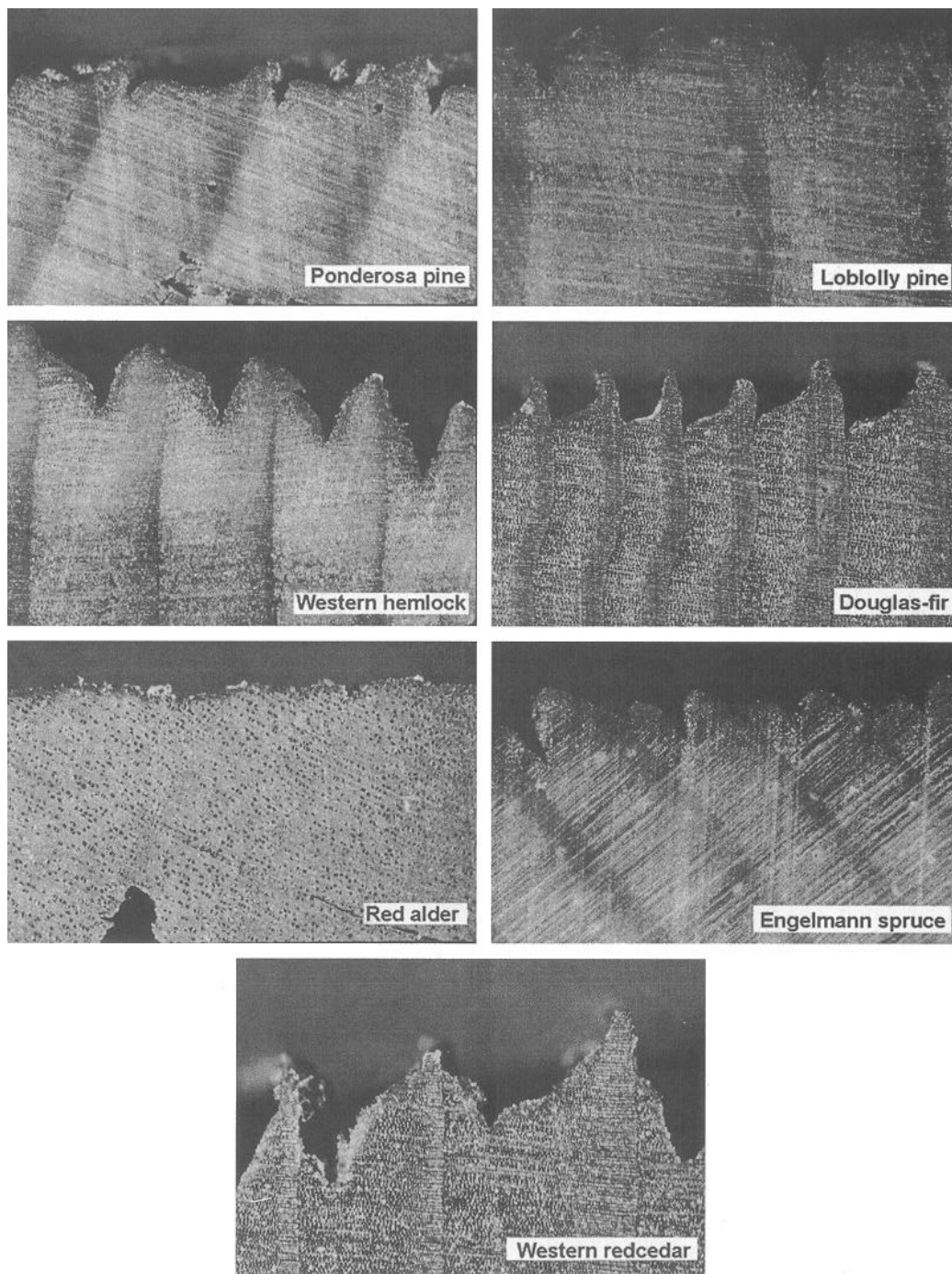
FIG. 7. Erosion of earlywood and latewood in weathered specimens of various species.
