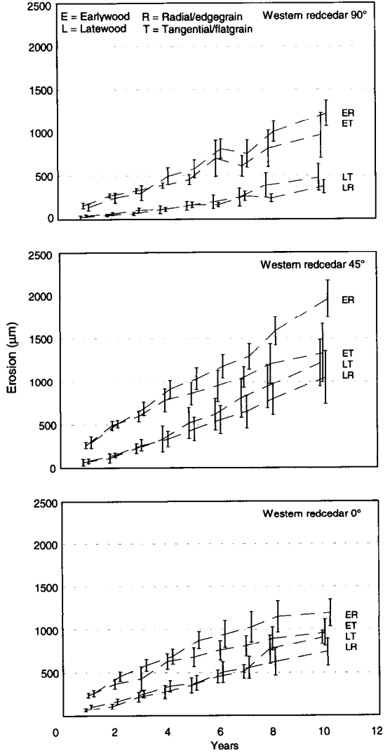
FIG. 4. Erosion of radial and tangential surfaces of western redcedar at various angles of exposure as a function of exposure period (average of three measurements on three replicate specimens). Bars indicate standard deviation and are offset for clarity.
