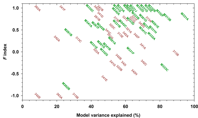
Figure 3. Relationship between F index (fuel/flammability control) and model variance explained for ecosections. Colors indicate Bailey “-” (brown) versus “M” (green) classification. To facilitate plotting and minimize overlap, especially among ecosections with F \sim 1 , slight jitter was applied.
