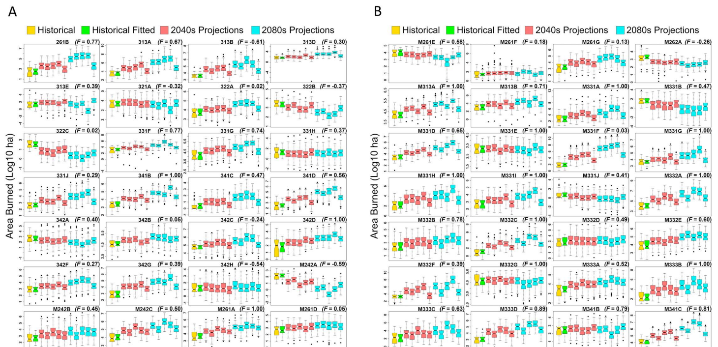
Figure 4. (a) Boxplots of historical, 2040s projected, and 2080s projected area burned by ecosection. Future scenarios, left to right, are 10 GCM composites, ECHAM5, HadGEM1, MIROC3.2, and PCM1. (b) Same as in Figure 4a.
