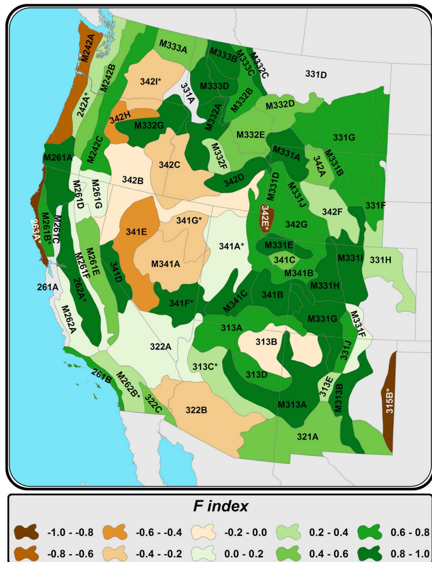
Figure 1. Western U.S. Bailey ecosections classified by climatic controls of area burned according to F index, a continuous indicator of fuel-to-flammability limitation determined by the relative importance of climate variables explaining variability in annual area burned (see Table 1 and diagnostics in the supporting information Table S1). Asterisks indicate ecosections for which statistical relationships allowed classification but statistical models were either weak or violated one or more diagnostic tests. Note that ecosection boundaries M313B (Sacramento/Manzano Mountains, NM), 321A (Chihuahuan Basin and Range), 315B (Southwest Texas High Plains), 331F (Northwestern Great Plains), and 331H (Central High Plains) are mapped only for the portion of the ecosection within one or more of the eleven western states from which fire data was extracted.
