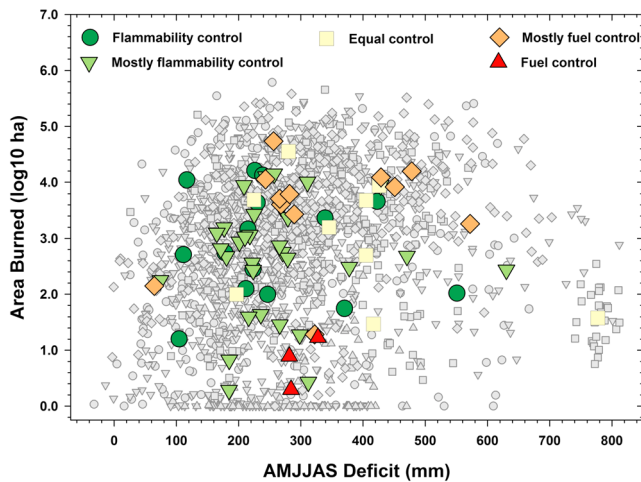
Figure 2. Relationship between fire season deficit and annual area burned across all 70 ecosystems. Large colored symbols represent ecosystem means for 1980–2006, gray symbols indicate individual years.
