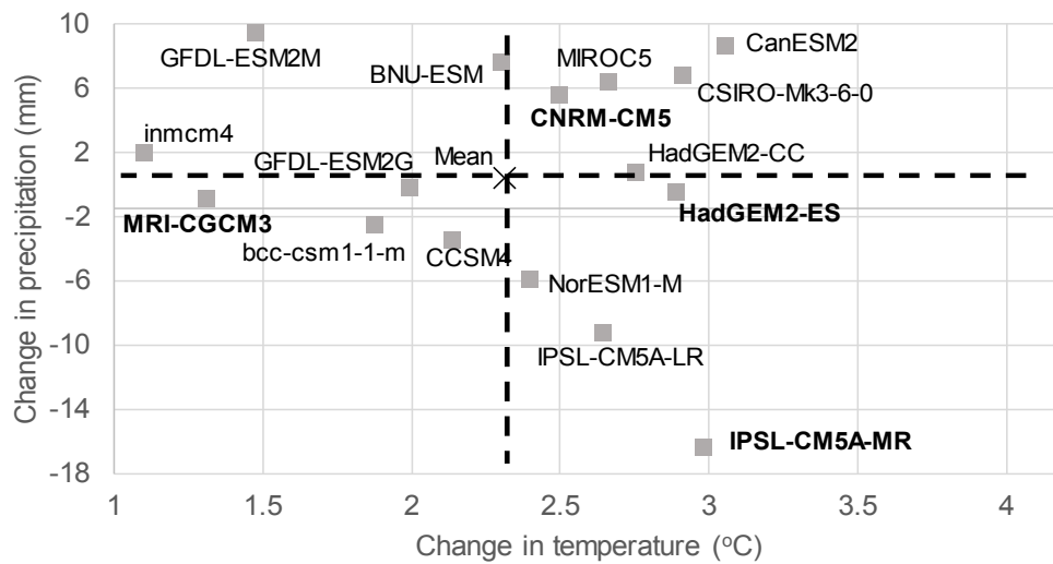
(a) RCP 4.5
