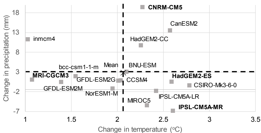
(a) RCP 4.5
