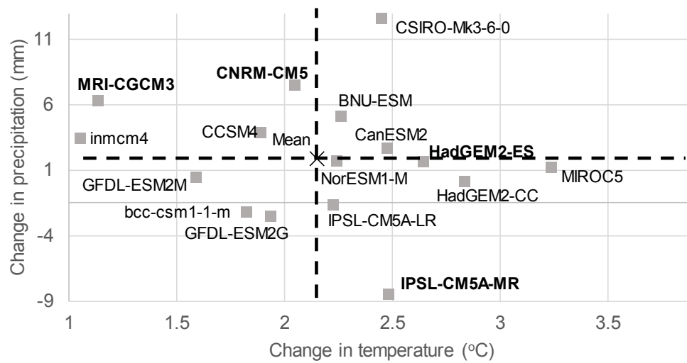
(a) RCP 4.5
