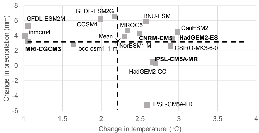
(a) RCP 4.5
