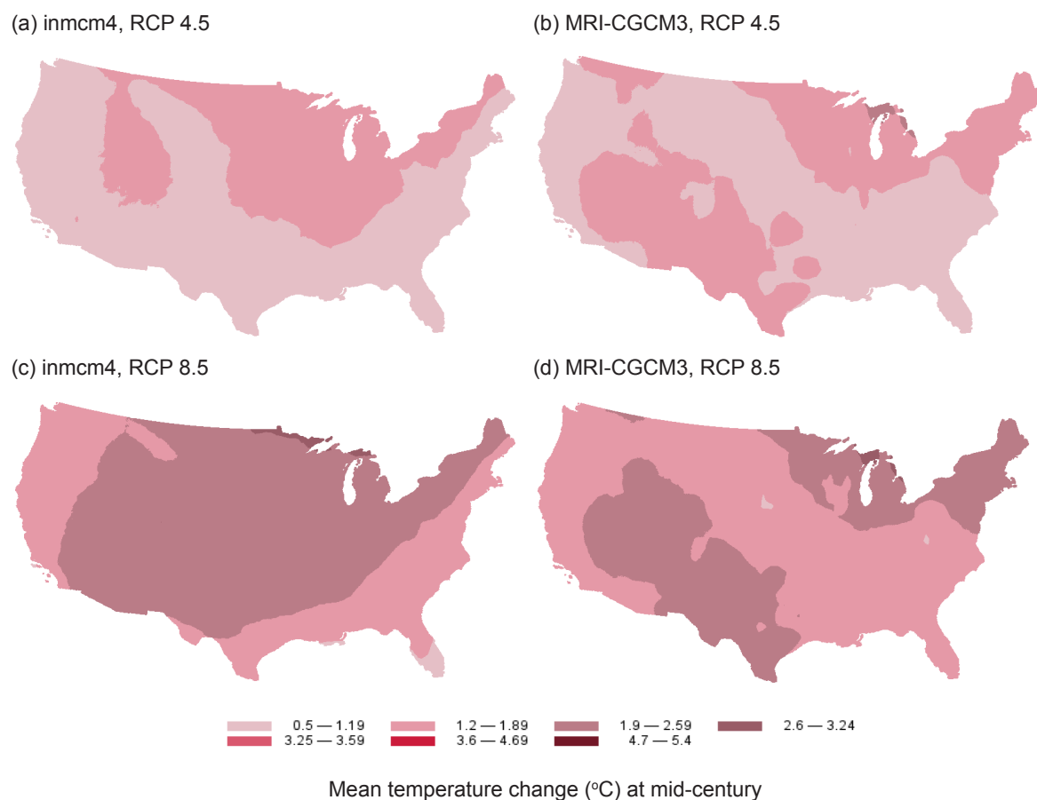
Figure 4 —Mean temperature change (°C) at mid-century (2041–2070) from the historical period (1971–2000) as projected by the inmcm4 model under RCP 4.5 (a) and RCP 8.5 (c) and the MRI-CGCM3 model under RCP 4.5 (b) and RCP 8.5 (d).
