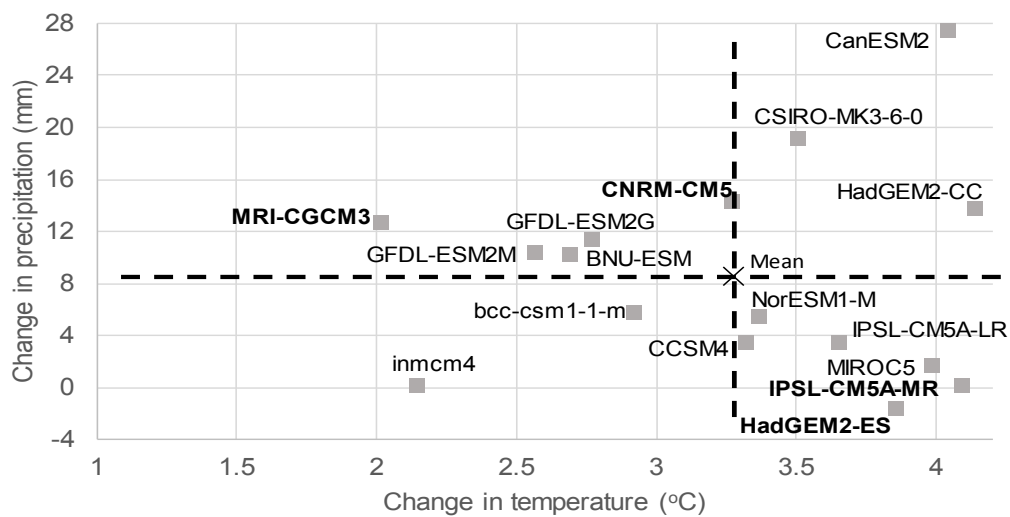
(b) RCP 8.5
