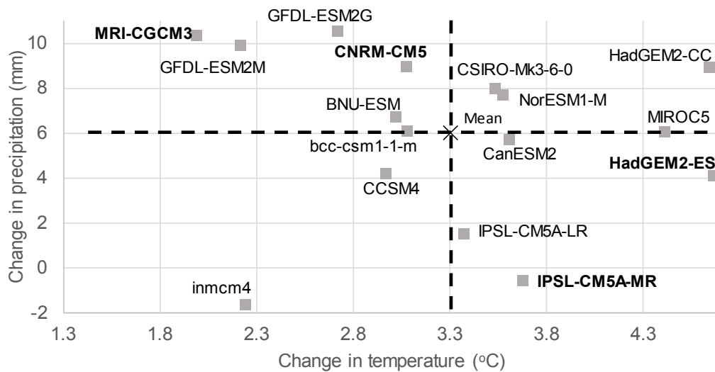
(b) RCP 8.5
