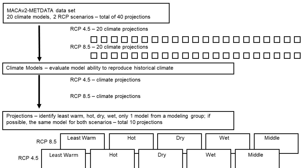
Figure 1 —Process used to identify five climate projections from the MACAv2-METDATA climate dataset to be used under RCP 4.5 and RCP 8.5 in the 2020 RPA Assessment.
