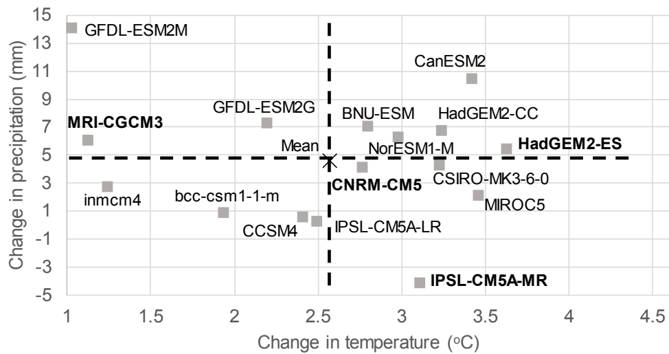
(a) RCP 4.5
