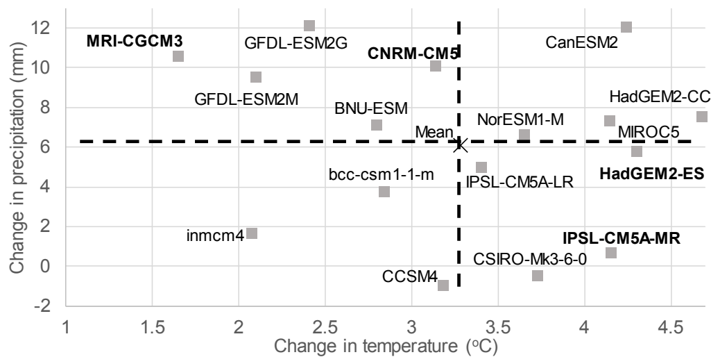
(b) RCP 8.5
