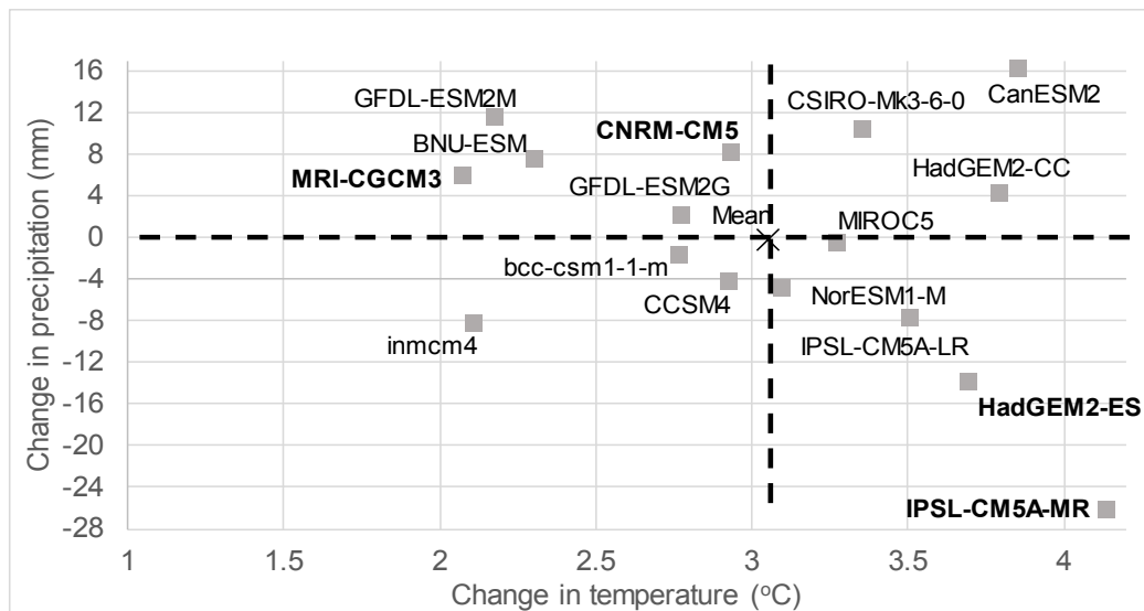
(b) RCP 8.5
