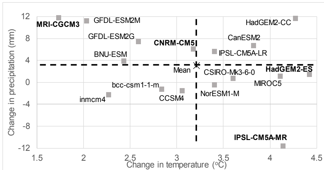
(b) RCP 8.5
