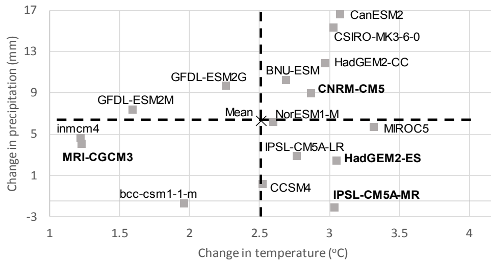
(a) RCP 4.5
