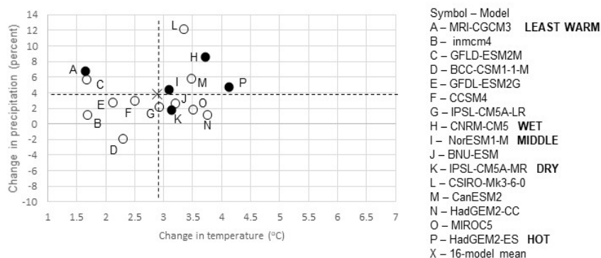
(b) RCP 8.5
