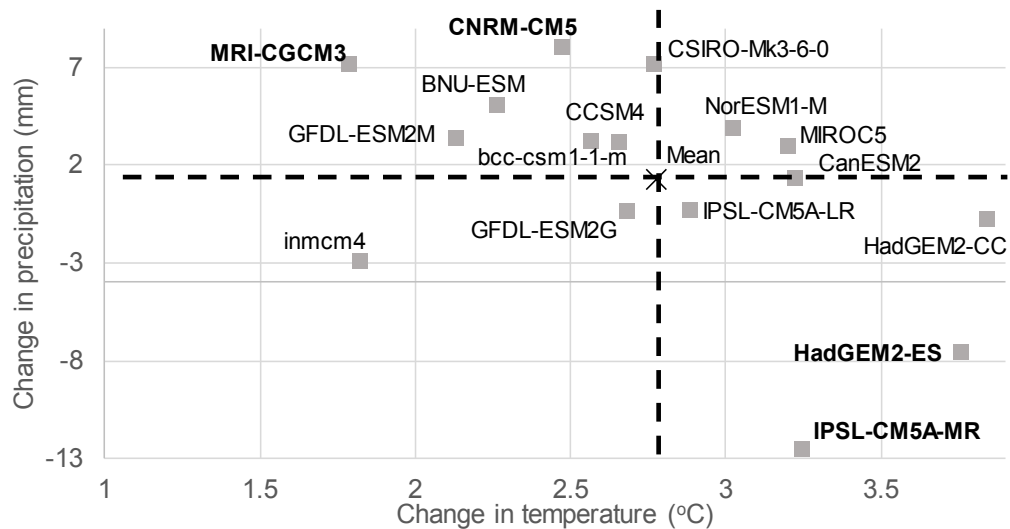
(b) RCP 8.5
