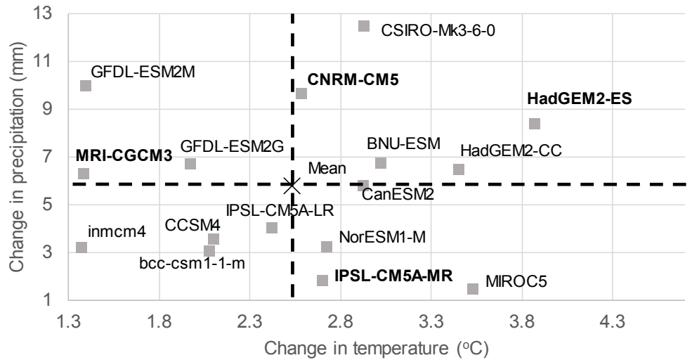
(a) RCP 4.5
