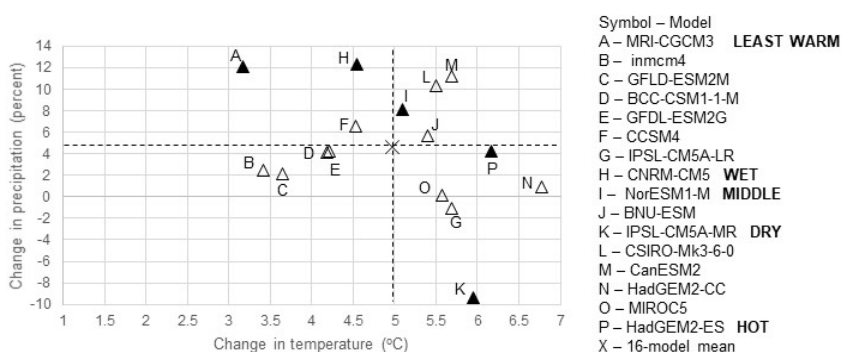
(b) RCP 8.5
