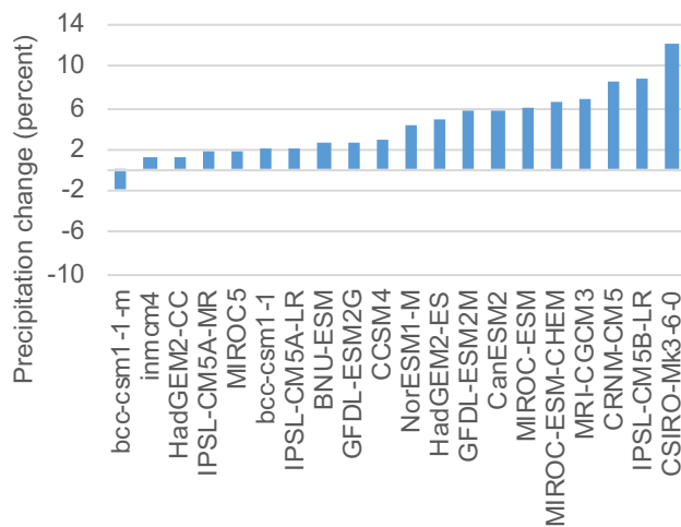
Figure 19 —Area-weighted change in mean temperature (°C) and annual precipitation (percent) at end of century (2070–2099) from the historical period (1971–2000) under RCP 4.5 (a,c) and RCP 8.5 (b,d) for all 20 models at the conterminous U.S. scale. Poor performing models retained here for comparison only (MIROC-ESM, MIROC-ESM-CHEM, bcc-csm1-1, IPSL-CM5B-LR).
