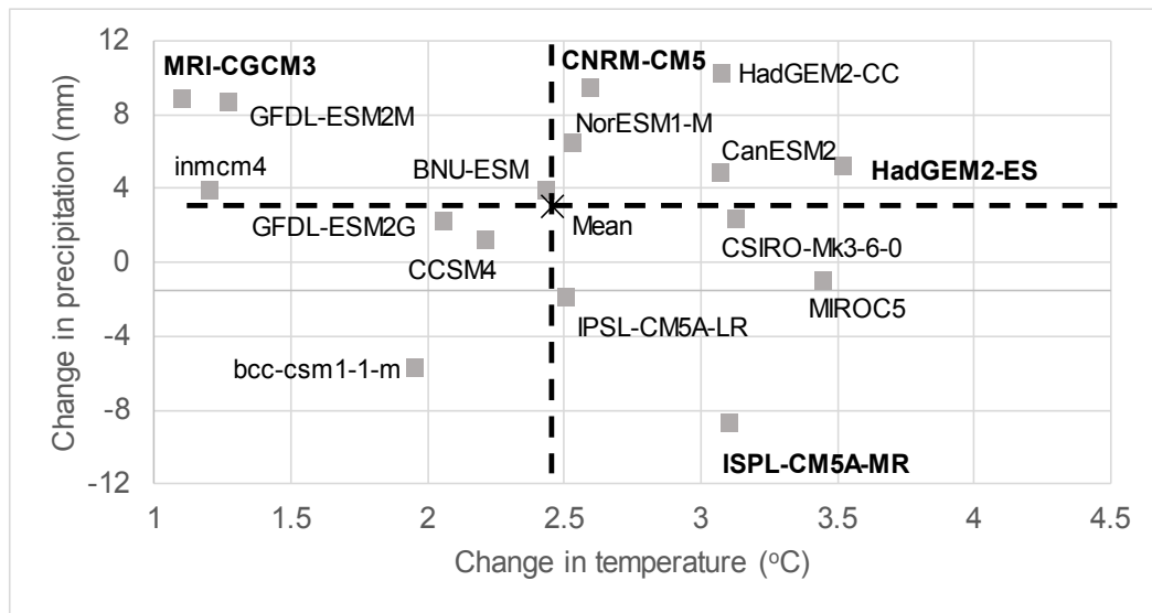
(a) RCP 4.5
