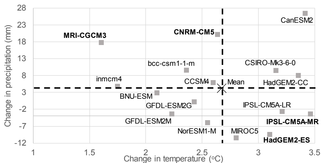
(b) RCP 8.5
