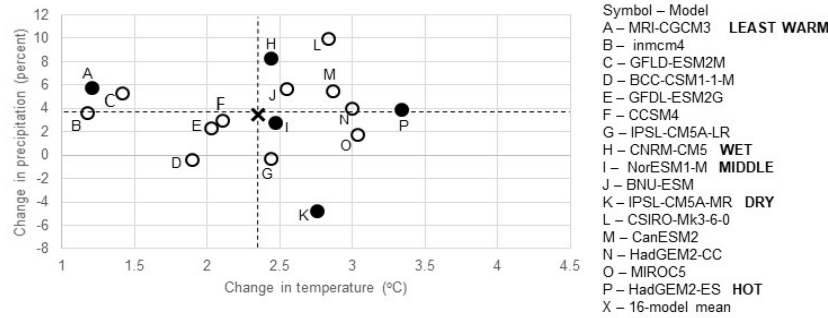
(b) RCP 8.5
