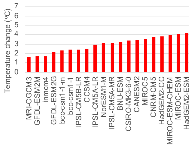
(c) RCP 4.5
