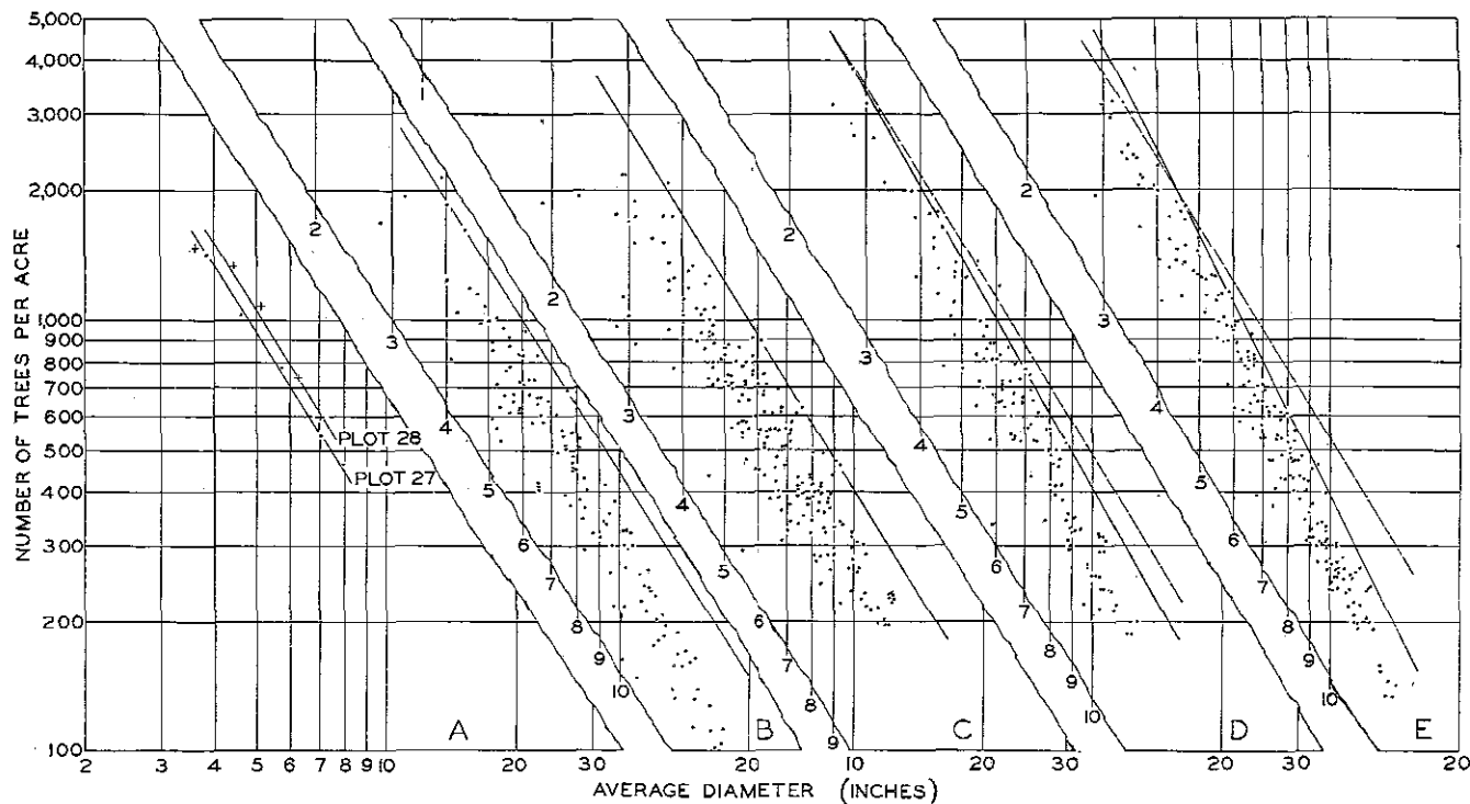
FIGURE 7.—Agreements with and divergences from the reference curve in different species. Parallelism is found in (A) loblolly pine at 5-year intervals, on permanent plots, (B) temporary yield-plot data for loblolly pine, and (C) longleaf pine; divergence is noted to a slight degree in (D, dotted line) slash pine, and more definitely in (E, dotted line) shortleaf pine
