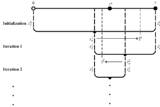
Figure 3.1 — Solving the consumer's problem (von Haefen et al., 2004)
