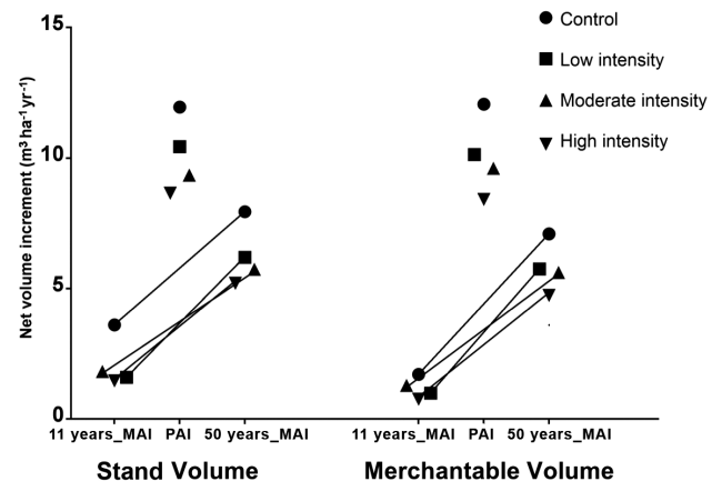
Figure 4. Mean annual increment (MAI) of stand volume and merchantable volume 11 years and 50 years after treatment and the periodic annual increment (PAI) for the time span in between.
