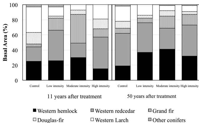
Figure 3. Species composition of different treatments 11 years and 50 years after thinning. Species are presented in order of shade tolerance with western hemlock as the most shade-tolerant and western larch the least shade-tolerant. Other conifers could include Engelmann spruce, subalpine fir, and western white pine, lodgepole pine, or ponderosa pine.
