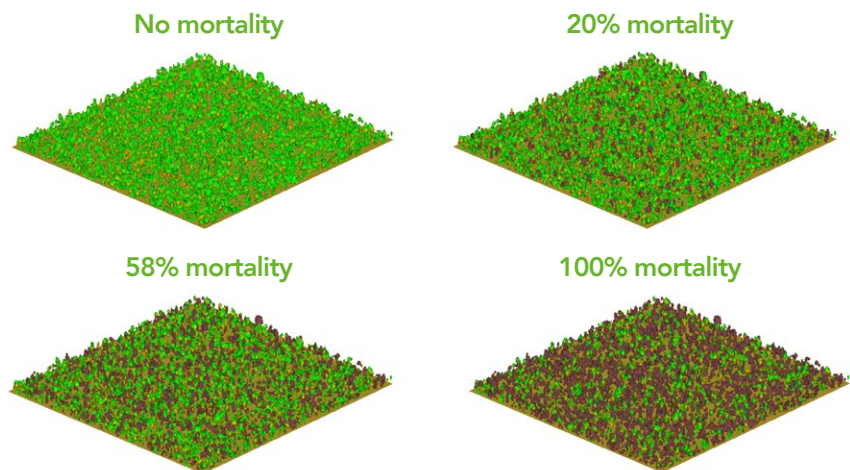
Fire behaviour simulations: field data was used to create analogous forest. 4 levels of fire mortality were simulated.
