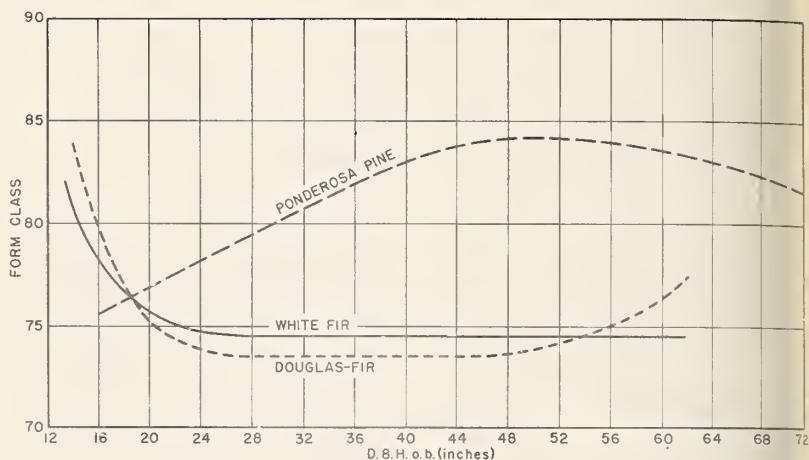
Fig. 1 - Average form class by d.b.h. of the sample trees used in preparing the volume tables.
