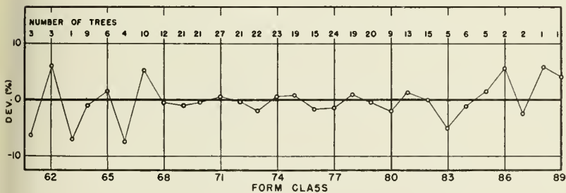
Fig. 4 - Difference between tubular and scoled volumes to 10 inch top, of individual red fir trees, grouped by log height, d.b.h., and form class.
