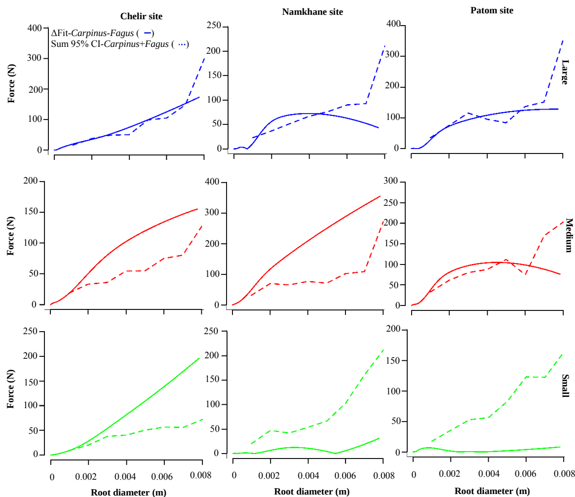
Figure 5. Calculation of difference between the fitting curves of tensile force vs. root diameter for Carpinus
