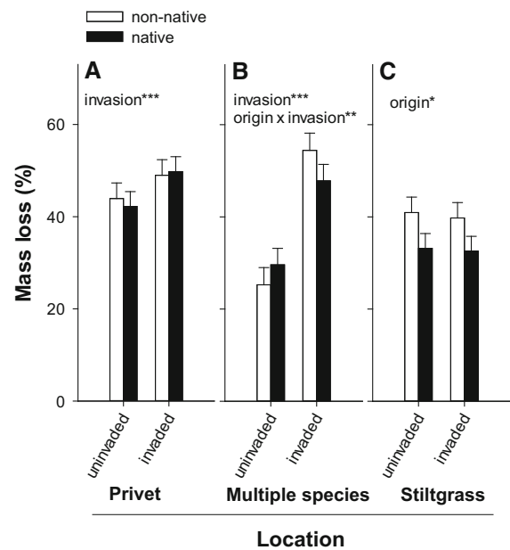
Fig. 3 Percent mass loss (LS-means \pm SE) for non-native (open bars) vs. native wood (closed bars) species placed in uninvaded and invaded sites at three locations. The individual locations included sites invaded by Ligustrum (a), multiple plant species (b) or by Microstegium (c). Although all six sites were invaded to some extent by non-native plants, they are labelled here as uninvaded or invaded for simplicity. Asterisks next to significant effects indicate the level of significance: P < 0.1^* , P < 0.05^{**} , and P < 0.01^{***} . Invasion refers to whether the sites were invaded or uninvaded and origin distinguishes between non-native and native wood species
