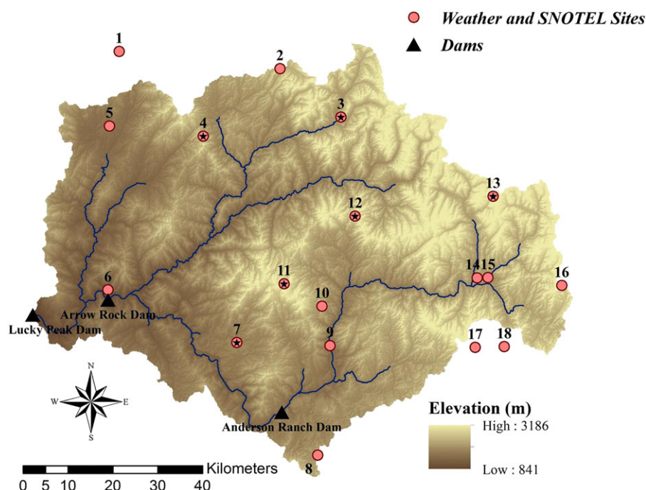
FIGURE 1 Digital elevation map of the Boise River Basin showing the location of weather and SNOTEL sites. Black stars indicate SNOTEL sites with snow water equivalent measurements, which were used in the evaluation of model performance
