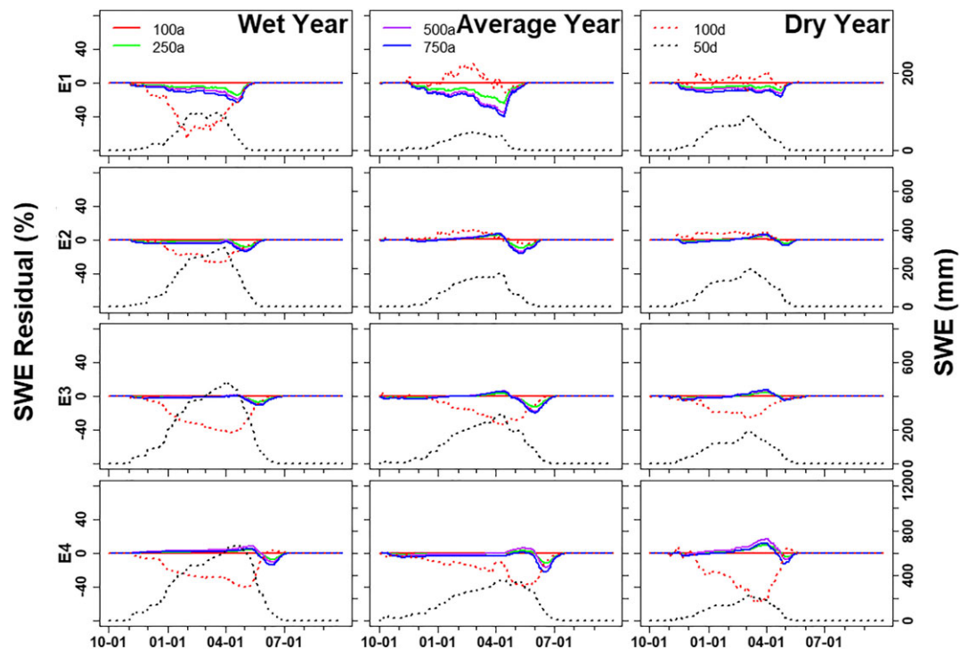
FIGURE 3 Aggregated estimated snow water equivalent (SWE) over four elevation bands. Dotted lines show the 50-m (d) and 100-m (d) scenarios, but solid lines indicate the aggregated scenarios (from the 100 (a) to 750 m (a)). Primary (left) axis shows residuals, the estimated SWE generated from all the scenarios minus that of the 50-m (d) scenario. Secondary Y (right) axis shows the estimated SWE from the 50-m (d) scenario
