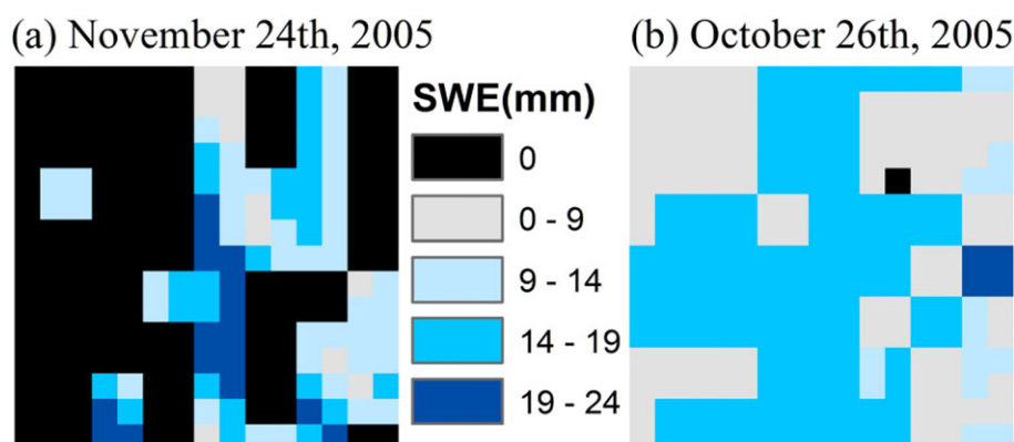
FIGURE 4 Subgrid variability of snow water equivalent (SWE) in (a) the 750 m-E2-cell and (b) 750 m-E4-cell
