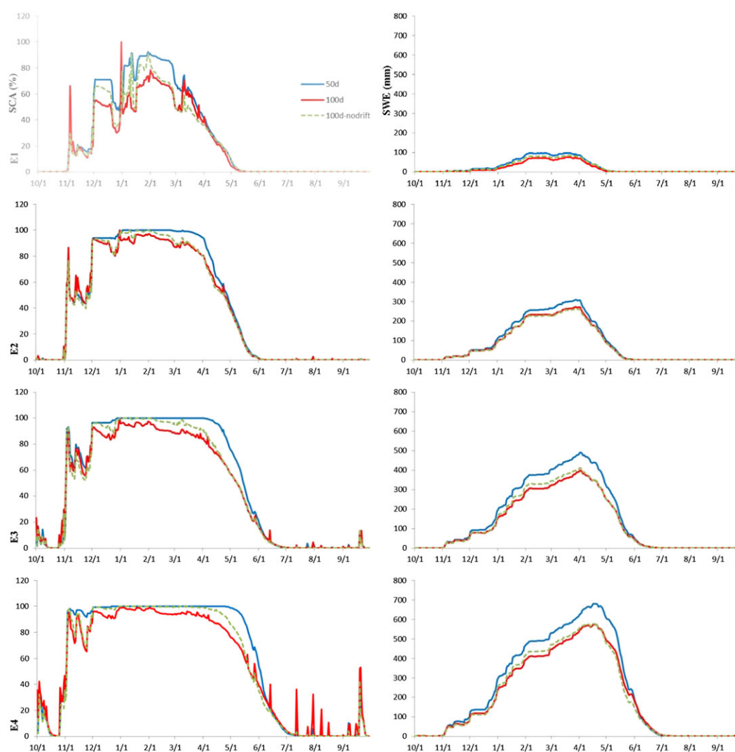
FIGURE 7 The scaling effect on the estimation of snow-covered area (SCA) and snow water equivalent (SWE) once the effect of scaling on wind-induced snow drifting was removed. The left column indicates the estimated SCA, and the right column shows the estimated SWE for the 50-m (d; solid blue line), 100-m (d; solid red line), and 100-m (d)-nodrift (dotted green line) scenarios for the wet year over the elevation bands
