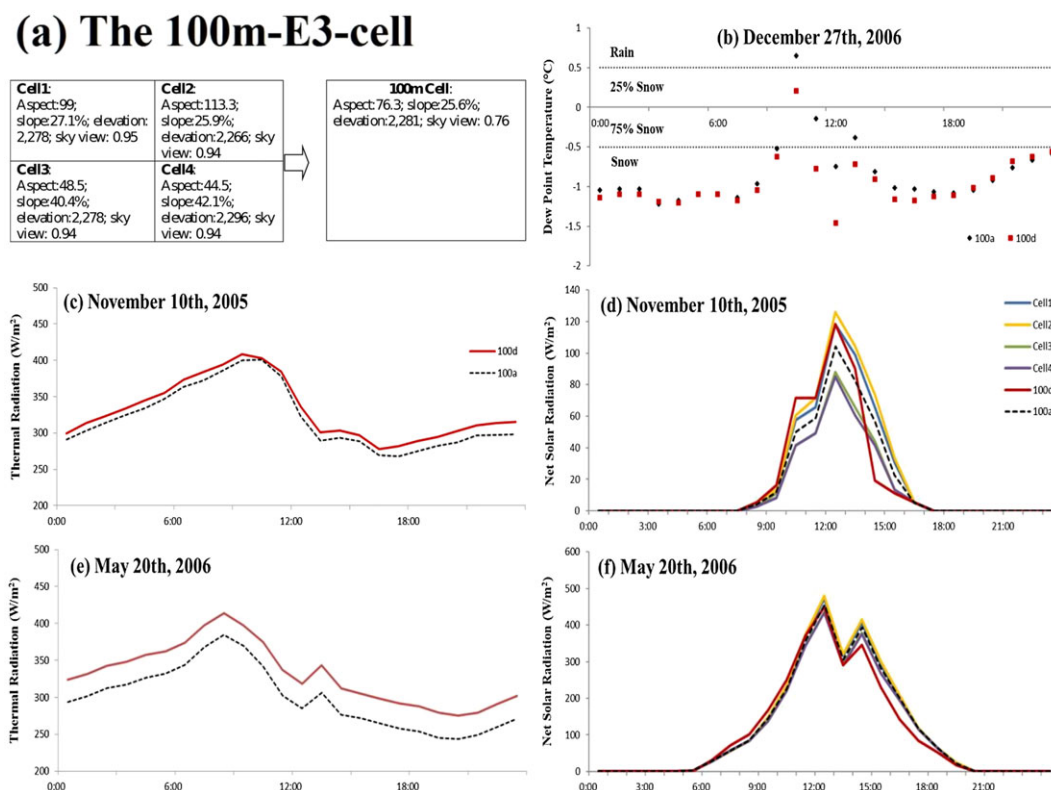
FIGURE 6 Differences in the estimated net solar and thermal radiations and dew point temperatures of the 50-m (d) or 100-m (a) scenarios and those of the 100-m (d) scenario. Panel (a) indicates that the establishment of 50-m (d) and 100-m (a) scenarios were very similar
