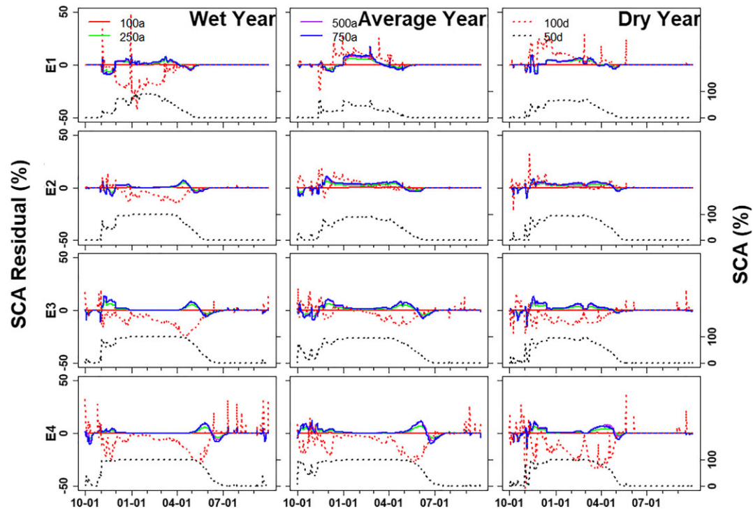
FIGURE 2 Aggregated estimated snow-covered area (SCA) over four climatic regions represented by elevation bands. Dotted lines show the 50-m (d) and 100-m (d) scenarios, and solid lines indicate the aggregated scenarios (100 m (a) through 750 m (a)). The primary Y (left) axis shows residuals between the estimated SCA generated from all the scenarios compared with that of the 50-m (d) scenario. The secondary Y (right) axis shows the estimated SCA from the 50-m (d) scenario
