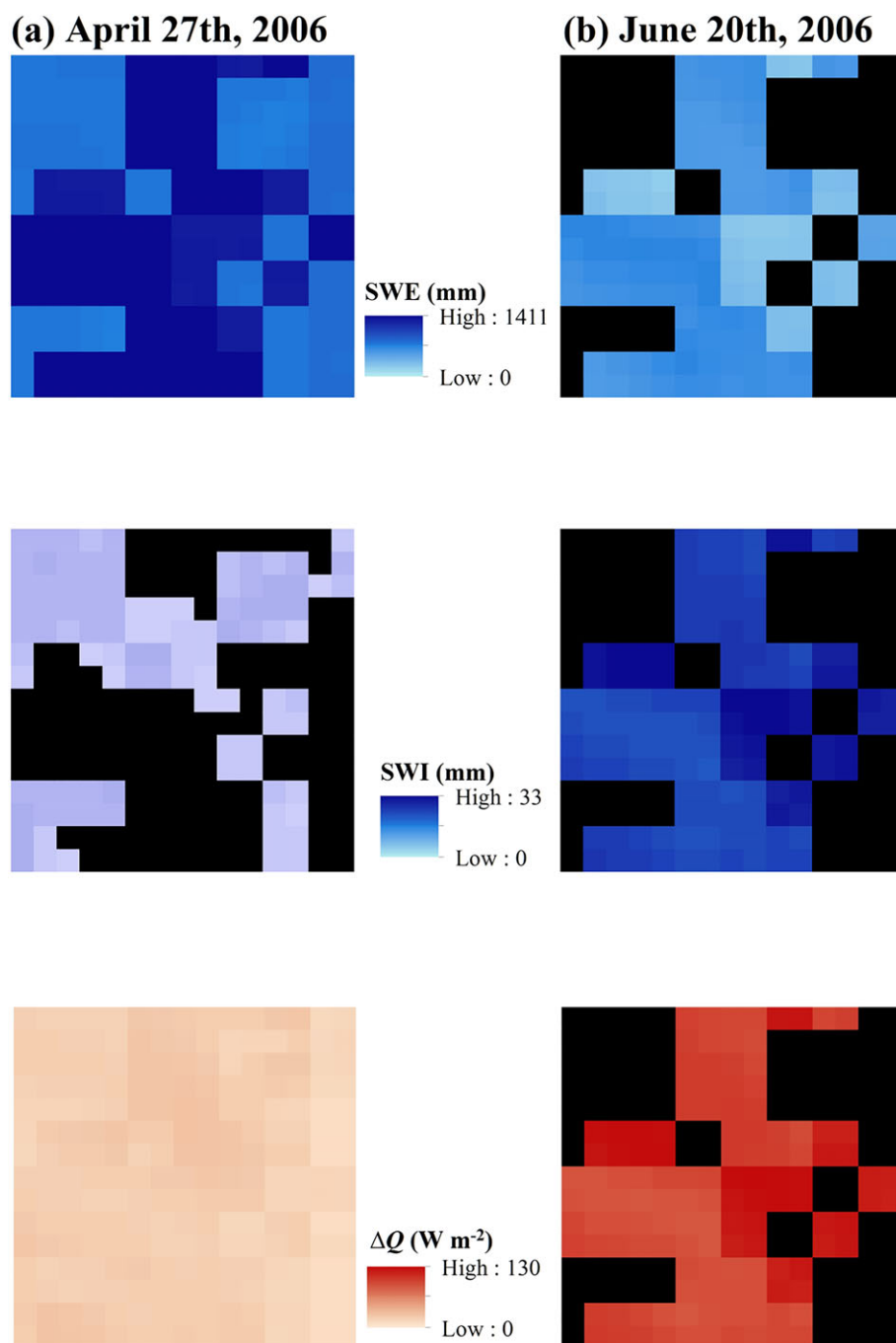
FIGURE 5 Subgrid variability of snow water equivalent (SWE), surface water input (SWI), and \Delta Q in the 750 m-E4-cell
