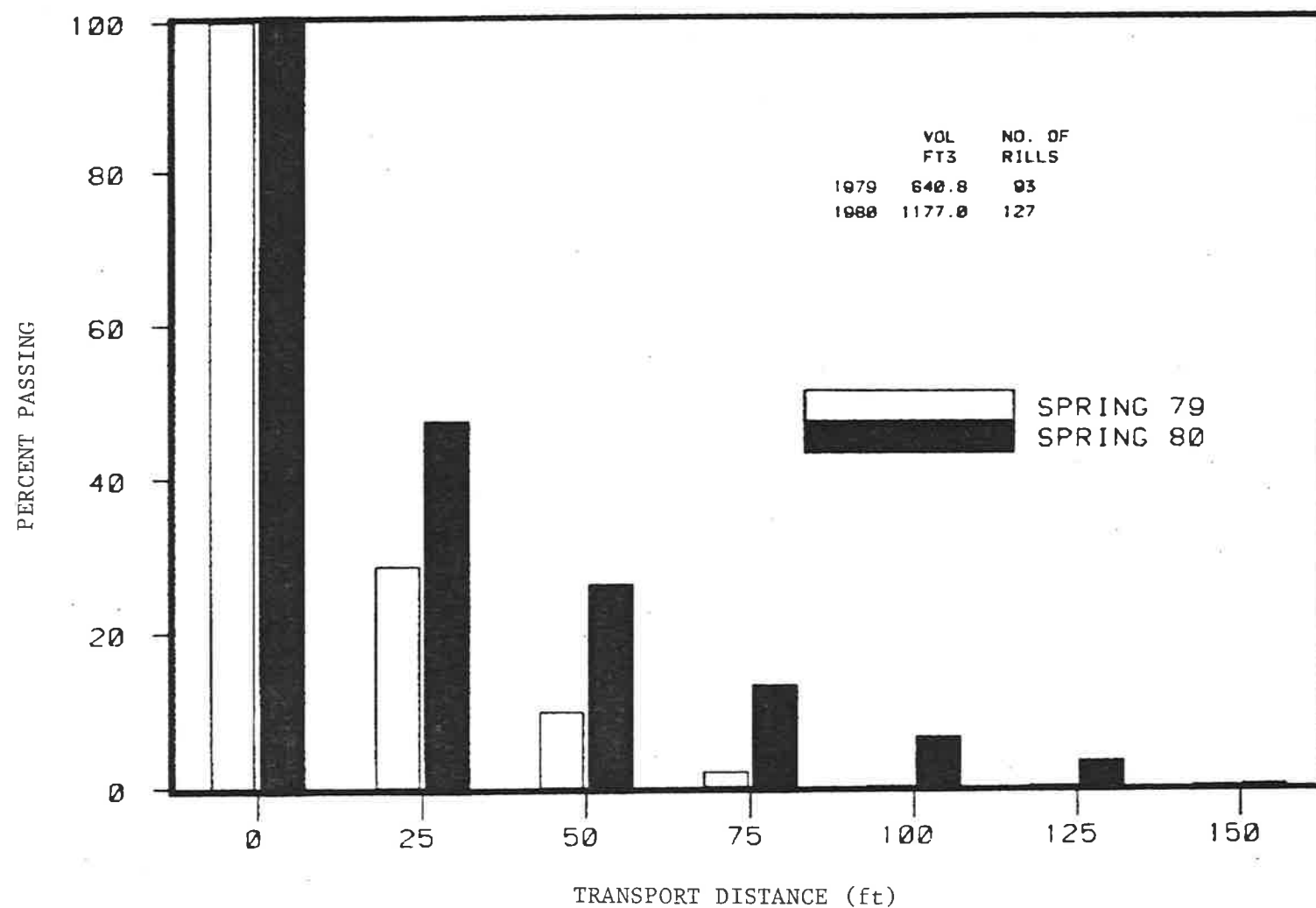
Figure 10. The percentage of material passing a defined downslope distance for the spring of 1979 and 1980.
