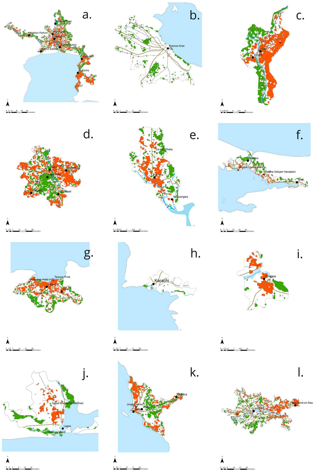
FIGURE 3A | The hot spot (green) and cold spot (red) clusters, city centers (dots), waters (blue), expressways (yellow lines), railways (black hashed lines), marine ports (anchors), airports (airplanes) within the metropolitan areas of: (a) Bangkok, (b) Buenos Aires, (c) Cairo, (d) Delhi, (e) Dhaka, (f) Istanbul, (g) Jakarta, (h) Karachi, (i) Kinshasa, (j) Lagos, (k) Lima, (l) London.
