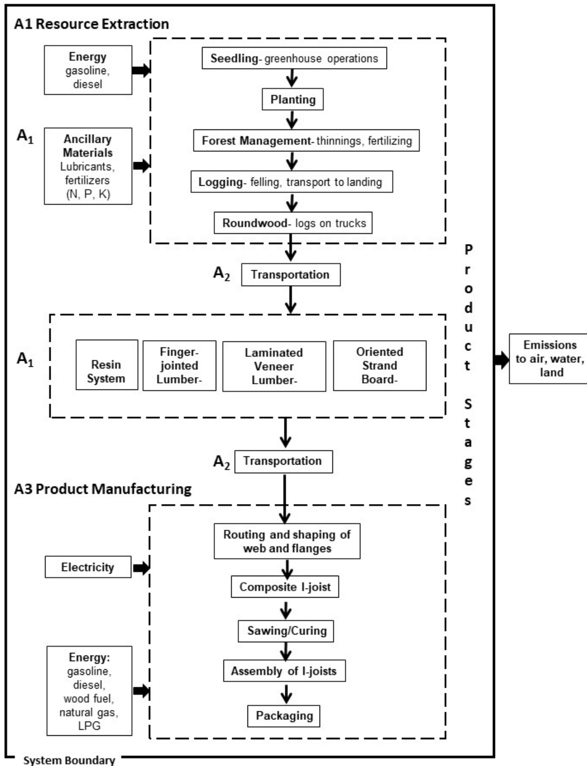
Figure 1 Cradle-to-gate system boundary for composite I-joist production in the SE region
