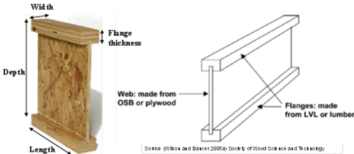
Figure 2. Typical composite I-joists shown here made with laminated veneer lumber (LVL) flanges and an oriented strandboard (OSB) web.
