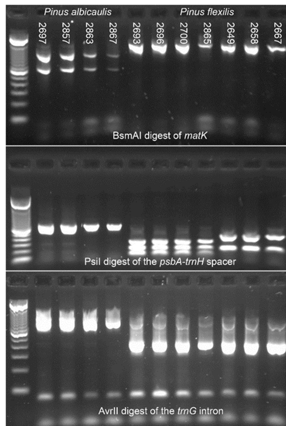
Figure 2. Restriction enzyme digests of whitebark ( Pinus albicaulis , lanes 2697 to 2867) and limber pine ( Pinus flexilis , lanes 2693 to 2667) PCR amplicons. The 12 lanes in each of the three panels represent the same DNA sample. The left-hand lane in each panel represents a 100 bps DNA ladder. Subsequent lanes are labeled by the DNA isolate number, from 2697 to 2667, the information for which is reported in the Supplemental Table S1.
