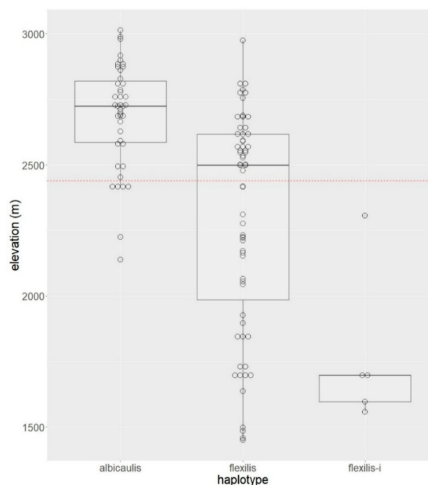
Figure 5. Dotplots with boxplot overlays showing the range of elevation for each of the three chloroplast DNA psbA-trnH haplotypes ( n = 43, 63 , and 5 for the “albicaulis”, “flexilis”, and “flexilis-i” haplotypes, respectively). The box captures 50% of the data points and the thick horizontal bar represents the median. Data points above and below the whiskers represent outliers. The red dashed line represents the 2440 m threshold above which five-needle pines lacking cones conventionally are assigned to whitebark pine.
