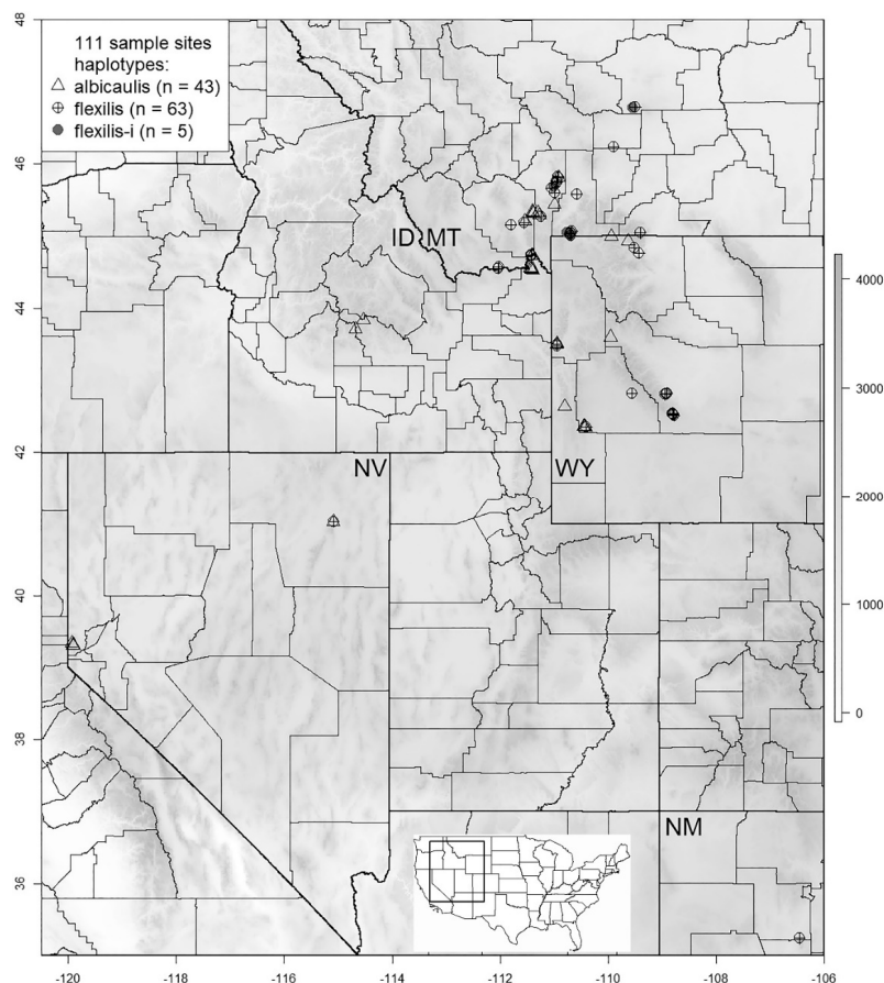
Figure 4. Geographic distribution in Idaho (ID), Montana (MT), Nevada (NV), New Mexico (NM), and Wyoming (WY) of the 111 sites where we sampled trees with attached seed cones. The rectangle on the inset map of the USA provides a larger geographical context of sample sites. Symbols marking each site indicate the sampled psbA-trnH haplotype. The shading represents elevation (m). Overlapping cross-circles and open triangles indicate where limber and whitebark pine are sympatric (e.g., Madison County, Montana; Elko County, Nevada; and Teton County, Wyoming).
