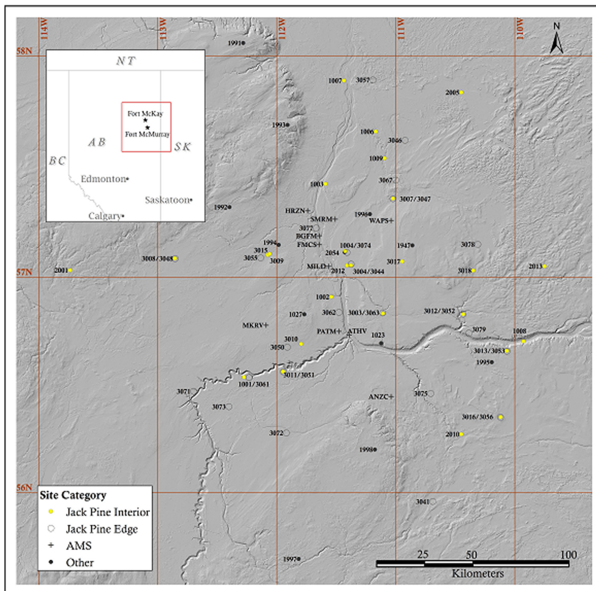
Fig. 1. Locations of monitoring and receptor sites used in this study. TEEM FHM sites have 4-digit ID, community and industrial sites have 4-letter ID.
