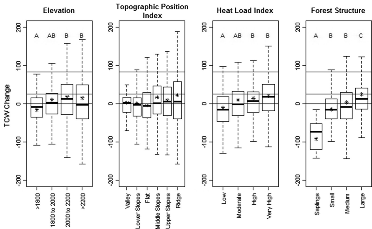
Fig. 7 Boxplots showing the relationship between TCW change and topographic and forest structure variables. TCW change values were taken from a differenced 2011–2016 LandTrendr image
