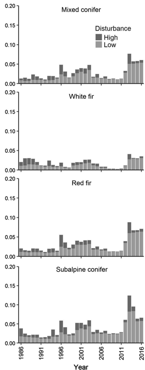
Fig. 4 Proportion of area disturbed for each year of the LandTrendr time series for each forest type. Low decline values were based on a 25-unit or greater decrease in tasseled cap wetness (TCW) between each year, while high decline was based on an 83-unit decrease. Note the elevated levels of disturbance in the red fir and subalpine conifer forest types
