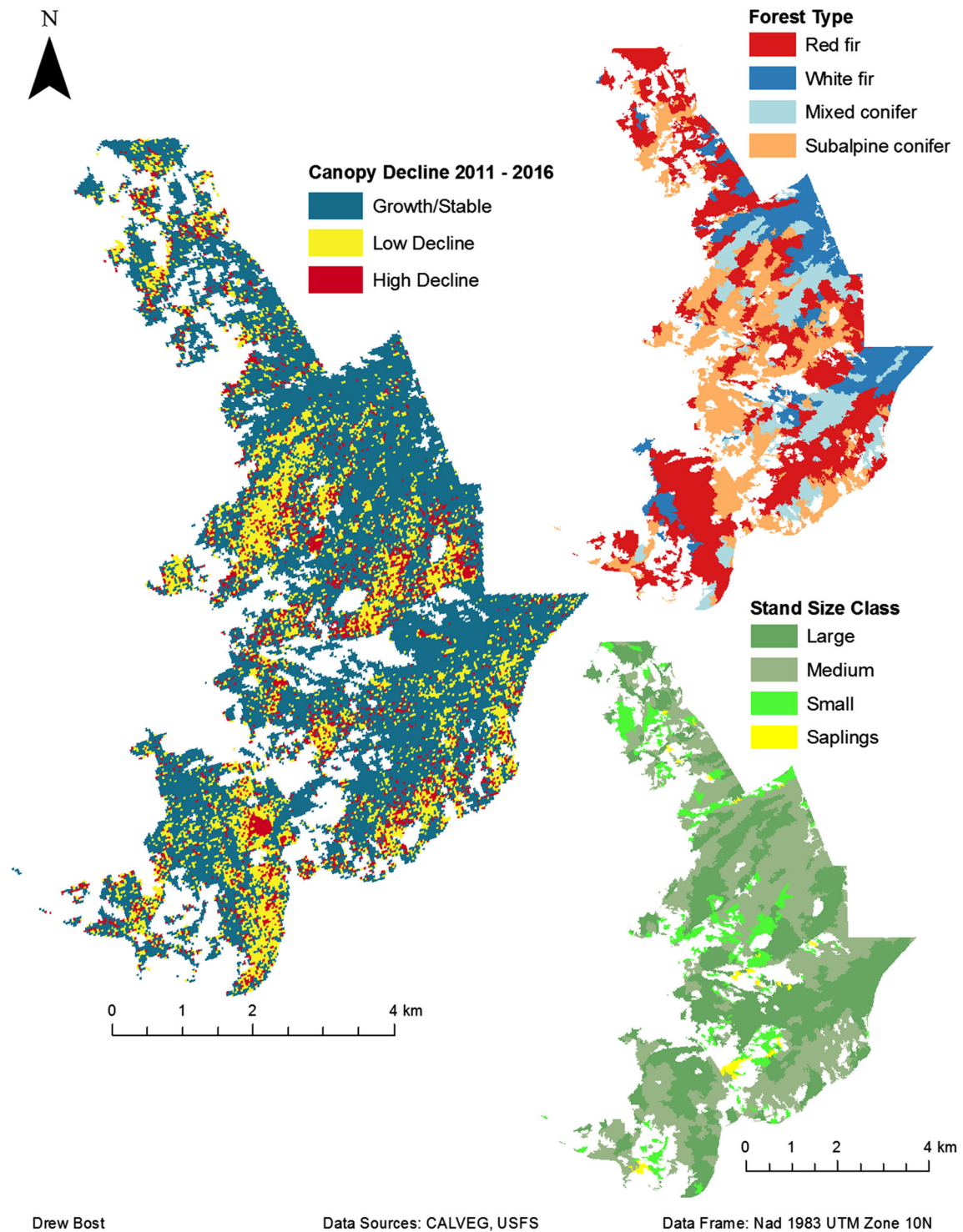
Fig. 5 Map of the Russian Wilderness, CA depicting the change in canopy decline between 2011 and 2016. Upper-right map depicts dominant forest types while lower-right map depicts forest stand size classes. Gaps indicate non-forested areas
