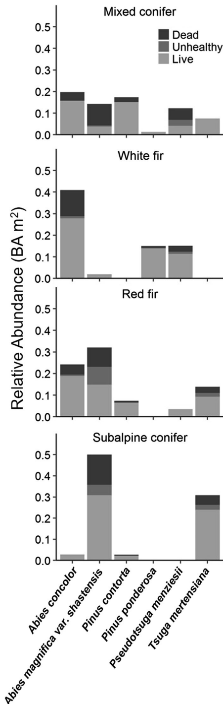
Fig. 2 Comparison of basal area (BA) among four forest types in the Russian Wilderness, CA based on 116 field-measured plots. Forest types were derived from combined CALVEG forest classes (see text for details). Plots were taken in summer of 2015
