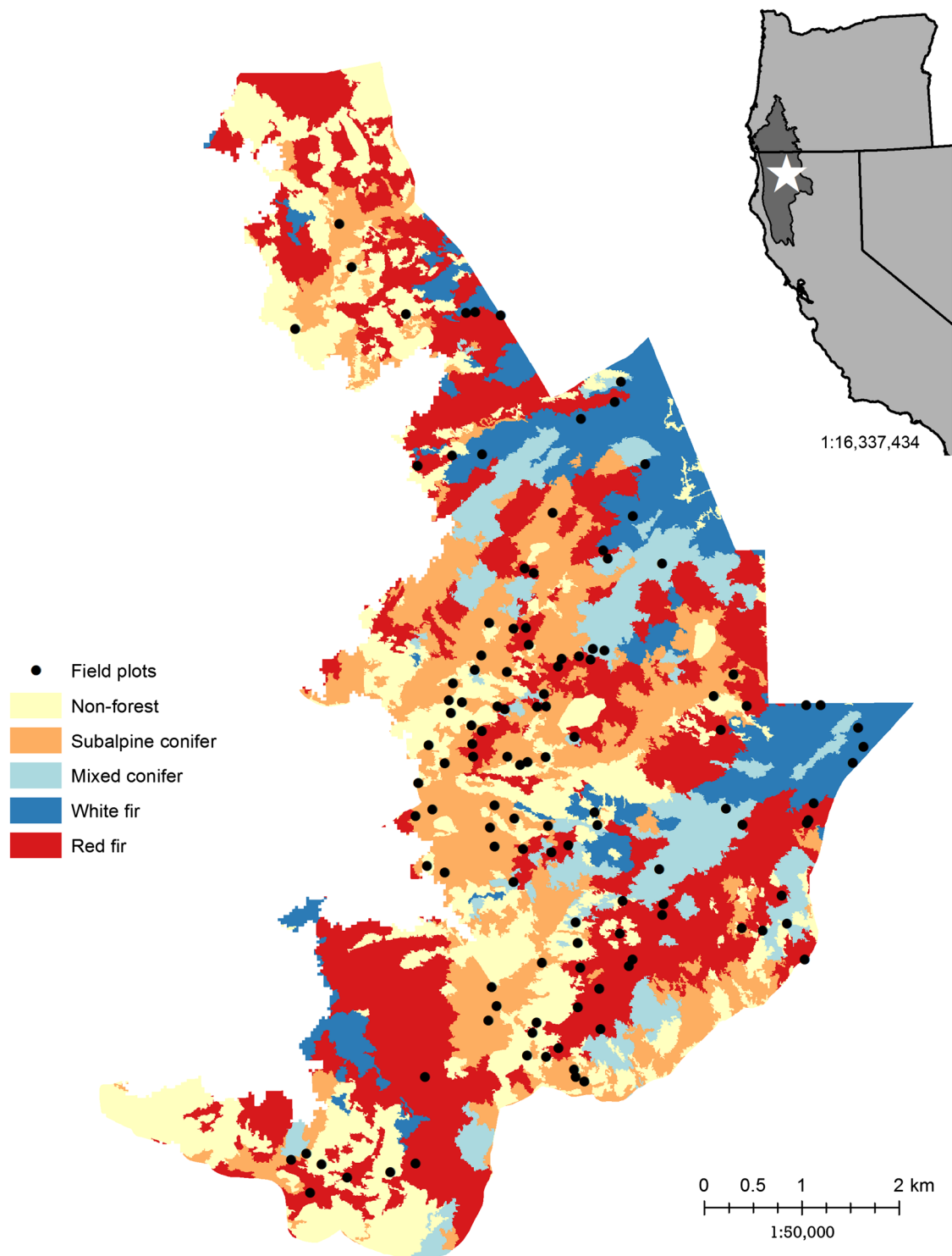
Fig. 1 Map of the study area in the Russian Wilderness, CA, located within the east-central extent of the Klamath Region (shown on locator map). Plot data was collected in summer of 2015. Forest type data is from the 2014 CALVEG dataset (Parker and Matyas 1979)
