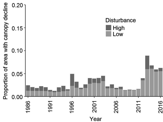
Fig. 3 Proportion of area experiencing canopy decline for each year of the LandTrendr time series for combined forest types. Low decline values were based on a 25-unit or greater decrease in tasseled cap wetness (TCW) between each year, while high decline was based on an 83-unit decrease
