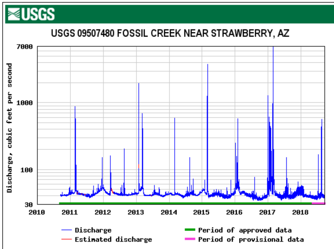
Figure 2-2. Instantaneous discharge in cubic feet per second at USGS Gage 09507480 at Fossil Creek Bridge
