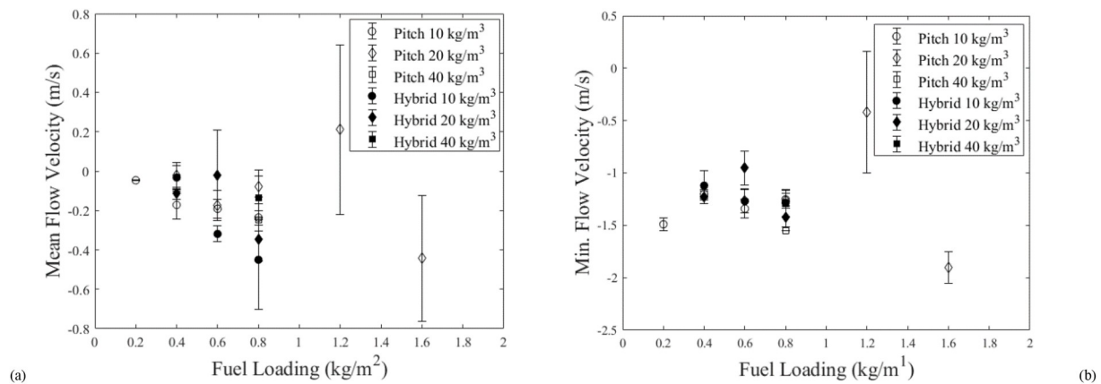
Fig. 8. Mean and minimum in-bed flow velocity towards the approaching flame front (50 mm–10 mm prior to flame arrival), in beds of different fuel loading and bulk density for beds of Pitch Pine and Pitch-Loblolly Pine hybrid respectively.
