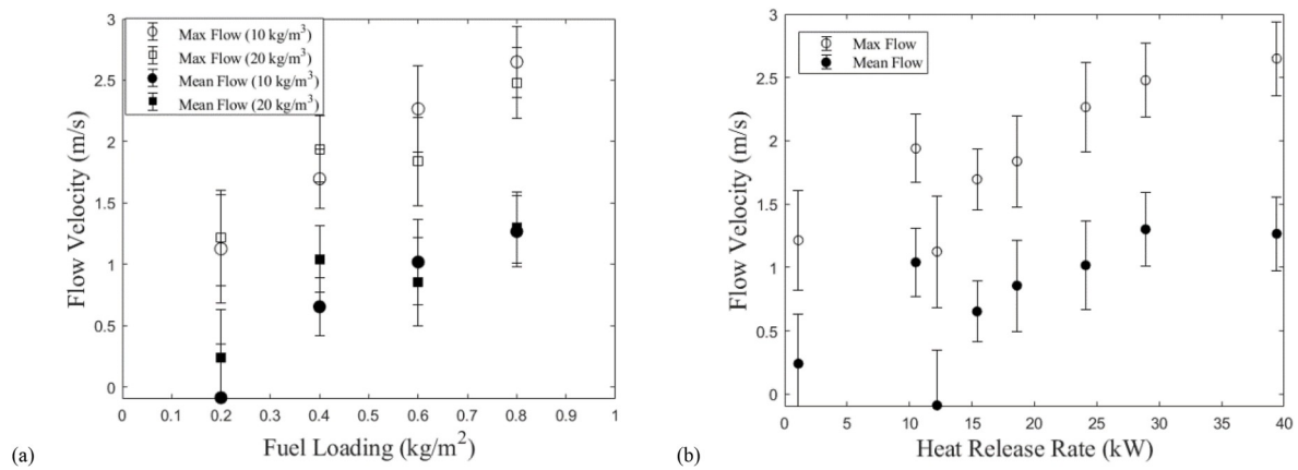
Fig. 7. Comparison of (a) Fuel Loading, (b) Heat Release Rate, with mean and max. buoyant flow velocity at a height of 1.2 m above Pitch Pine fuel beds, in the 10 s after flame arrival.
