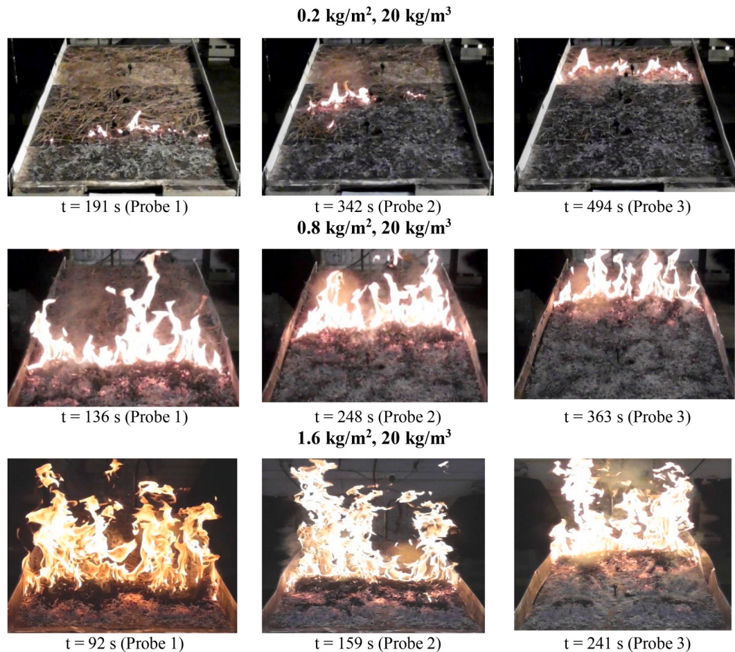
Fig. 2. Composite of frames from downward-looking video footage of flame spread experiments displaying variation in flame and front shape between Pitch Pine fuel beds of (Top) 0.2 kg/m 2 , 20 kg/m 3 (Middle) 0.8 kg/m 2 , 20 kg/m 3 (Bottom) 1.6 kg/m 2 , 20 kg/m 3 .
