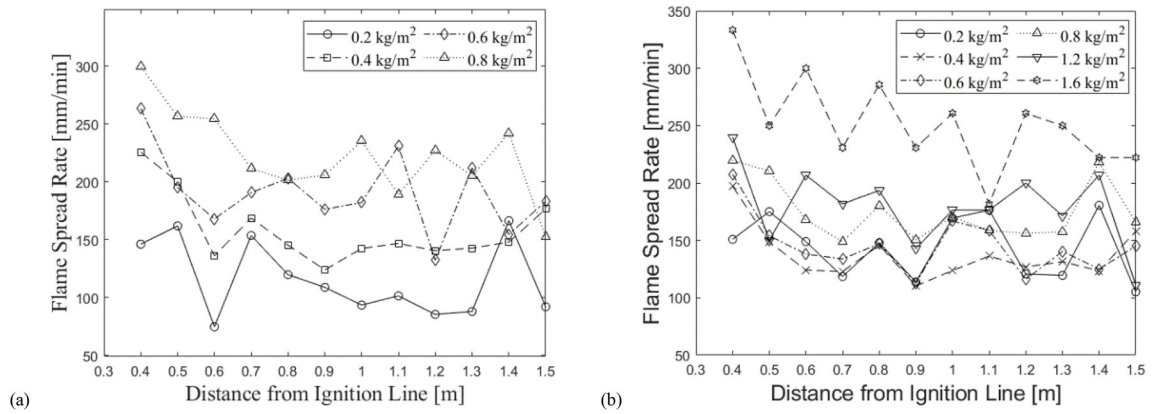
Fig. 4. Flame Spread Rate as a function of distance (based on video analysis) for Pitch Pine fuel beds of different fuel loadings at (a) 10 \text{ kg/m}^3 bulk density, and (b) 20 \text{ kg/m}^3 bulk density.
