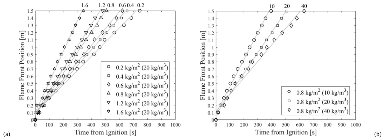
Fig. 3. Flame front position versus time from ignition for Pitch Pine beds of (a) 20 \text{ kg/m}^3 bulk density, and (b) 0.8 \text{ kg/m}^2 fuel loading (avg. of all experiments at each condition).
