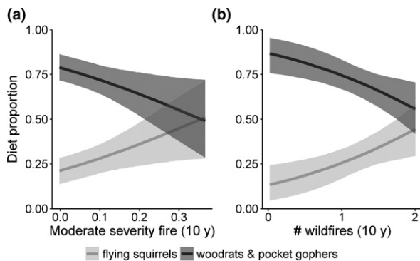
Figure 2. Relationships between California Spotted Owl diet and (a) the proportion of moderate-severity fire within owl territories in the last 10 years; and (b) the number of wildfires within owl territories in the last 10 years.
