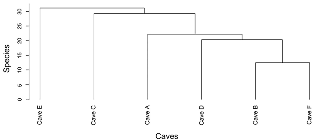
Fig. 2. Cluster analysis of vascular plants and bryophytes in six karst caves. Caves A, B, C, and D are located in Dixiahe, and caves E and F are located in Shangbaichang. Caves A, B, and C were developed for tourism in 1988. Cave B was closed for tourists and kept natural after 2000. Cave C was protected from disturbance after 2010. Cave F had a long history of high disturbance associated with the feeding of poultry on plants. Caves D and E were relatively undisturbed.
