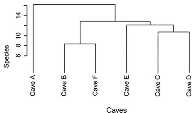
Fig. 4. The cluster analysis of vascular plants in six karst caves. See the Fig. 2 legend for descriptions of the six caves.
