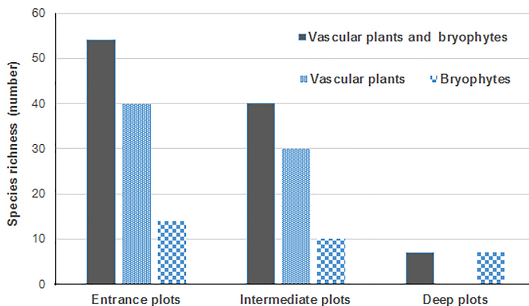
Fig. 1. Species richness per plot of vascular plants and bryophytes together, of vascular plants alone, and of bryophytes alone in the cave entrance, intermediate, and deep plots.
