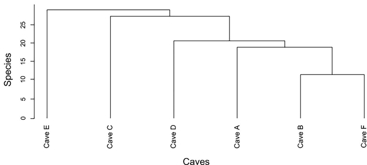
Fig. 3. The cluster analysis of bryophytes in six karst caves. See the Fig. 2 legend for descriptions of the six caves.
