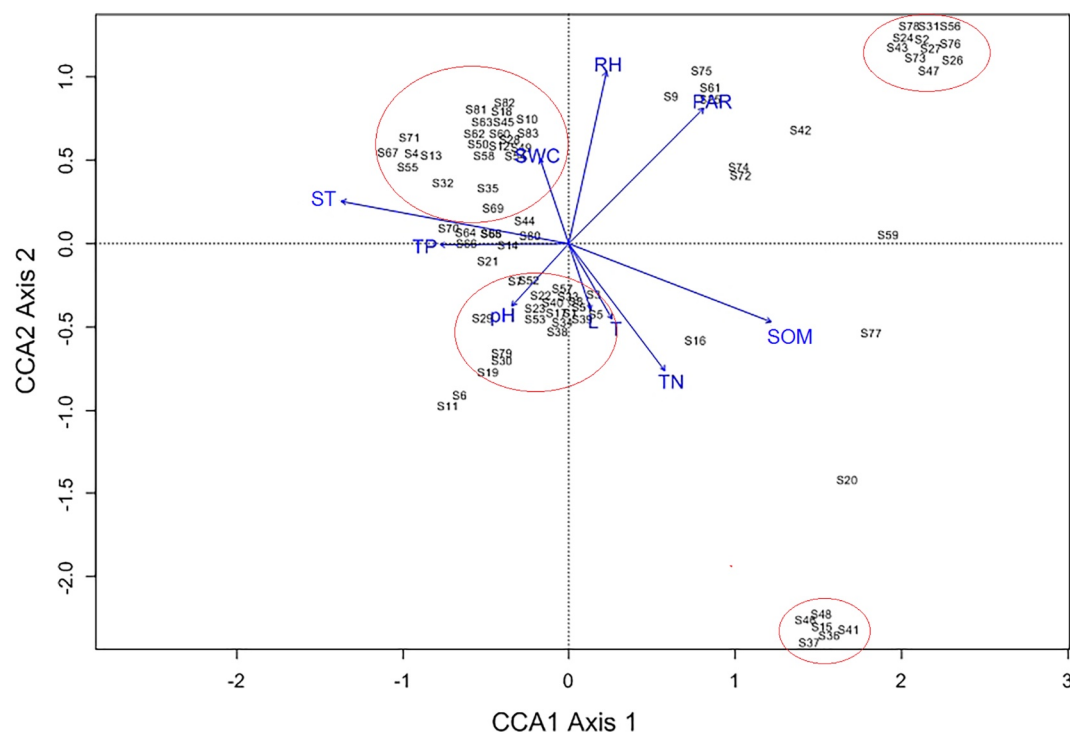
Fig. 5. Canonical correspondence analysis of the vegetation and 10 environmental factors in 18 plots in six karst caves. TN, total nitrogen content; TP, total phosphorus content; SOM, soil organic matter; pH, pH value; SWC, soil water content; ST, soil thickness; PAR, photosynthetically active radiation; RH, relative humidity; T, air temperature; L, light transmittance. The species codes are explained in Supplementary Table 1 (S1–S63) and Supplementary Table 2 (S64–S83).
