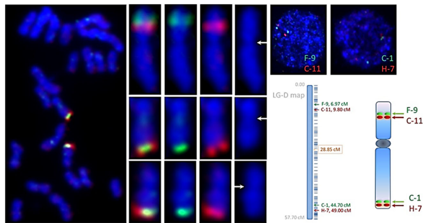
Fig. 2 Example of multiple-probe BAC-FISH mapping result for assignment of C. mollissima chromosomes linkage group D to its corresponding linkage group. FISH was conducted with four selected BAC clones (two from opposite ends of each arm) on Chinese chestnut chromosome spreads: (a) a complete root tip metaphase chromosome spread showed two BAC-FISH signals (BAC C1, 44.70 cM, green signal; BAC H7, 49.00 cM, red signal) located on the long arm of the LG_D homologs (chromosomes); (b1–4) an enlarged FISH image of a pro-metaphase chromosome with BAC clones (BAC F9, 6.97 cM, green signal; BAC C11, 9.80 cM, red signal) located on the short arm of the same chromosome; b1, a superimposed image from DAPI (blue
