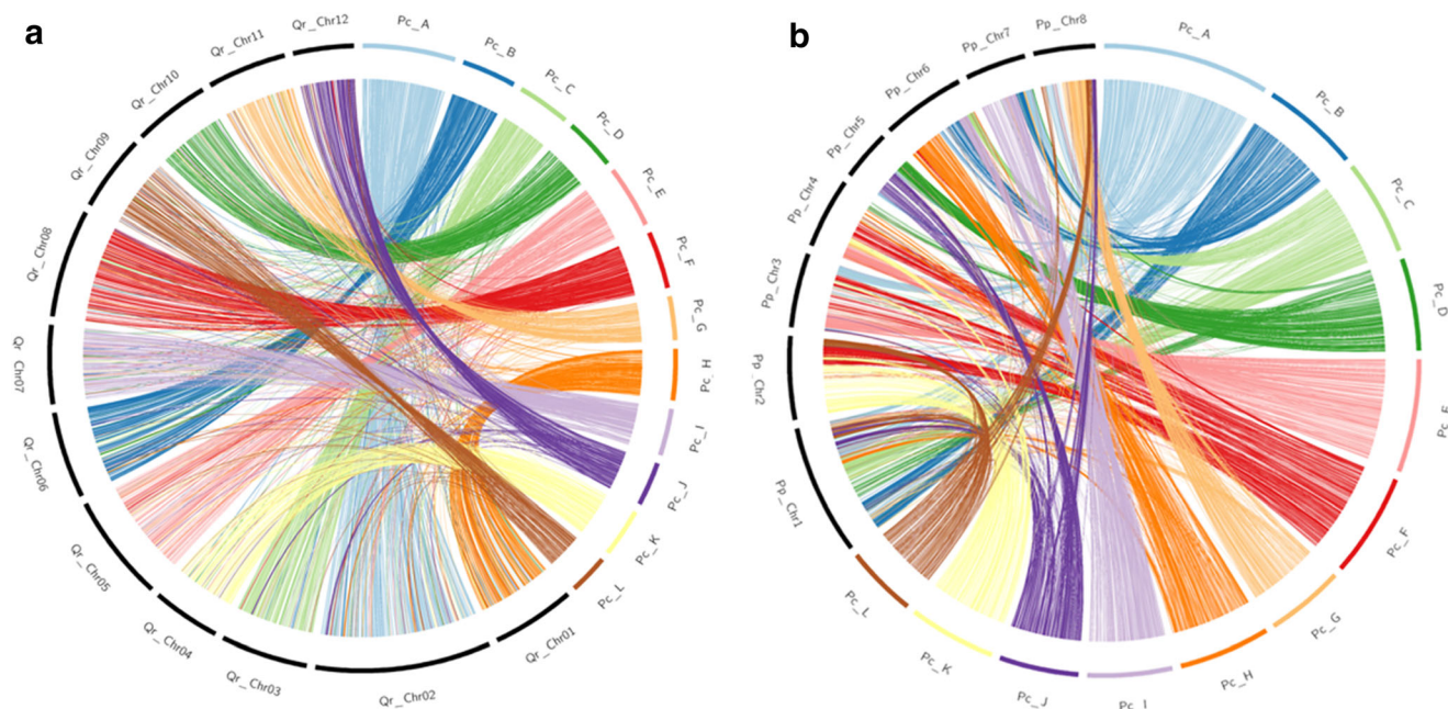
Fig. 3 Circos plot of alignments of orthologous genes in C. mollissima chromosomes (Pc_A-L) vs Q. robur chromosomes (Qr_1–12) (a) and Prunus persica chromosomes (Pp_1–8) (b). Alignment of the genomes
