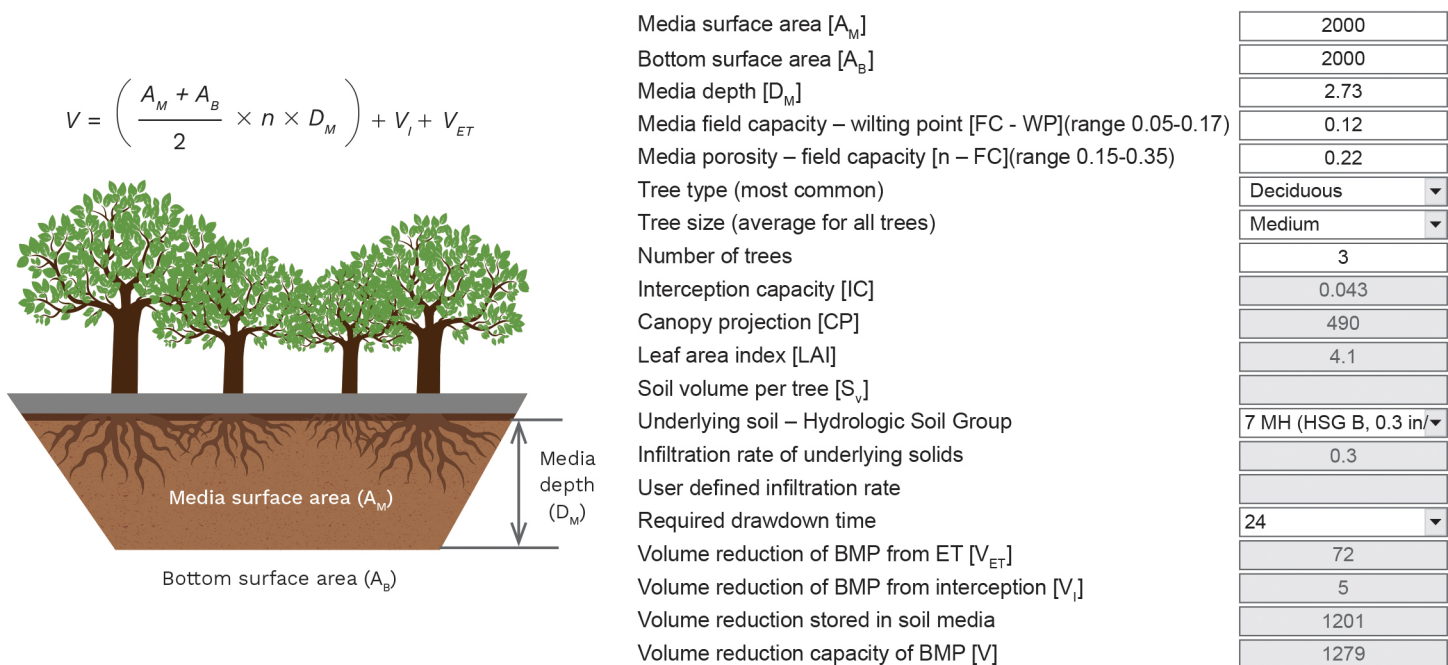
Figure 2. One of the Minimal Impact Design Standards (MIDS) Calculator Tree Trench Best Management Practice (BMP) input screens showing tree and soil inputs (white boxes) and model outputs (gray).
