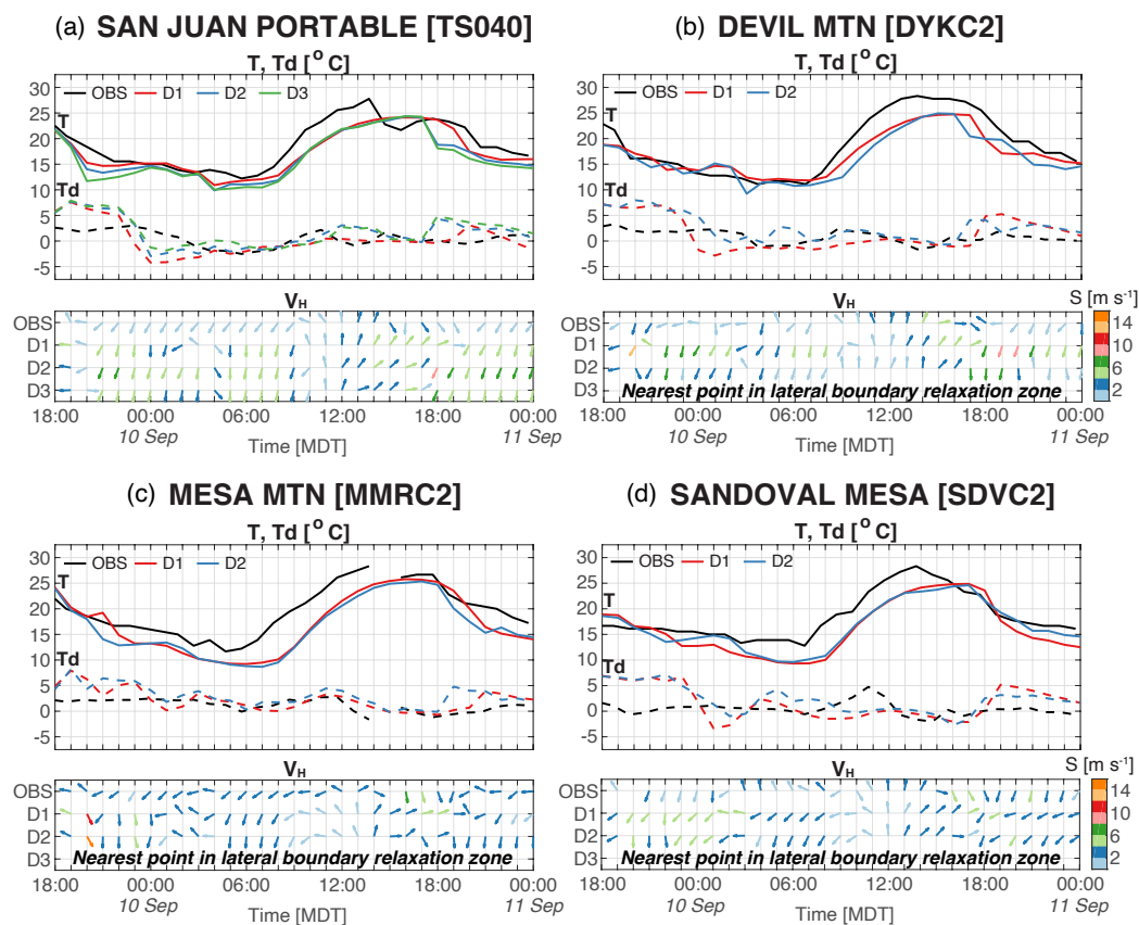
Figure 5. Time series of observed and simulated temperature (T), dewpoint (Td), and horizontal wind vectors ( V_H ; color scale for wind speed (S) included to right of figure), at four RAWS sites: (a) San Juan Portable (TS040), (b) Devil Mtn (DYKC2), (c) Mesa Mtn (MMRC2), and (d) Sandoval Mesa (SDVC2). Note that domain D3 is omitted from panels (b–d) because nearest grid points to RAWS sites are in lateral boundary relaxation zone. Temperature and dewpoint are measured at 2 m above ground level (AGL) at all four RAWS stations, and wind speed is measured at either 2 m AGL (TS040) or 6.1 m AGL (DYKC2, MMRC2, and SDVC2); all simulated variables are valid at the lowest grid level (D1: 25 m; D2: 12.5 m; D3: 5 m AGL). See Figure 1c for location of RAWS sites.
