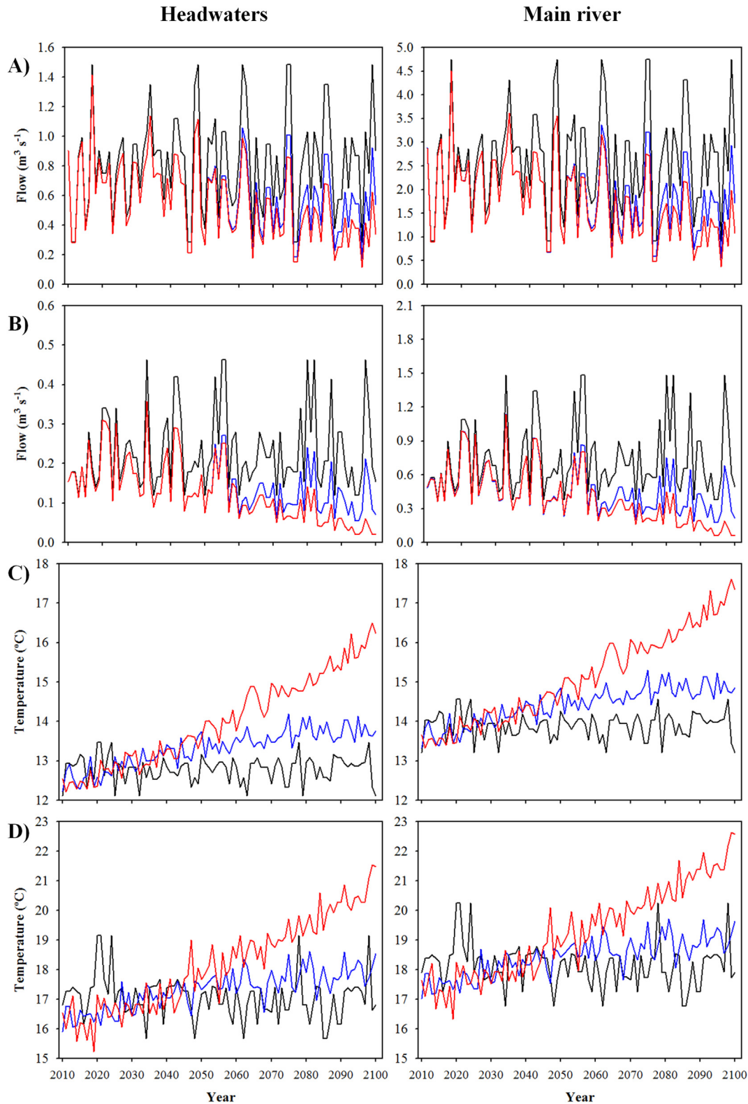
Fig. 1. Time series of mean daily flow (row A) and seven-day minimum daily flow (row B) during the trout growing season (March to October) under the no-flow-change (baseline, RCPs 4.5 and 8.5; black line), RCP4.5 + Flow change (blue line) and RCP8.5 + Flow change (red line) simulation scenarios. Time series of mean daily temperature (row C) and seven-day maximum daily temperature (row D) during the trout growing season under the baseline (black line), RCP4.5 (and RCP4.5 + Flow change; blue line) and RCP8.5 (and RCP8.5 + Flow change; red line) scenarios. (For interpretation of the references to colour in this figure legend, the reader is referred to the web version of this article.)
