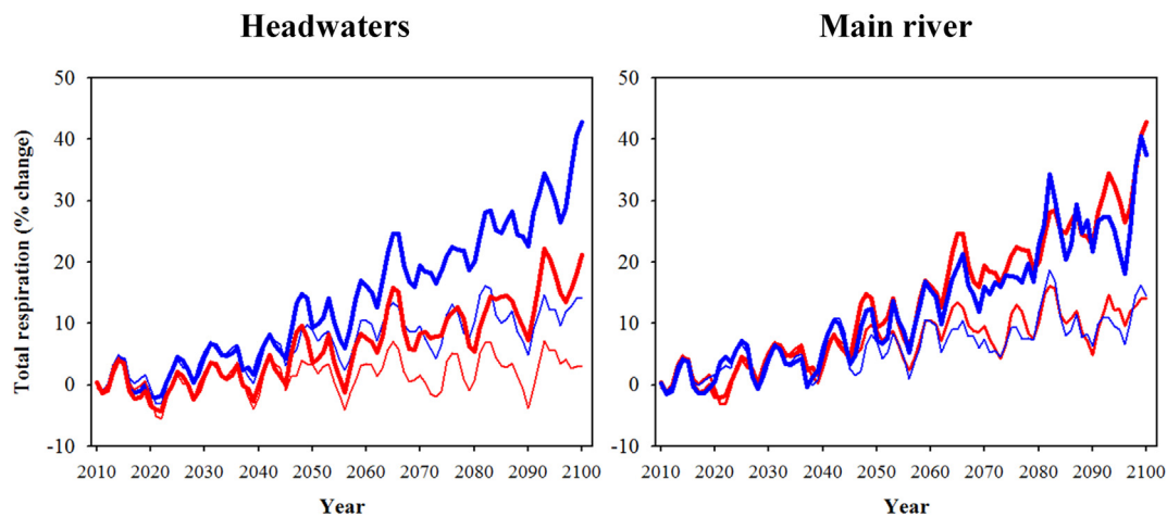
Fig. 3. Change over time in total respiration costs under the RCP4.5 (blue thin line), RCP8.5 (blue thick line), RCP4.5 + Flow change (red thin line) and RCP8.5 + Flow change (red thick line) scenarios. Changes in respiration costs are expressed as the percentage change: [(\text{value environmental change scenario} - \text{value baseline}) / \text{value baseline}] \times 100 . Time series were smoothed using the three-year moving average for representation purposes. (For interpretation of the references to colour in this figure legend, the reader is referred to the web version of this article.)
