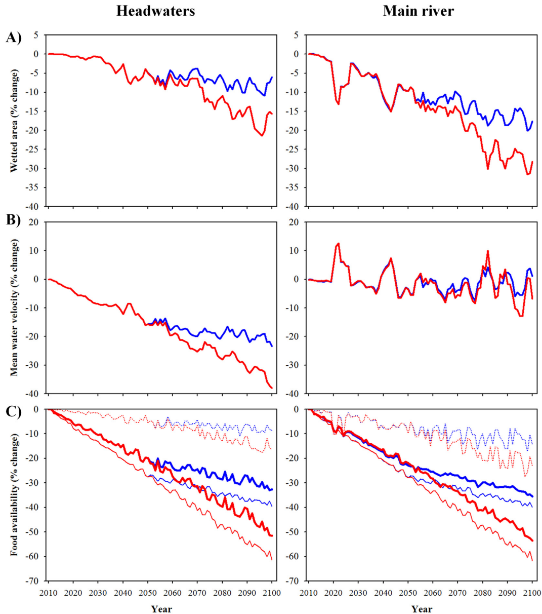
Fig. 2. Change over time in the physical habitat and food availability variables under scenarios of flow change relative to the baseline scenario in two river types (headwaters vs. main river). The figure shows wetted area (row A) and mean water velocity (row B) changes under RCP4.5 + Flow change (blue line) and RCP8.5 + Flow change (red line) scenarios. Row C shows the availability of drift (thin continuous line), benthic (dotted line) and total food (thick continuous line) changes under RCP4.5 + Flow change (blue colour) and RCP8.5 + Flow change (red colour) scenarios. Changes in the variables are expressed as the percentage change: [(\text{value flow change scenario} - \text{value baseline}) / \text{value baseline}] \times 100 . Time series were smoothed using the three-year moving average for representation purposes. (For interpretation of the references to colour in this figure legend, the reader is referred to the web version of this article.)
