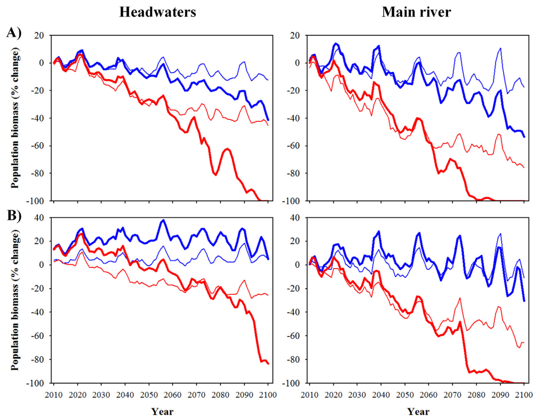
Fig. 4. Change over time in population biomass under scenarios of environmental change without (A) and with simulated increase in food production (B) relative to the baseline scenario in two river types (headwaters vs. main river). Biomass change was simulated under the RCP4.5 (blue thin line), RCP8.5 (blue thick line), RCP4.5 + Flow change (red thin line) and RCP8.5 + Flow change (red thick line) scenarios. Changes in biomass are expressed as the percentage change: [(\text{value environmental change scenario} - \text{value baseline}) / \text{value baseline}] \times 100 . Time series were smoothed using the three-year moving average for representation purposes. (For interpretation of the references to colour in this figure legend, the reader is referred to the web version of this article.)
