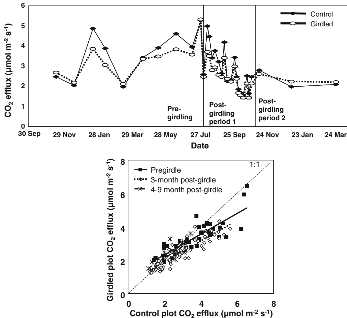
Fig. 3 Soil \text{CO}_2 efflux ( upper ) dropped by 15.8% in the first 3 months in response to girdling ( p = 0.01 ), but the 6.6% reduction that occurred from 4 to 9 months post-girdling was not significant ( p > 0.5 ). The slopes of the relationships between control and
