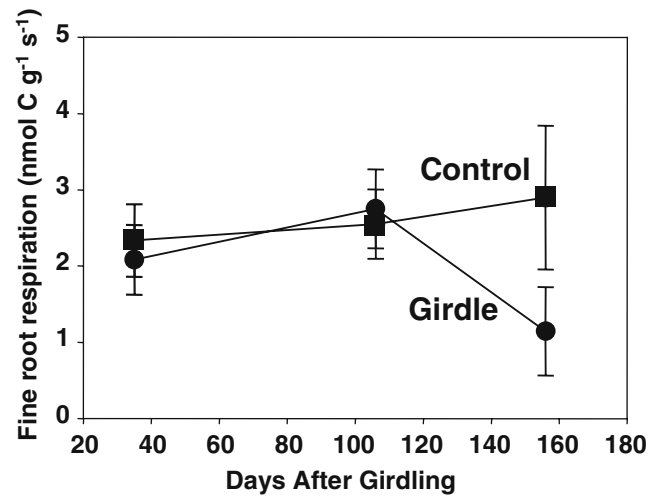
Fig. 6 Root respiration did not differ between the control and girdled plots after girdling for Experiment 1. Bars are standard errors of the means for four replicate plots
