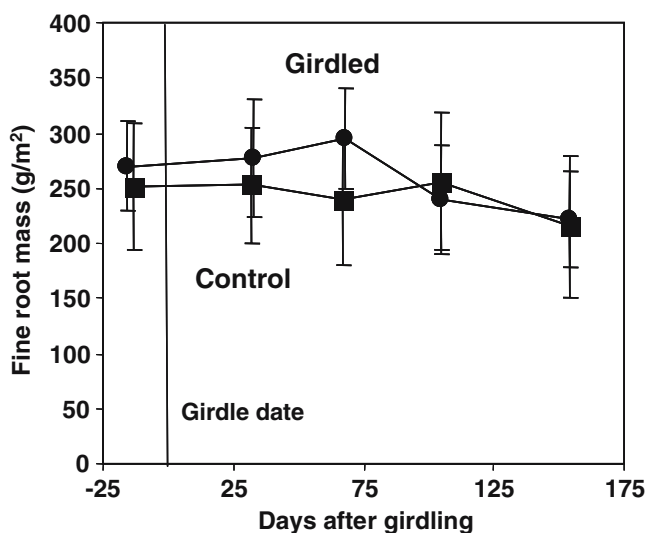
Fig. 5 Biomass of live fine roots in Experiment 1 did not respond to girdling for more than 150 days after girdling. Bars are standard errors of the means for four replicate plots
