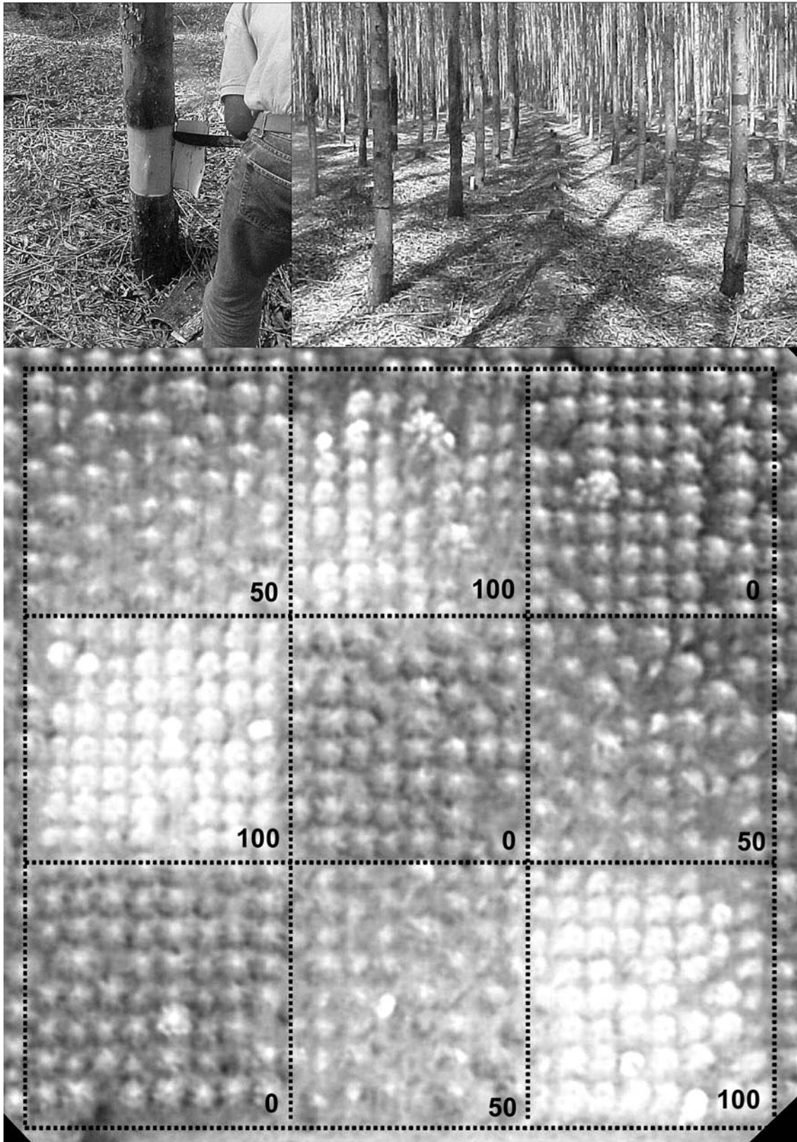
Fig. 1 Top left Photo of tree-girdling treatment plot, top right Experiment 1 immediately after girdling; grid photograph aerial view of Experiment 2 11 months after girdling showing light-
