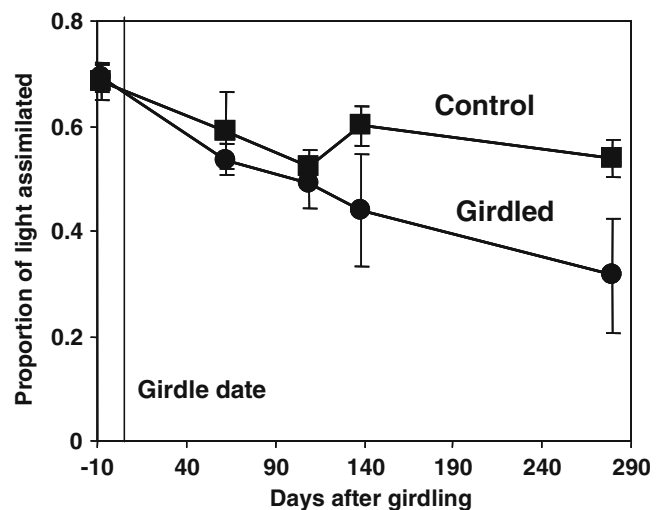
Fig. 2 Light interception in Experiment 1 remained similar between control and girdled plots for more than 100 days after girdling. Bars are standard errors of the means from four plots/treatment
