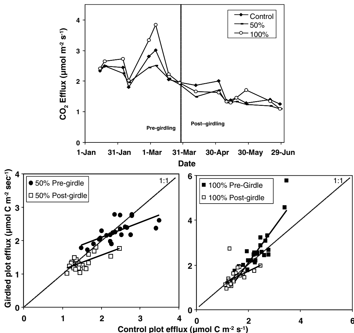
Fig. 4 Girdling of all trees in Experiment 2 reduced soil CO 2 efflux (left) by 24%, and girdling one half of the trees reduced it by 20% ( p=0.02 for girdling effect; for the difference between 50 and 100% girdling, p=0.22 ). The slopes of the relationships between the
