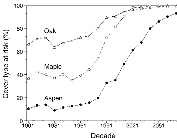
FIG. 5. Predicted change in risk (percentage of cover type with p \geq 0.5 of gypsy moth establishment) to aspen (solid circles), oaks (triangles), and maples (open circles) in Utah, based on normals from the 1901–1930 to 2071–2100 periods.
