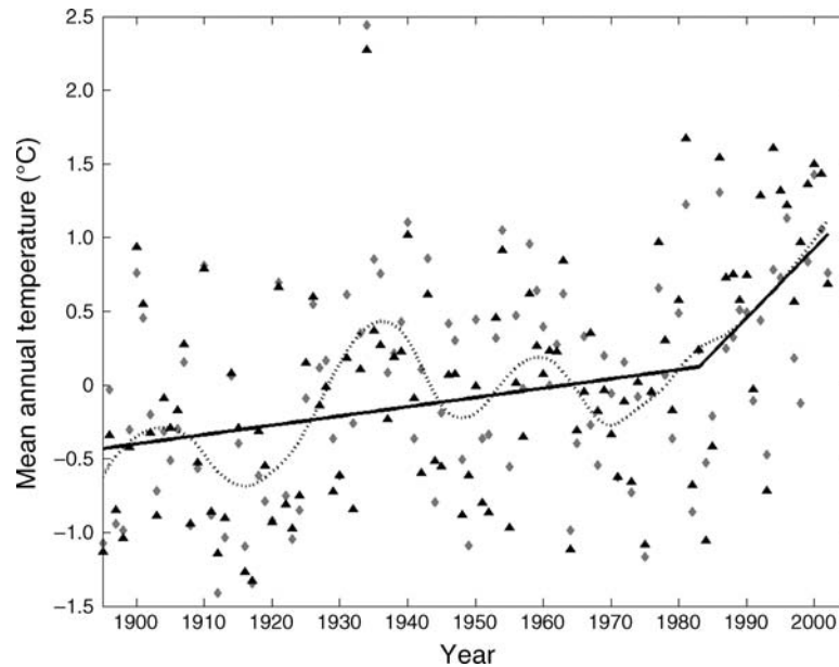
FIG. 2. Deviation (temperature, °C) from mean annual temperature for Utah NCDC Division 4 (diamonds) and Division 5 (triangles), with fitted Lowess-estimated trend line (dotted line), and piecewise linear model (solid line; Eq. 5).
