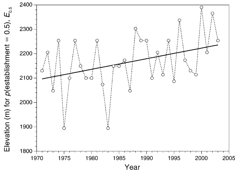
FIG. 4. Change through time of E_{0.5} , the elevation at which the probability of gypsy moth establishment ( p ) crosses 0.5, in the middle of the simulation transect across Utah ( 39^\circ N, 111^\circ 30' W), based on simulations using NCDC Summary of the Day records between 1971 and 2003. Open circles indicate results of the annual logistic regression model (Eq. 6); the solid line indicates results of the global logistic regression model (Eq. 7).
