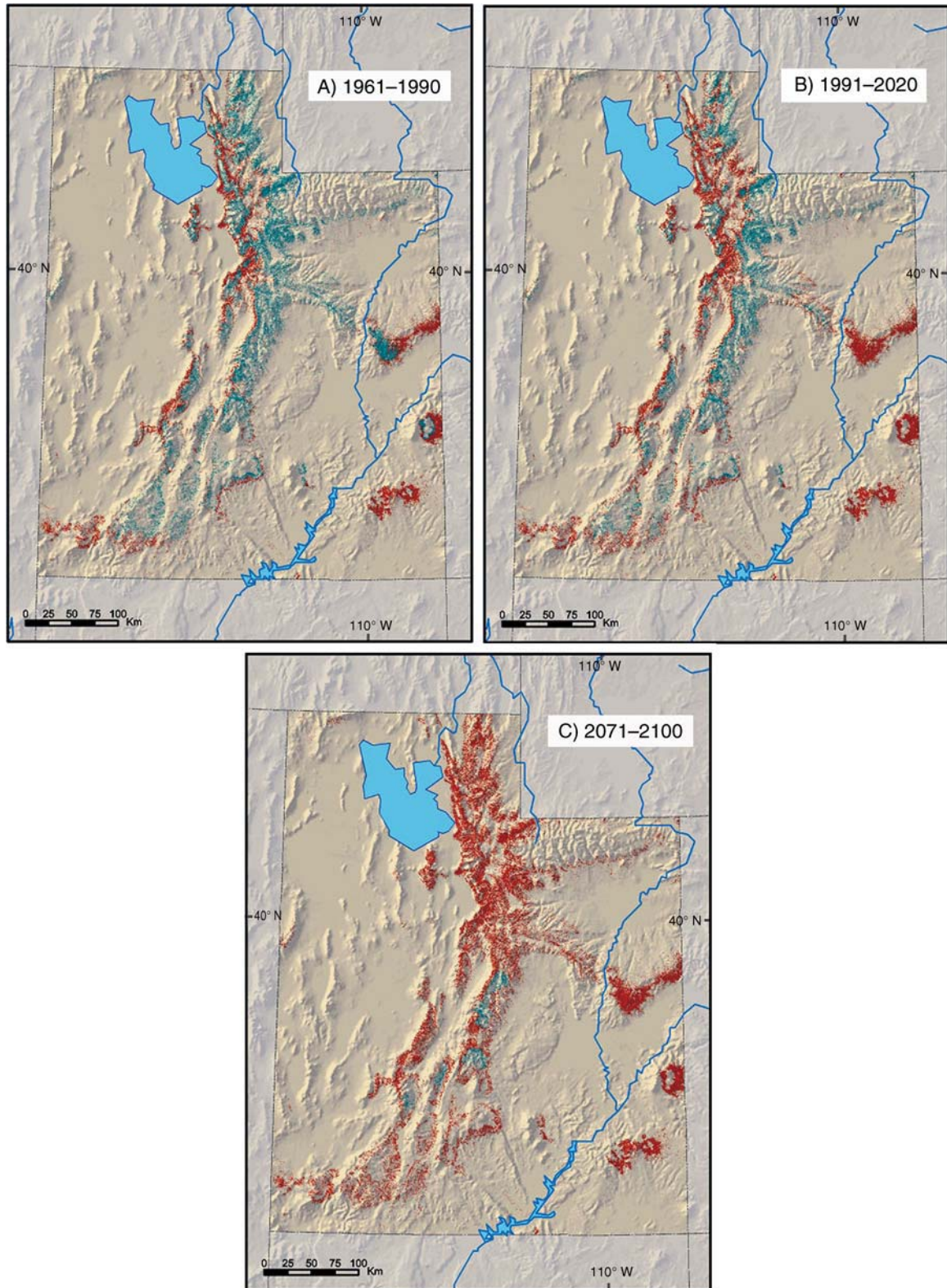
FIG. 6. Hazard maps ( p \leq 0.5 , green; p > 0.5 , red) for the three primary host plants (aspen, oaks, and maples) in Utah, as effected by climate change: (A) 1961–1990 normals, (B) 1991–2020 normals, and (C) 2071–2100 normals (VEMAP gridded database).
