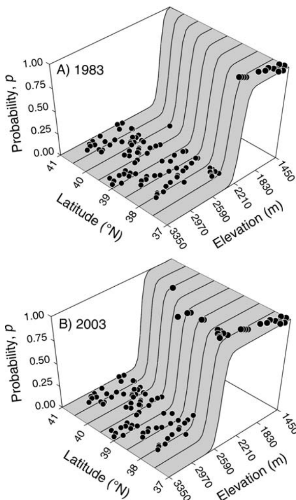
FIG. 3. Logistic relationship between probability of gypsy moth establishment ( p ), latitude, and elevation (based on NCDC Summary of the Day records along a north–south transect across Utah in (A) 1983 and (B) 2003. Individual climatic suitability flag values ( F ) appear as solid circles. Logistic regression surfaces are generated by Eq. 6.
