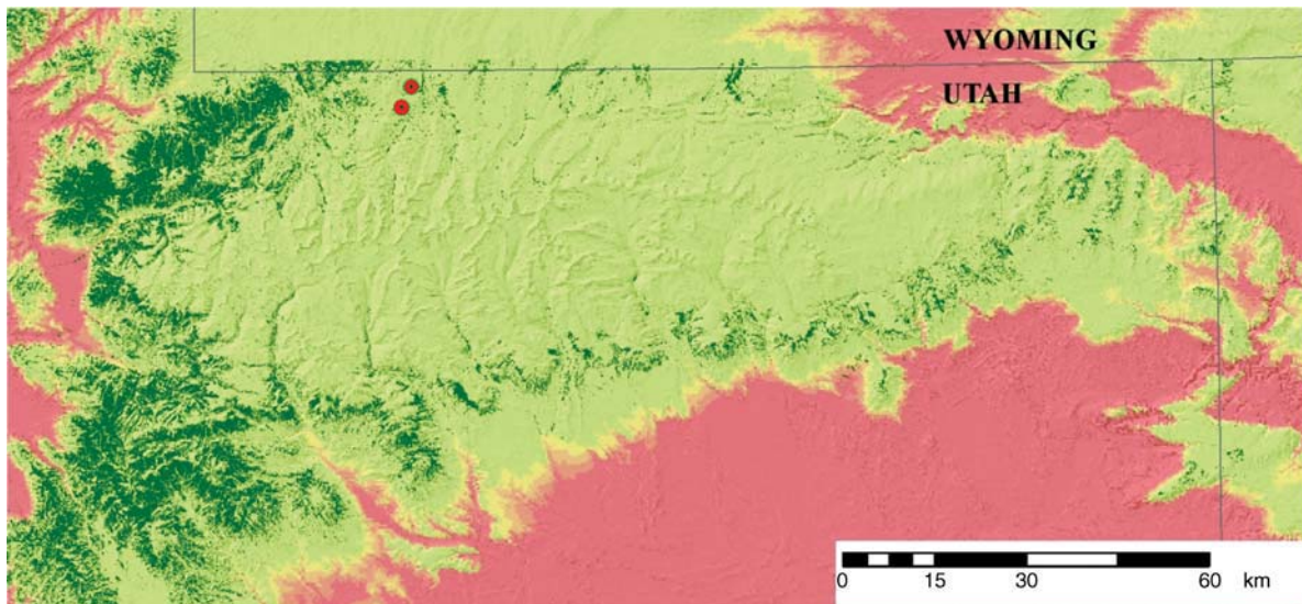
FIG. 7. Hazard rating for the Uinta Mountains of northern Utah is shown, ranging from green ( p = 0.0\text{--}0.2 ) to red ( p = 0.9\text{--}1.0 ), based on climate normals for 1981–2010. The locations for the 2003 trap recoveries are shown as red target-circles. Aspen distribution (Utah GAP data) is indicated by dark green.
