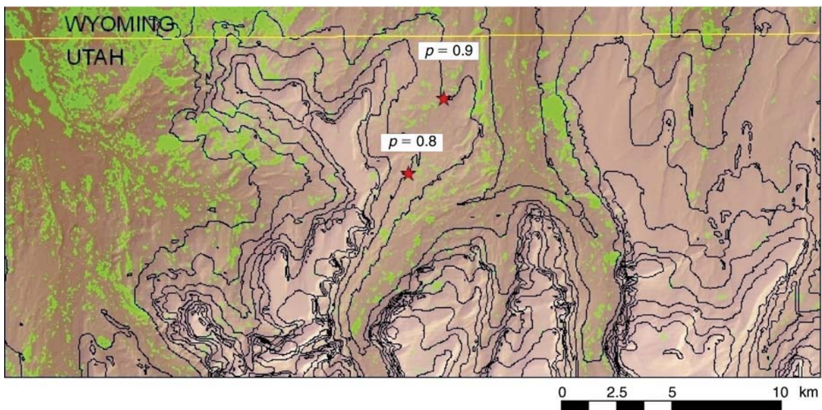
FIG. 8. Gypsy moth hazard in the Lyman Lakes quadrangle, with climate normals projected for the period 2071–2100. Male moth trap recovery locations are indicated by the red stars. Contour lines are indicated in black, with one trap lying on the p = 0.9 line and the other on the p = 0.8 line, indicating that by 2100 the benign introduction of 2003 would be predicted to be a serious threat. Aspen distribution (Utah GAP data) is indicated by green.
