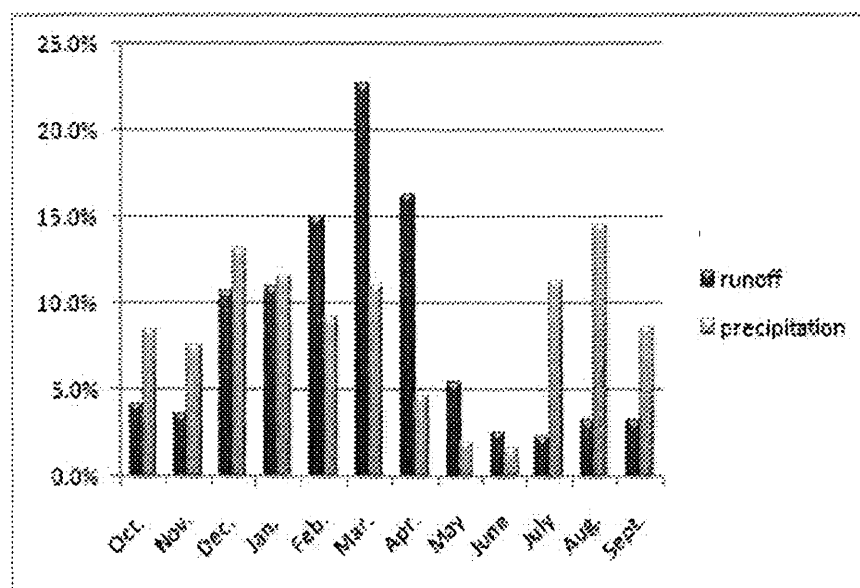
Figure 2. Comparison of average monthly precipitation and runoff at Workman Creek. Data are presented as monthly percents of total of the annual precipitation and runoff to illustrate the trend therein. Due to the location of the precipitation gauge at a lower elevation, the actual quantities of precipitation are not included. Runoff in winter months is related more to snowmelt than to precipitation received during that month.
