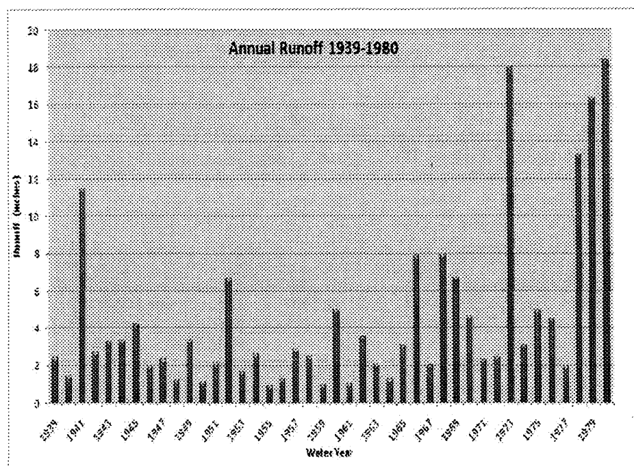
Figure 1. Total yearly runoff at Main Dam of Workman Creek from 1939-1980.
