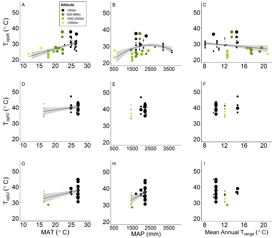
Figure 2.2 The optimum temperature of net photosynthesis and biochemical responses to three primary climate variables. The optimum temperature of net photosynthesis ( T_{opt} ) response to A) mean annual temperature (MAT), B) mean annual precipitation (MAP), and C) mean annual temperature range ( T_{range} ). The optimum temperature of net photosynthesis ( T_{optV} ) response to D) mean annual temperature (MAT), E) mean annual precipitation (MAP), and F) mean annual temperature range ( T_{range} ). The optimum temperature of net photosynthesis ( T_{optU} ) response to G) mean annual temperature (MAT), H) mean annual precipitation (MAP), and I) mean annual temperature range
