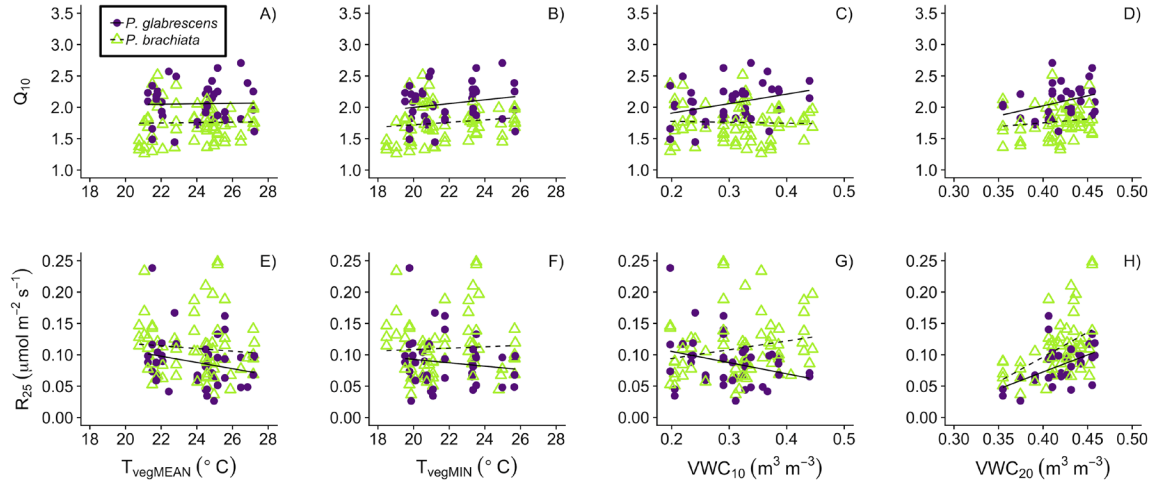
Fig. 3.6 Respiratory parameter responses to mean ( T_{vegMEAN} ), min ( T_{vegMIN} ) daily vegetation temperature, soil moisture at 10-20 cm ( VWC_{10} ), and 20-30 cm depth ( VWC_{20} ). A) The increase in respiration for every 10 °C ( Q_{10} ) response to T_{vegMEAN} of P. brachiata (green triangles) and P. glabrescens (purple circles), B) Q_{10} response to T_{vegMIN} , C) Q_{10} response to VWC_{10} , D) Q_{10} response to VWC_{20} , E) the rate of respiration at 25 °C ( R_{25} ) response to T_{vegMEAN} , F) R_{25} response to T_{vegMIN} , G) R_{25} response to VWC_{10} , and H) R_{25} response to VWC_{20} . Fit lines (solid - P. glabrescens ; dashed – P. brachiata ) indicated individual species fit when there is an overall significant environmental response, species difference, or an interaction between the environmental variable and species (Table B4).
