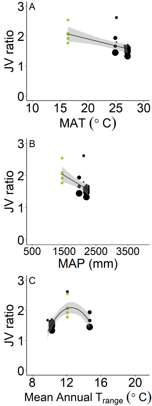
Figure 2.5 The ratio between rate of J_{max} and V_{cmax} responses to three primary climate variables. The ratio between the rate of J_{max} at 25 °C and V_{cmax} at 25 °C ( JV ) responses to A) mean annual temperature (MAT), B) mean annual precipitation (MAP), and C) mean
