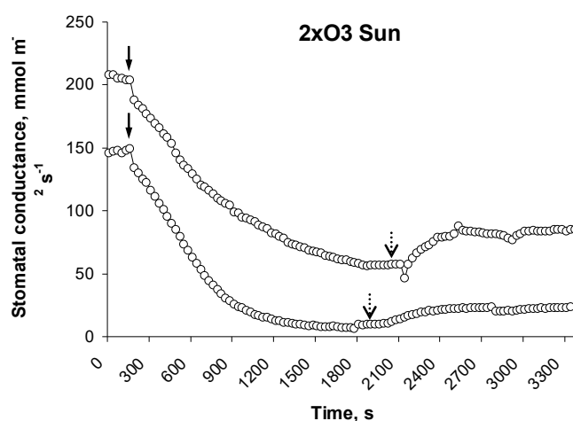
Figure 5. Examples of unresponsive 2xO_3 beech leaves. Stomata closed regularly when the light was off (full arrows) but did not re-open when the light was on (dotted arrows).
