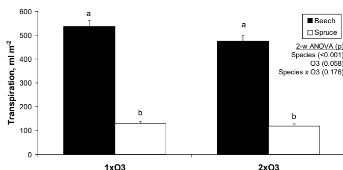
Figure 3. Mean daily total transpiration ( \pm SE) calculated from sap flow measurements in beech and spruce trees. Each bar is the average of 4–5 trees in 31 days (July 2007). The inset shows the levels of significance from a two-way (tree species x O_3 regime) analysis of variance ( n = 31 days).
