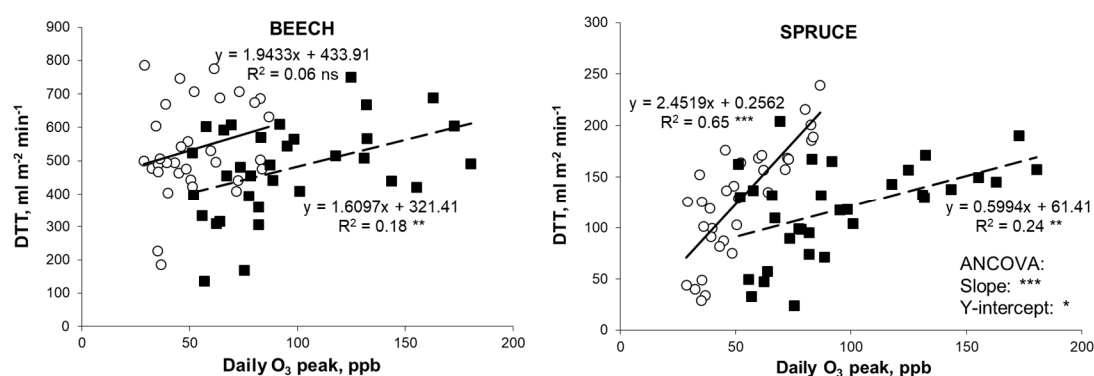
Figure 2. Daily total transpiration (DTT) increased with increasing daily ozone peaks in mature trees of European beech and Norway spruce exposed to ambient (○ solid line) and twice-ambient O 3 regimes (■, dashed line) (July 2007). Each point is the average of 4–5 trees. Asterisks show the significance of the analysis: ***, p < 0.001 ; **, p < 0.01 ; *, p < 0.05 ; ns, p \geq 0.05 .
