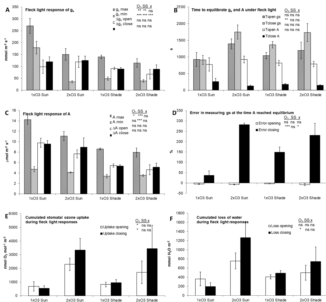
Figure 4. Summary of stomatal and assimilatory responses to fleck light in beech ( \pm SE): (A) max and min stomatal conductance ( g_s ) and span of g_s variation ( \Delta ); (B) time g_s and A reached equilibrium when stomata closed and opened (T); (C) max and min photosynthesis (A) and span of A variation ( \Delta ); (D) error in measuring g_s at the time A reached equilibrium when stomata closed and opened
