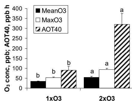
Figure 1. Descriptors of ozone exposure at ambient (1xO 3 ) and twice-ambient ozone (2xO 3 ). Data are daily means of hourly concentrations and accumulated hourly values above 40 ppb (+SE) in July 2007. Different letters show significant differences between the ozone regimes ( t -test or Mann–Whitney U test, p < 0.001 , n = 31 days).
