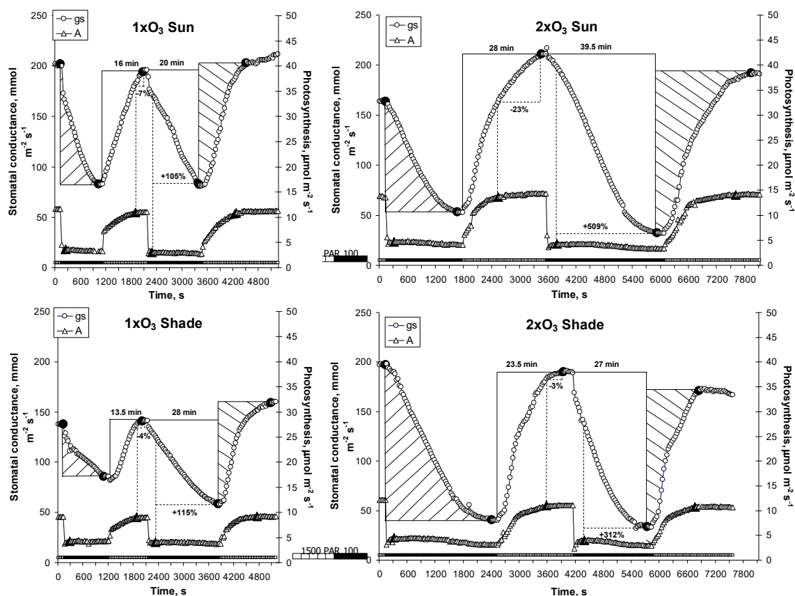
Figure 6. Example of fleck light responses in sun and shade leaves of beech trees. When stomatal conductance (gs) achieved equilibrium, the light intensity was sharply decreased from 1500 to 100 \mu\text{mol m}^{-2} \text{s}^{-1} until equilibrium, and then increased again. The treatment was repeated two times. Full symbols show the time equilibrium was reached, i.e., gs or A (photosynthesis) values were stable in the following two minutes. Full lines show examples of calculation of the time to open and to close stomata (in min). Dotted lines show examples of calculation of the error in recording gs at the time A reached equilibrium (as percent of steady-state gs). Slashed surfaces show examples of cumulated water loss and stomatal O 3 uptake when stomata closed (/) and opened (\).
