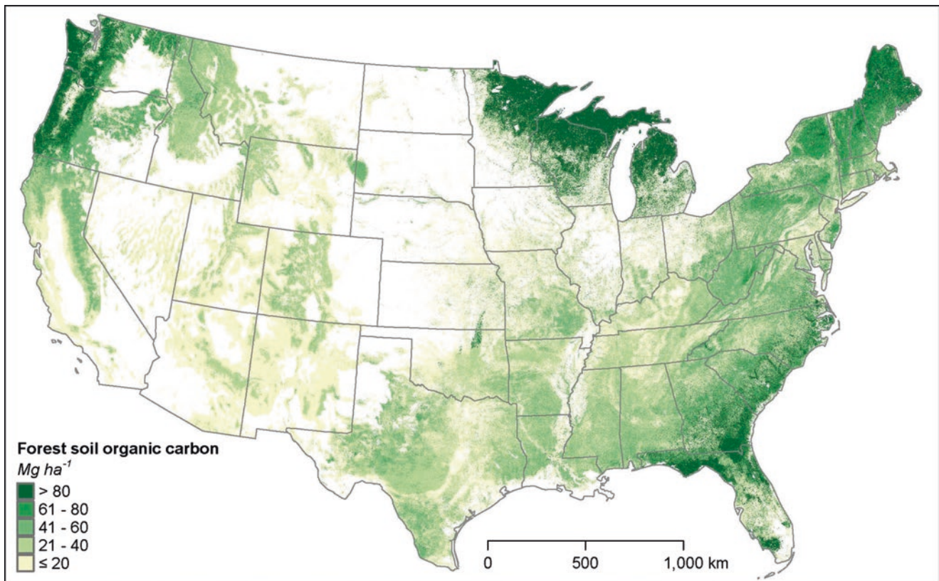
Fig. 9.4 Soil organic C density imputed from USDA Forest Service Forest Inventory and Analysis (FIA) plots in the conterminous United States for 2000–2009. (Source: Wilson et al. 2013, used with permission)
