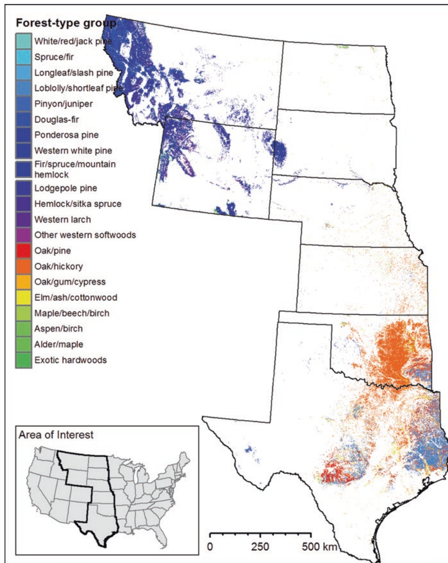
Fig. A12 Forest-type groups of the Great Plains (Source: Ruefenacht et al. 2008)
