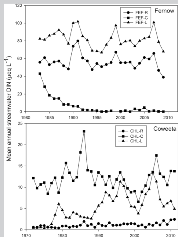
Box Fig. 4.1 Mean annual dissolved inorganic N (DIN) concentration in streams draining the six watersheds at the Fernow Experimental Forest (top panel) and Coweeta Hydrologic Laboratory (bottom panel). For DIN, 1 \mu\text{eq L}^{-1} is 1 \mu\text{mol L}^{-1} . (Source Adams 2014, reprinted with permission)
