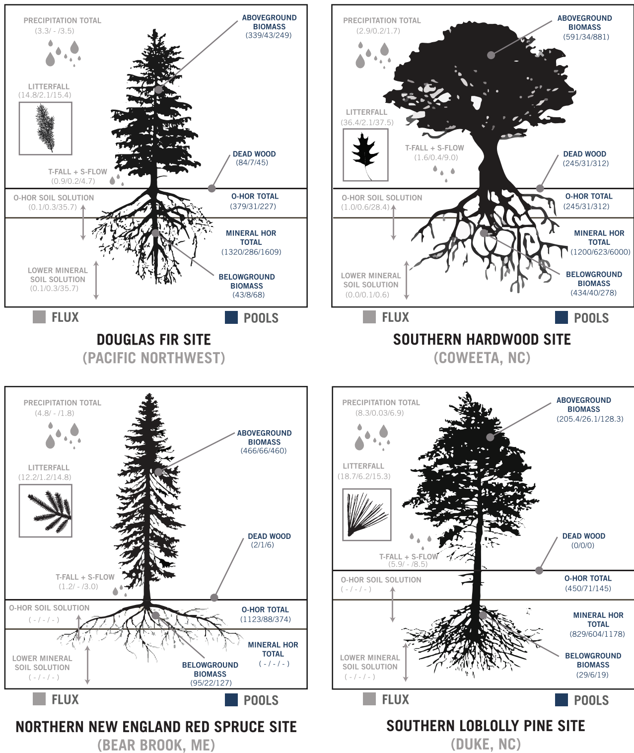
Fig. 4.1 Element pools and cycling of nitrogen (N), phosphorus (P), and calcium (Ca) in representative forest ecosystems in the United States. Values are given as N/P/Ca and are expressed as \text{kg ha}^{-1} for flux and \text{kg ha}^{-1} for pools (source: Johnson and Lindberg 1992)
