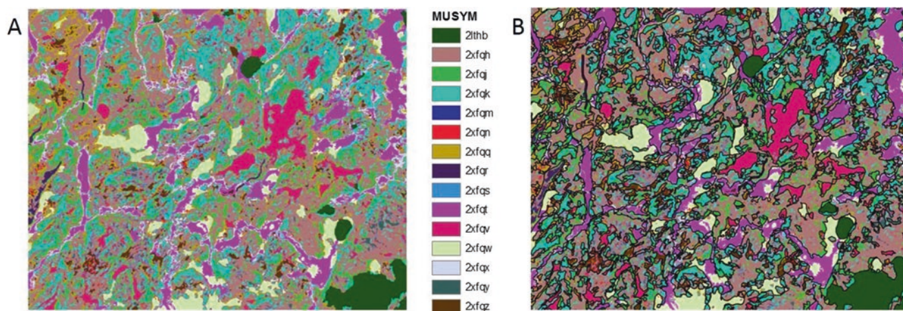
Fig. 9.1 Soil Survey Geographic (SSURGO) soil maps from the Boundary Waters Canoe Area Wilderness, Superior National Forest (MN613; St. Louis County, Minnesota, Crane Lake Part): (a) Component-level USDA NRCS SSURGO raster (10 m) soil survey
