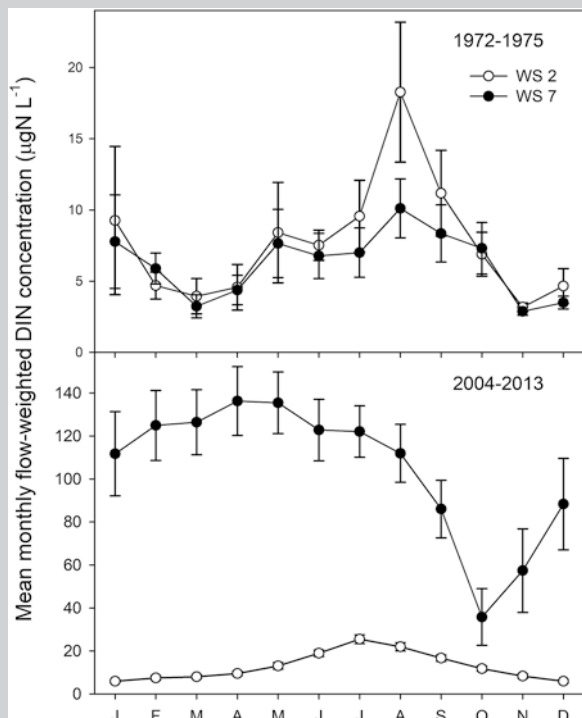
Box Fig. 4.2 Average ( \pm SE) flow-weighted monthly dissolve inorganic nitrogen (DIN) concentrations for WS2 and WS7 before clearcutting (1972-1975, top panel) and for the most recent 10 years (2004-2013, bottom panel). In the bottom panel most error bars for WS2 are smaller than the symbols
