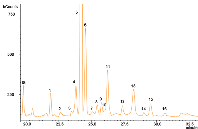
Fig. 1. Representative GC–MS chromatogram of TMS-derivatized phytosterols from a black walnut. The peak numbers in the chromatograms refer to the following components: 1 = campesterol, 2 = stigmasterol, 3 = \Delta^{5,23} -stigmastadienol, 4 = clerosterol, 5 = \beta -sitosterol, 6 = stigmastanol and \Delta^5 -avenasterol, 7 = unidentified, 8 = \Delta^{5,24(25)} -stigmastadienol, 9 = unidentified, 10 = cycloeucalenol, 11 = cycloartenol, 12 = 28-methylobtusifolol; 13 = 24-methylenecycloartenol; 14 = unidentified, 15 = citrostadienol, 16 = unidentified, IS = \alpha -cholestanol (internal standard).
