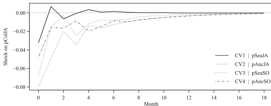
Fig. 6. Generalized impulse responses from the error correction model of five prices for Japan and South Korea for a one standard error shock on the price variable of pColJA over 18 months. See Fig. 5 for the definition of co-integrating vectors. Note that pColJA denotes the export price between Col and JA. See Fig. 1 for other definitions.
