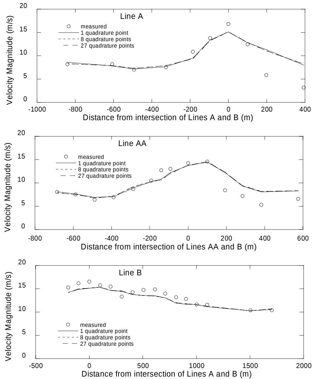
Figure 13. Comparison of simulated vs. measured wind velocities based on the number of quadrature points used in the numerical integration for Askervein Hill. Distances are from reference lines identified in Figure 9.
