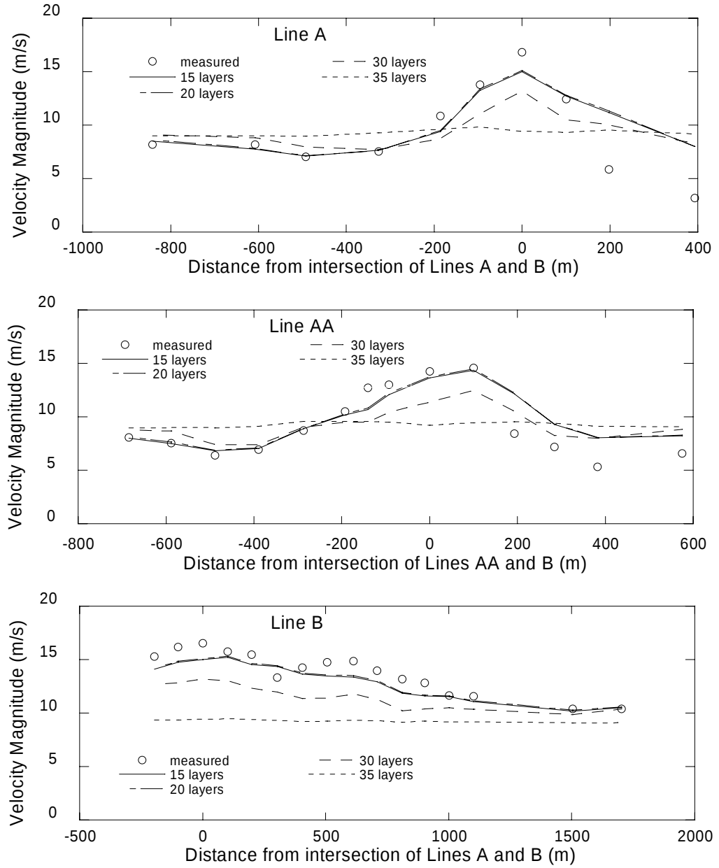
Figure 15. Comparison of simulated vs. measured wind velocities based on meshes with different numbers of vertical layers of cells for Askervein Hill. Distances are in relation to reference lines identified in Figure 9.
