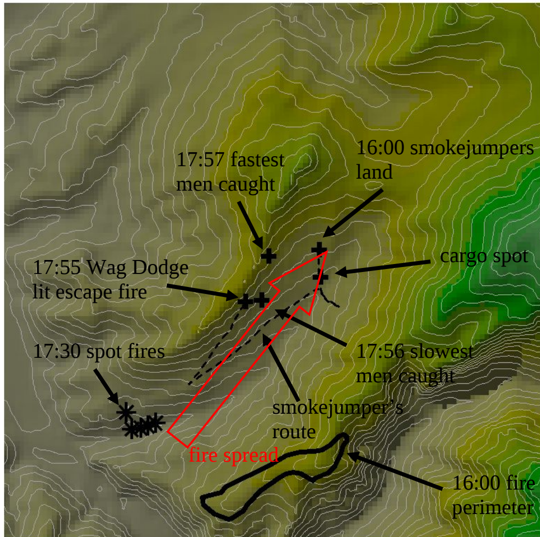
Figure 29. Elevation contour plot of the Mann Gulch Fire area. Contour spacing is 100 vertical feet. North is toward the top of the image. Locations identified are from Rothermel (1993).
