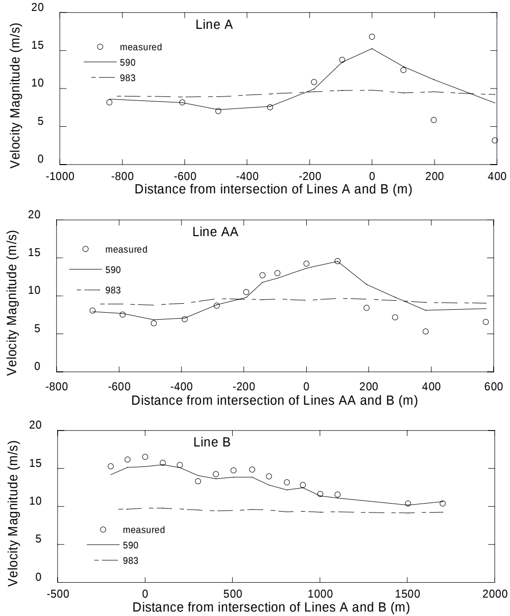
Figure 16. Comparison of simulated vs. measured wind velocities based on meshes with different aspect ratio (equation ( 31 )) for Askervein Hill. The case with an aspect ratio of 590 used the same input parameters as the 983 aspect ratio case, except that the horizontal cell size used was 23.4375 meters instead of 40 meters which gave the lower aspect ratio. The vertical cell sizes were approximately equal. Distances are in relation to reference lines identified in Figure 9.
