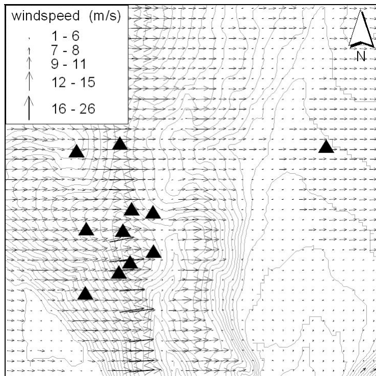
Figure 7. Wind vector plot of simulated flow using the fine mesh in the Waterworks Hill area. The vectors are spaced on an 80 meter grid.
