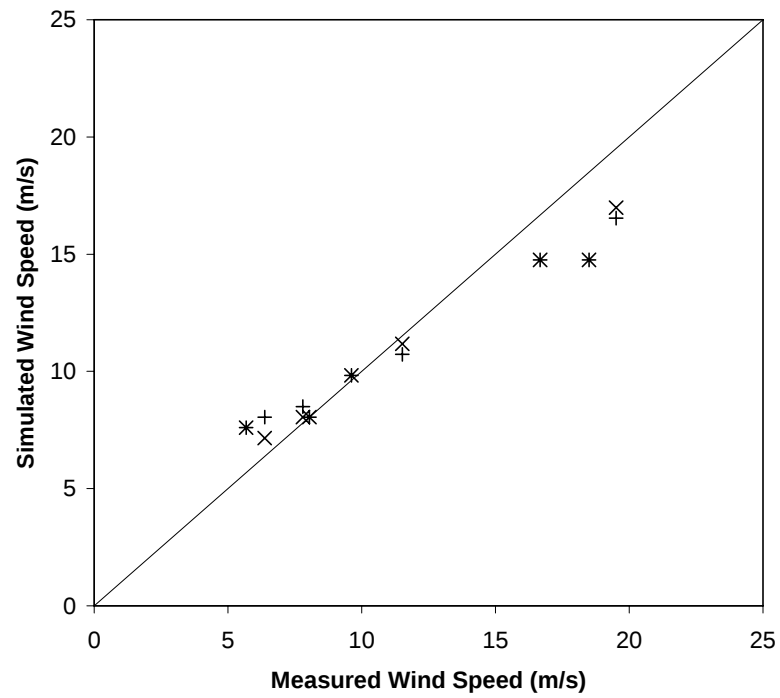
Figure 8. Comparison of simulated and observed wind speeds over Waterworks Hill. The x's represent the fine grid and the + signs represent the coarse grid. The solid black line is the line of perfect agreement.
