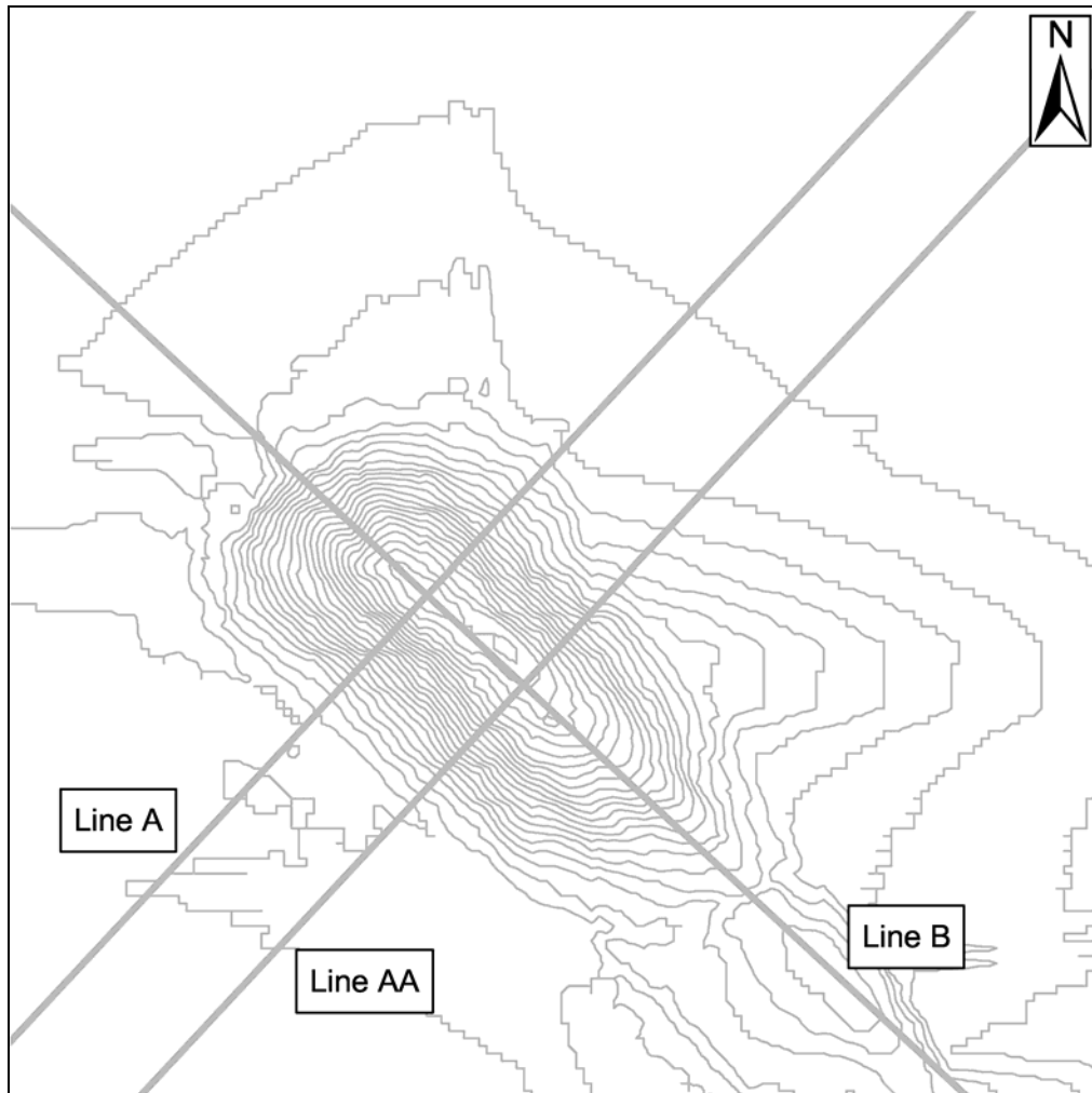
Figure 1. Contour map of Askervein Hill showing locations of Lines A, AA, and B. The contour interval is 5 meters.
