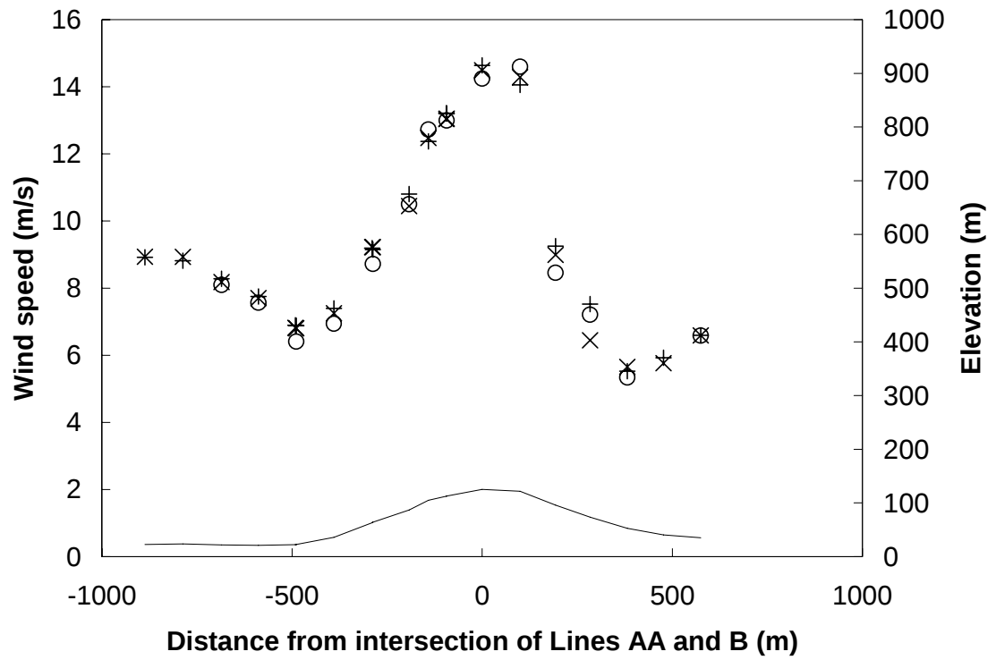
Figure 3. Wind speed along line AA (Figure 1). Circles represent measured values, x's are the fine grid and plus symbols are the coarse grid. The solid line shows the elevation of Askervein hill.
