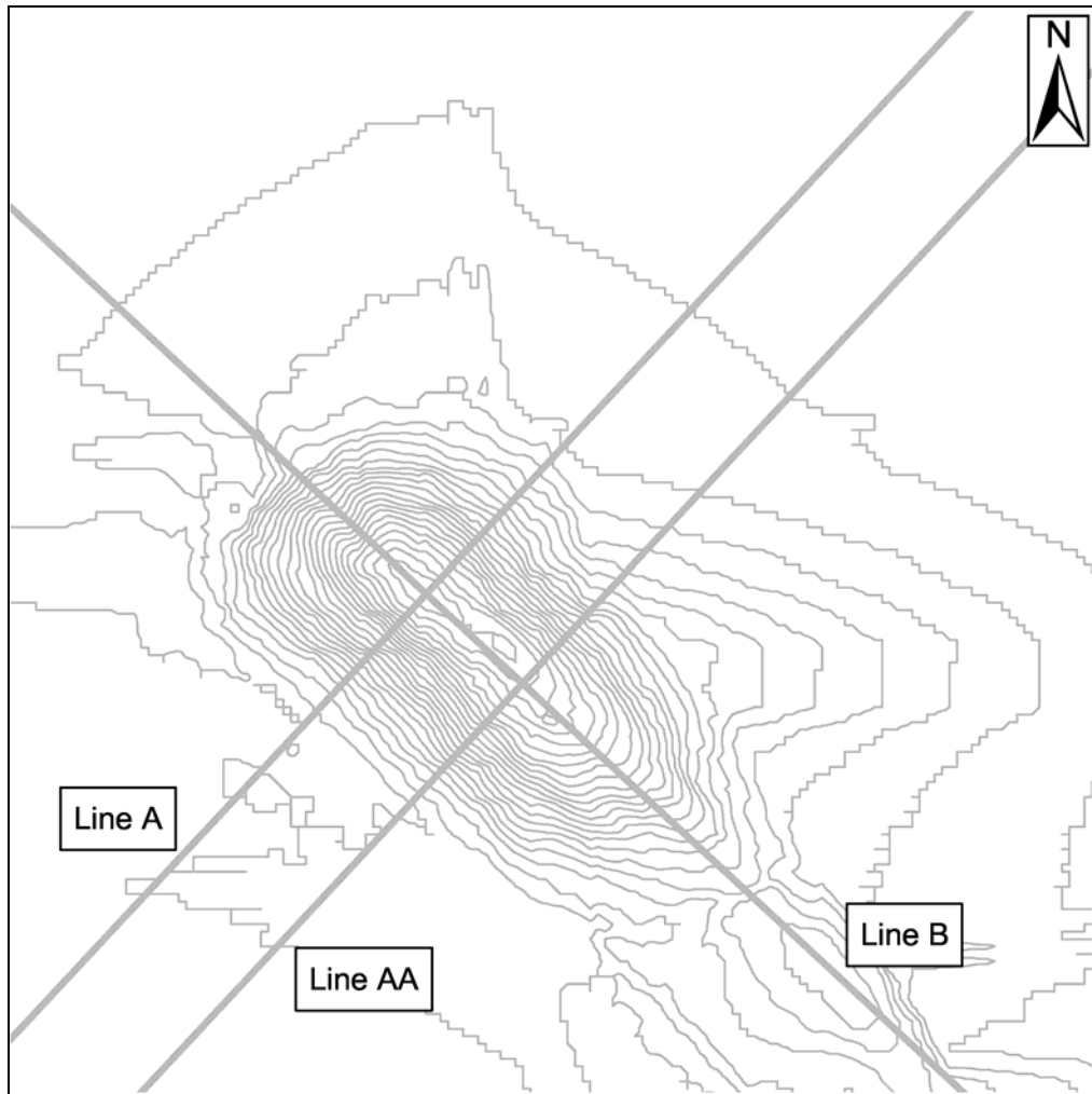
Figure 20. Contour map of Askervein Hill showing locations of Lines A, AA, and B. The contour interval is 5 meters.
