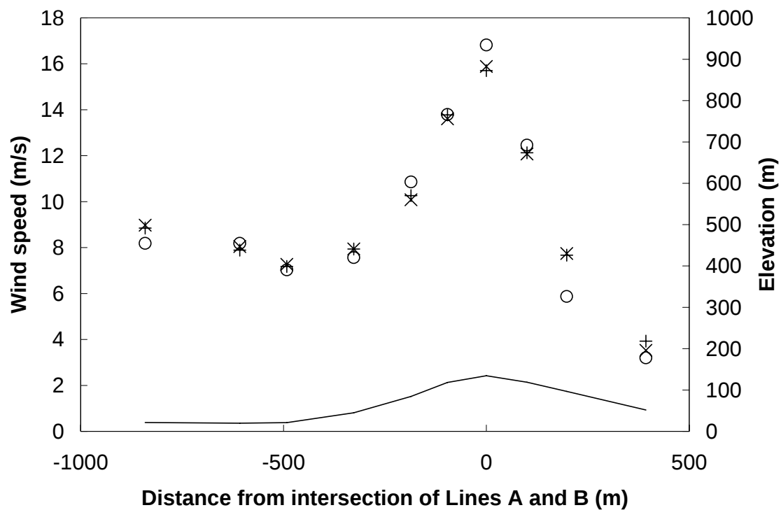
Figure 2. Wind speed along line A (Figure 1). Circles represent measured values, x's are the fine grid and plus symbols are the coarse grid. The solid line shows the elevation of Askervein hill.
