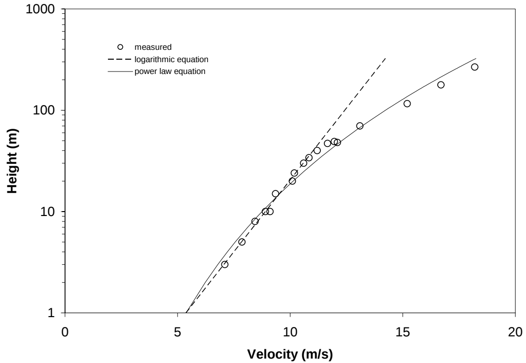
Figure 10. Comparison of wind velocities with a logarithmic and power law equation at the upstream reference site at Askervein Hill on semi-log axes.
