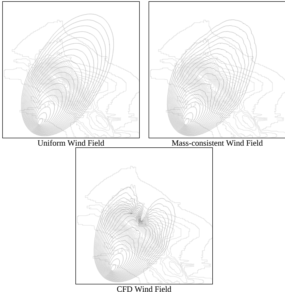
Figure 22. Comparison of three fire spread simulations for the Askervein Hill area using different wind fields. Dark lines denote the fire progression spaced 10 minutes apart, light lines are the 5 meter elevation contour lines. North is toward the top of the image.
