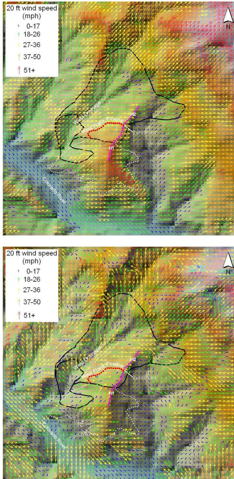
Figure 26. Wind simulations for the South Canyon Fire. The general winds are from 240 degrees. The top image is a mass-consistent model run and the bottom image is a CFD run. The two black outlines are the observed fire perimeters at 1607 and 1623.
