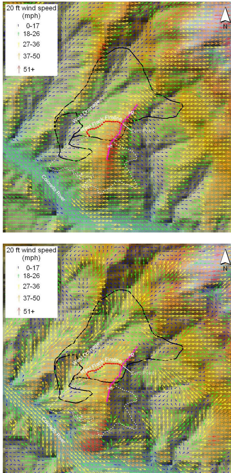
Figure 27. Wind simulations for the South Canyon Fire. The general winds are from 270 degrees. The top image is a mass-consistent model run and the bottom image is a CFD run. The two black outlines are the observed fire perimeters at 1607 and 1623.
