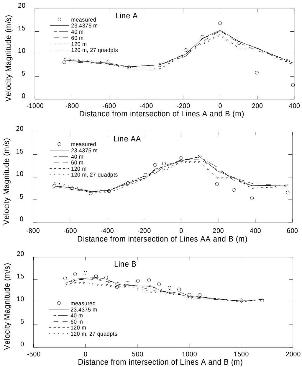
Figure 14. Comparison of simulated vs. measured wind velocities based on meshes with different horizontal cell resolution for Askervein Hill. Distances are in relation to reference lines identified in Figure 9.
