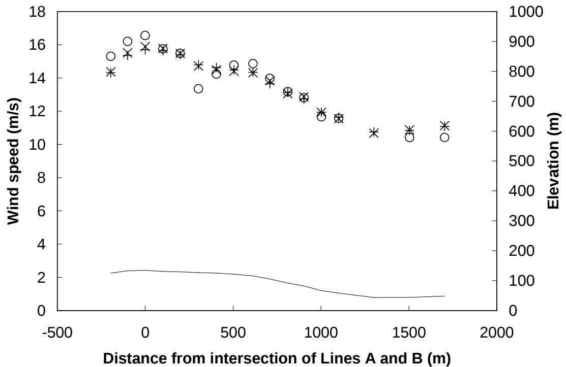
Figure 4. Wind speed along line B (Figure 1). Circles represent measured values, x's are the fine grid and plus symbols are the coarse grid. The solid line shows the elevation of Askervein hill.
