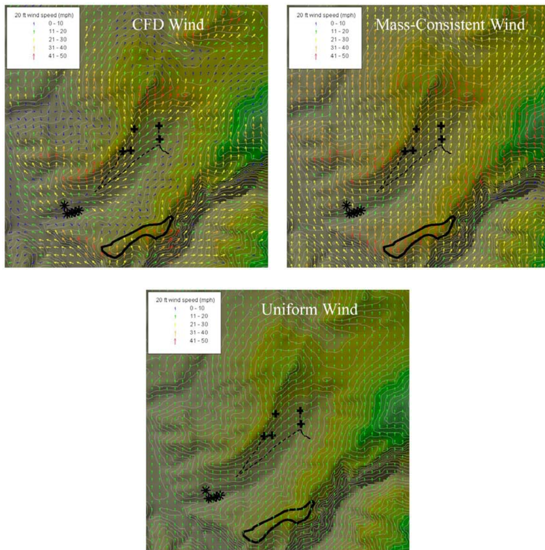
Figure 31. Wind simulations and uniform wind for the Mann Gulch Fire. Wind direction is from 180°. North is toward the top of the images.
