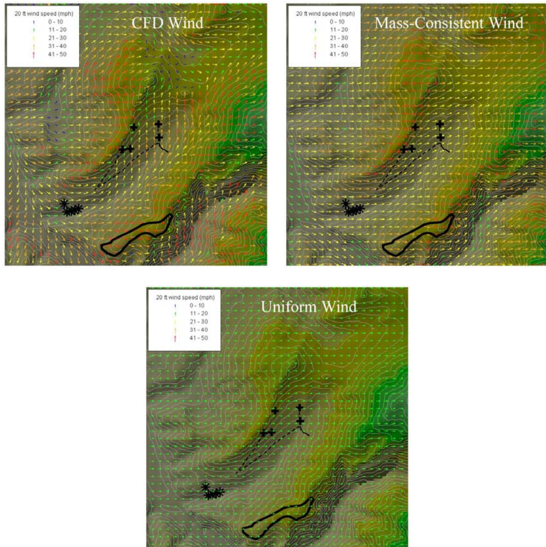
Figure 32. Wind simulations and uniform wind for the Mann Gulch Fire. Wind direction is from 270°. North is toward the top of the images.
