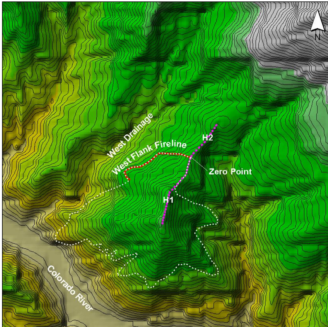
Figure 23. South Canyon Fire area map. The white dotted line indicates the fire perimeter before the blowup, the red dotted line is the West flank fireline, and the purple dotted line indicates the main ridge fireline. Helispots 1 and 2 are indicated by H1 and H2. The “Zero Point” is the point where the West flank fireline meets the ridgeline, as designated in Butler et al. (1998). The contour lines and coloring show the terrain relief.
