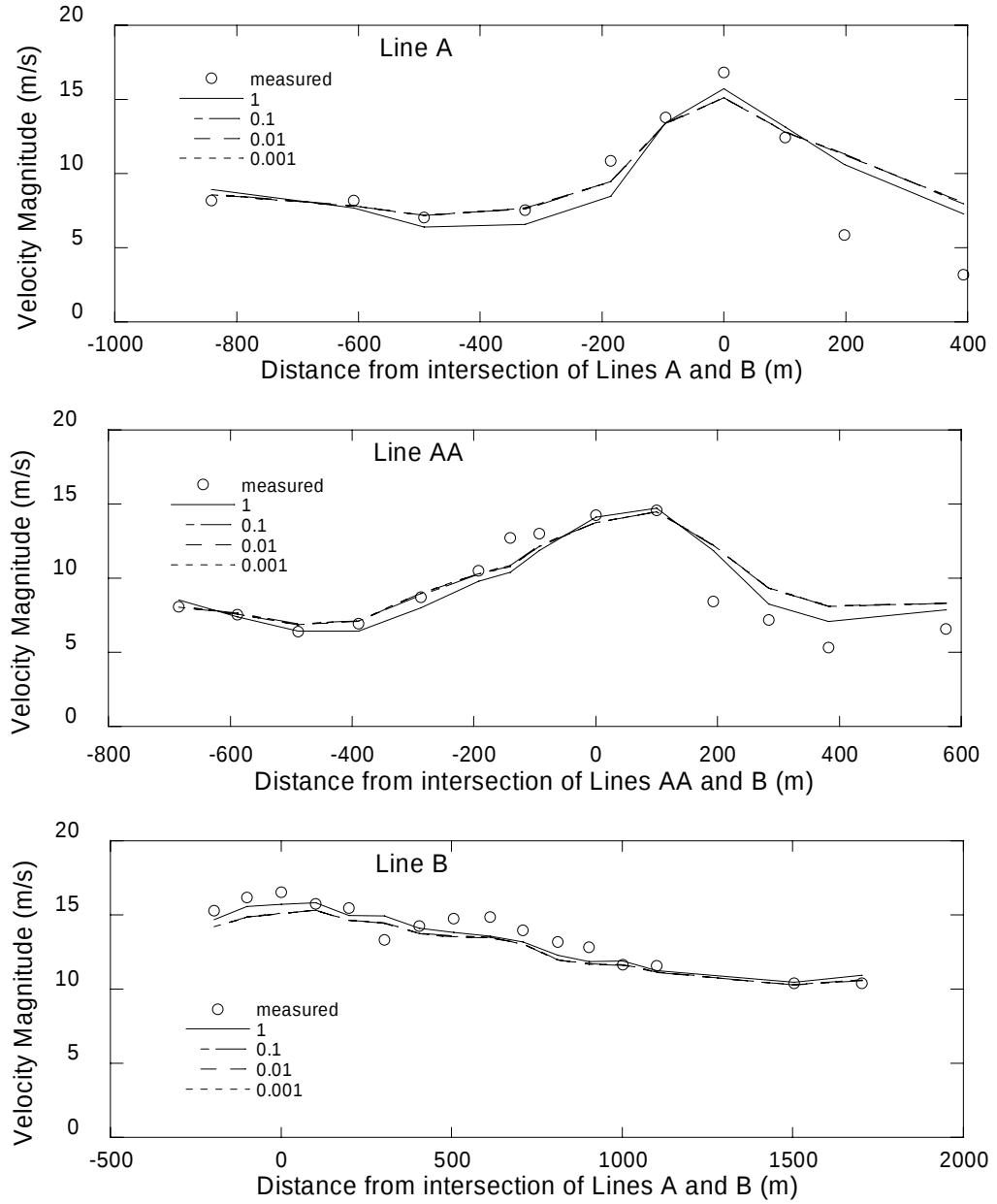
Figure 12. Comparison of simulated vs. measured wind velocities with different stop\_tol values (equation ( 30 )) for Askervein Hill. Distances are in relation to reference lines identified in Figure 9.
