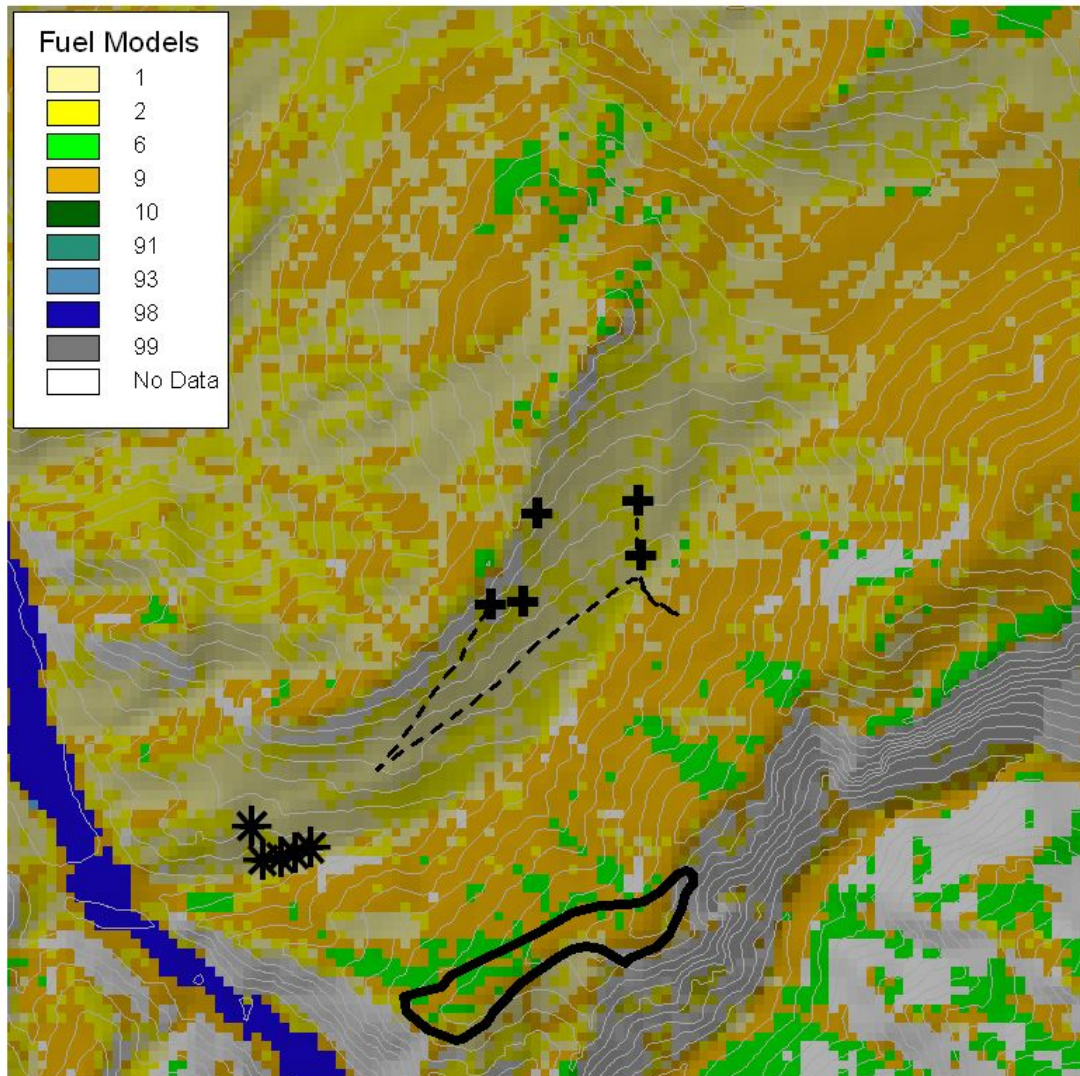
Figure 30. Fuels map used in simulations of the Mann Gulch Fire area. Contour line spacing is 100 vertical feet. North is toward the top of the image.
