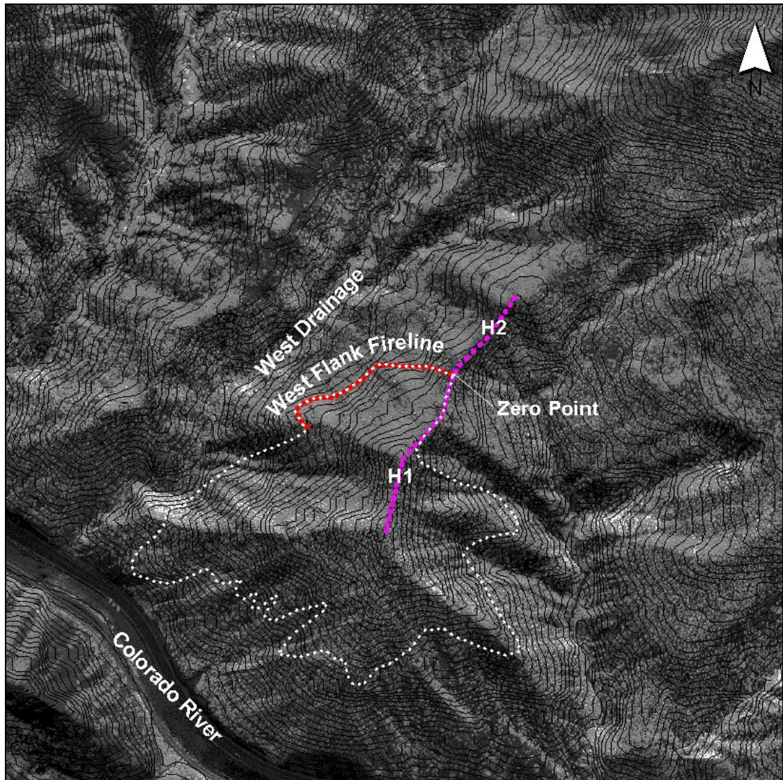
Figure 24. Original DOQ at 1 meter resolution for the South Canyon Fire. Lines and notation shown are described in Figure 23.
