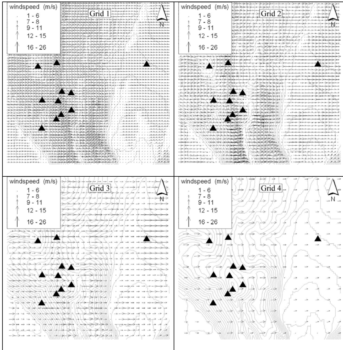
Figure 18. Wind vectors on Waterworks Hill for different grids. The plots are zoomed in to the hill area. Measurement stations are shown as black triangles.
