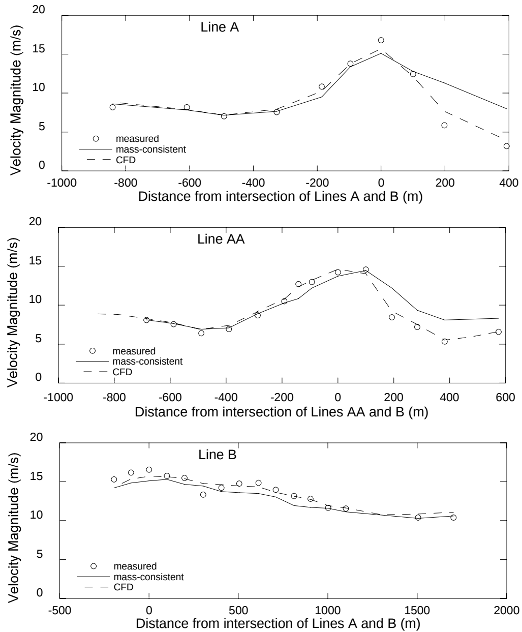
Figure 21. Simulated wind speeds from the mass-consistent and CFD models compared with measured wind speeds for Lines A, AA, and B from Figure 20 over Askervein Hill. The winds are for 10 meters above the ground.
