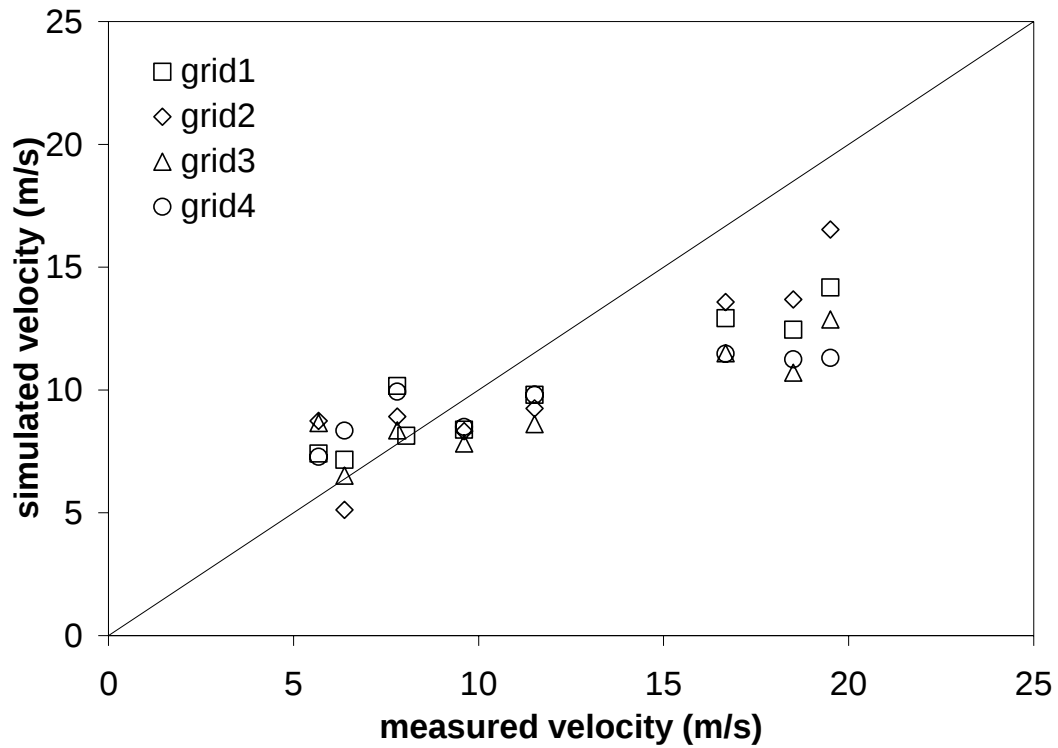
Figure 19. Waterworks Hill simulation results compared to measured values.
