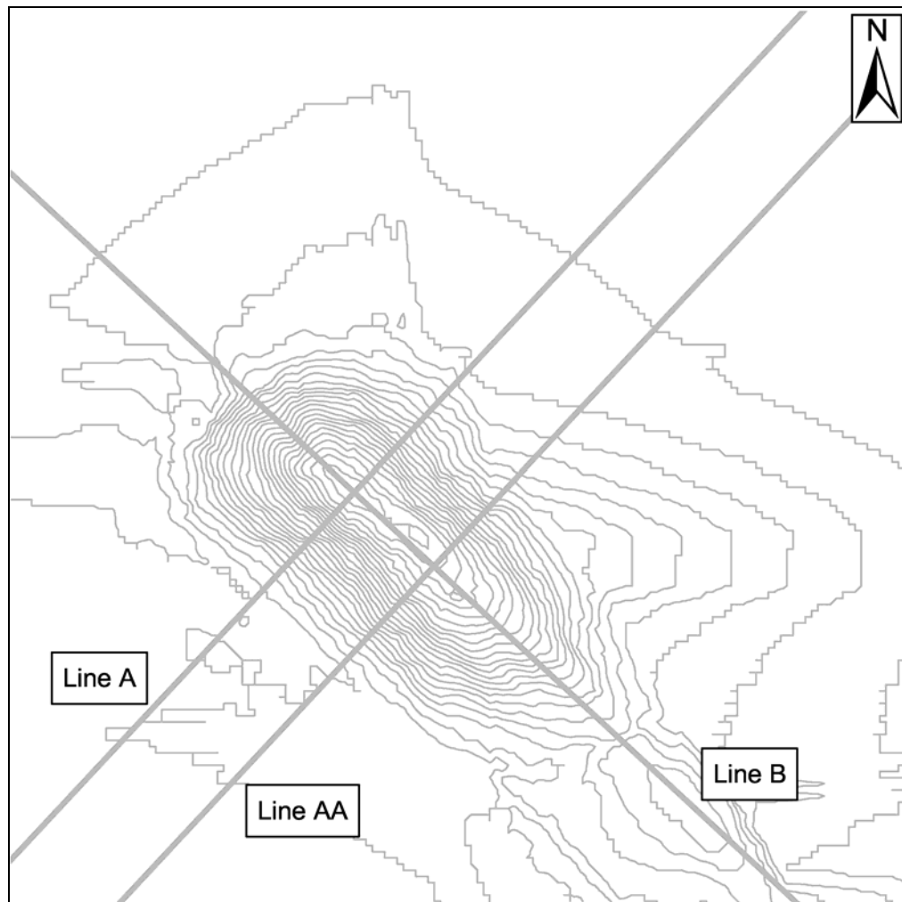
Figure 9. Contour map of Askervein Hill showing locations of Lines A, AA, and B. The contour interval is 5 meters.
