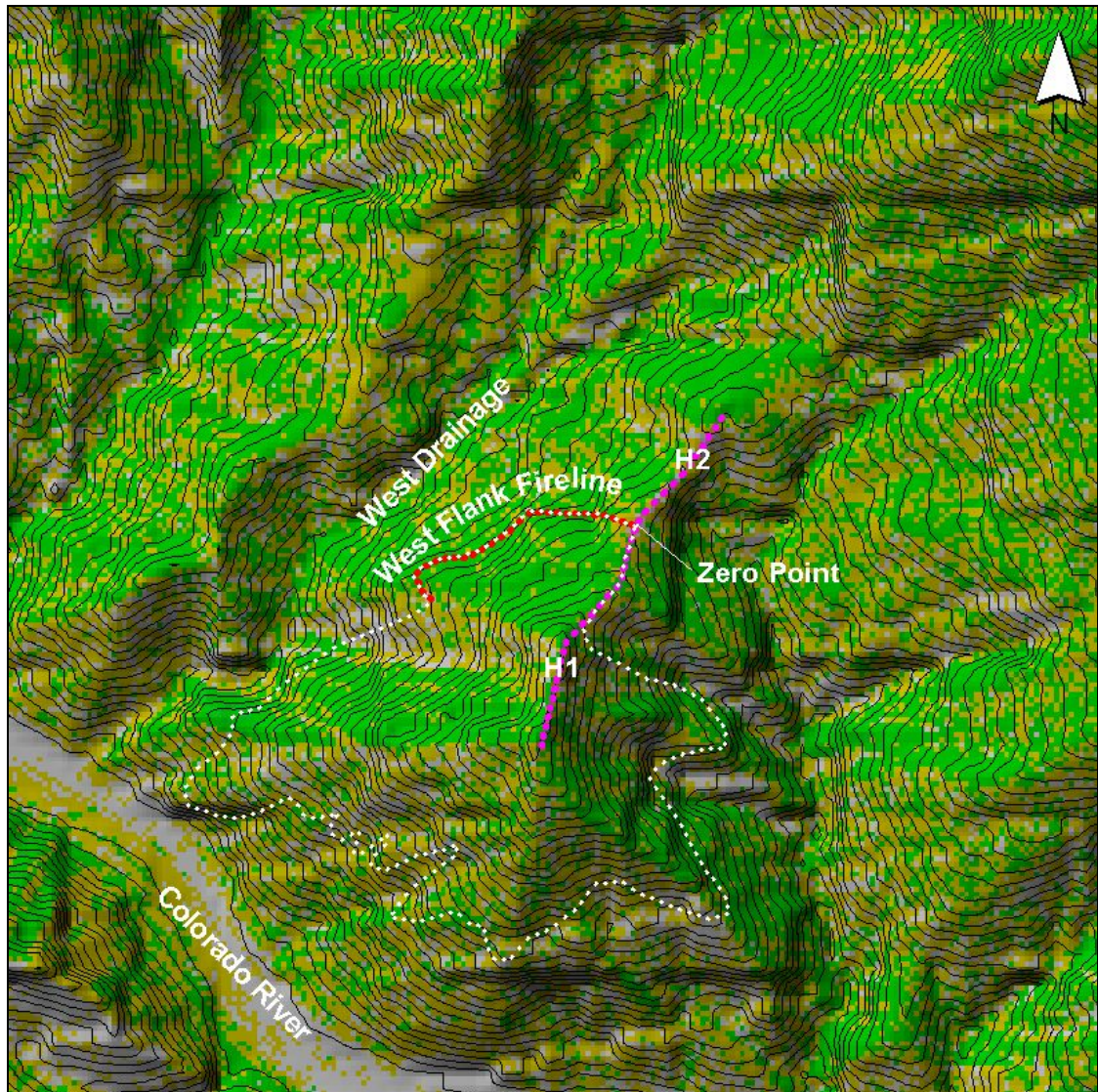
Figure 25. Fuel model map at 10 meter resolution for the South Canyon Fire vicinity. FM 10 - dark green; FM 4 - green; FM 2 - tan; FM 99 (barren-rock) - gray. Lines and notation shown are described in Figure 23.
