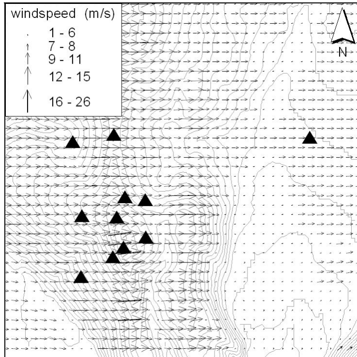
Figure 6. Wind vector plot of simulated flow using the coarse mesh in the Waterworks Hill area. The vectors are spaced on an 80 meter grid.
